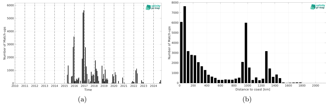
Figure 2: Number of match-ups between TSG (SAMOS) and SMAP SSS L2 v6 - 40 km (RSS) SSS as a function of time (a) and as function of the distance to coast (b) over the Roaring Forties and Furious Fifties Pi-MEP region and for the full satellite product period.
