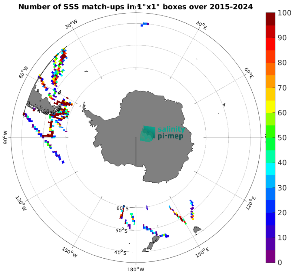
Figure 5: Number of SSS match-ups between TSG (SAMOS) SSS and the SMAP SSS L2 v6 - 40 km (RSS) SSS product for the Roaring Forties and Furious Fifties Pi-MEP region over 1^\circ \times 1^\circ boxes and for the full satellite product period.
