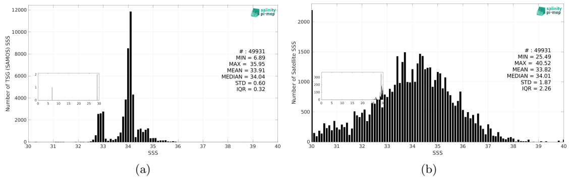
Figure 3: Histograms of SSS from TSG (SAMOS) (a) and SMAP SSS L2 v6 - 40 km (RSS) (b) considering all match-up pairs per bins of 0.1 over the Roaring Forties and Furious Fifties Pi-MEP region and for the full satellite product period.
