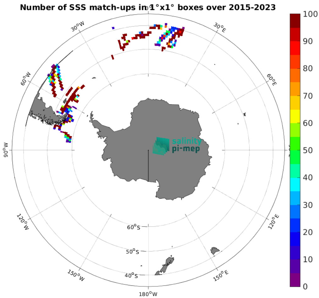
Figure 5: Number of SSS match-ups between TSG (Polarstern) SSS and the SMAP SSS L2 v6 - 40 km (RSS) SSS product for the Roaring Forties and Furious Fifties Pi-MEP region over 1^\circ \times 1^\circ boxes and for the full satellite product period.
