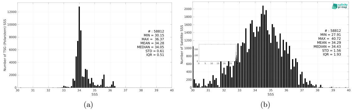
Figure 3: Histograms of SSS from TSG (Polarstern) (a) and SMAP SSS L2 v6 - 40 km (RSS) (b) considering all match-up pairs per bins of 0.1 over the Roaring Forties and Furious Fifties Pi-MEP region and for the full satellite product period.
