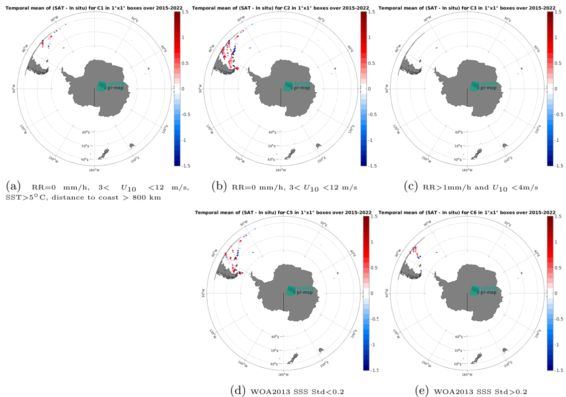
Figure 14: Temporal mean gridded over spatial boxes of size 1^\circ \times 1^\circ of \Delta SSS (SMAP SSS L2 v6 - 40 km (RSS) - TSG (CSIC-UTM)) for 5 different subdatasets corresponding to:RR=0 mm/h, 3 < U_{10} < 12 m/s, SST>5°C, distance to coast > 800 km (a), RR=0 mm/h, 3 < U_{10} < 12 m/s (b), RR>1mm/h and U_{10} < 4 m/s (c), WOA2013 SSS Std<0.2 (d), WOA2013 SSS Std>0.2 (e).
