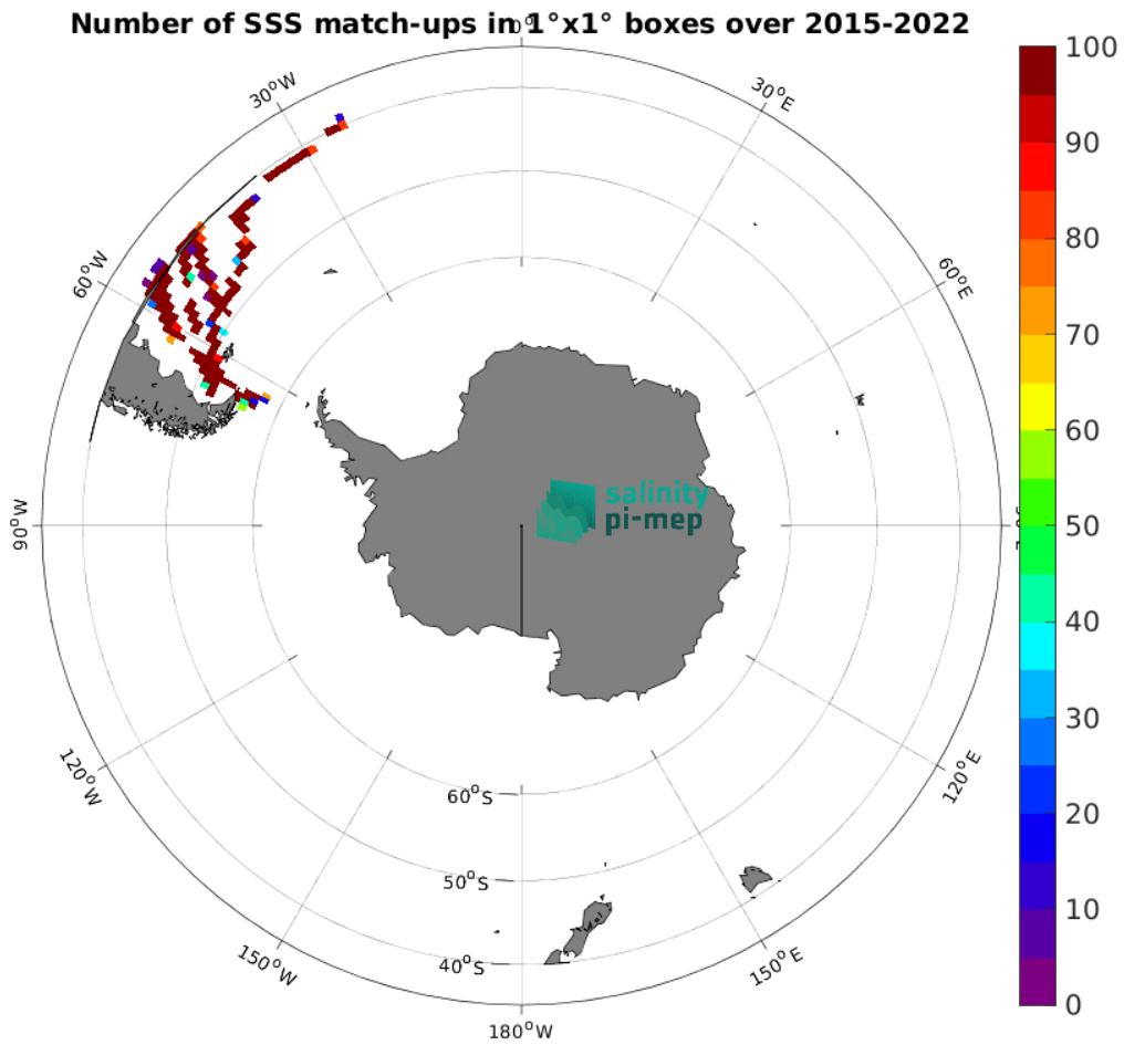
Figure 5: Number of SSS match-ups between TSG (CSIC-UTM) SSS and the SMAP SSS L2 v6 - 40 km (RSS) SSS product for the Roaring Forties and Furious Fifties Pi-MEP region over 1^\circ \times 1^\circ boxes and for the full satellite product period.
