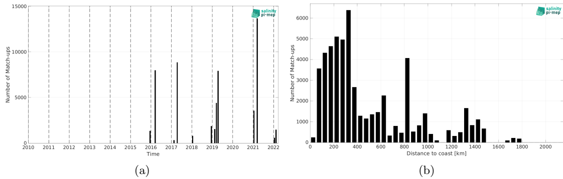
Figure 2: Number of match-ups between TSG (CSIC-UTM) and SMAP SSS L2 v6 - 40 km (RSS) SSS as a function of time (a) and as function of the distance to coast (b) over the Roaring Forties and Furious Fifties Pi-MEP region and for the full satellite product period.
