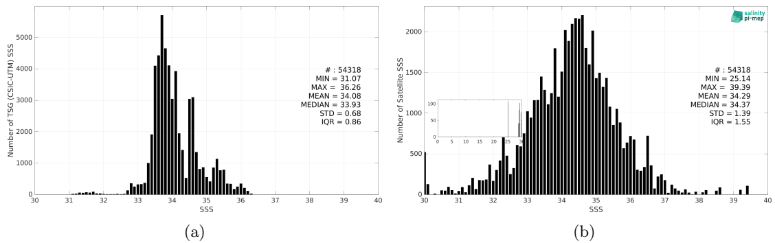
Figure 3: Histograms of SSS from TSG (CSIC-UTM) (a) and SMAP SSS L2 v6 - 40 km (RSS) (b) considering all match-up pairs per bins of 0.1 over the Roaring Forties and Furious Fifties Pi-MEP region and for the full satellite product period.
