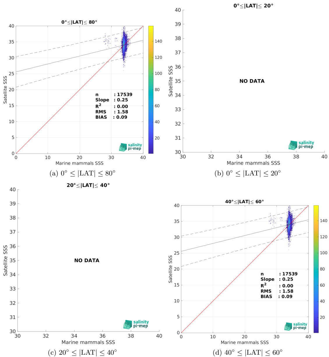
Figure 10: Contour maps of the concentration of SMAP SSS L2 v6 - 40 km (RSS) SSS (y-axis) versus Marine mammals SSS (x-axis) at match-up pairs for different latitude bands. For each plot, the red line shows x=y . The black thin and dashed lines indicate a linear fit through the data cloud and the \pm 95\% confidence levels, respectively. The number match-up pairs n , the slope and R^2 coefficient of the linear fit, the root mean square (RMS) and the mean bias between satellite and in situ data are indicated for each latitude band in each plots.
