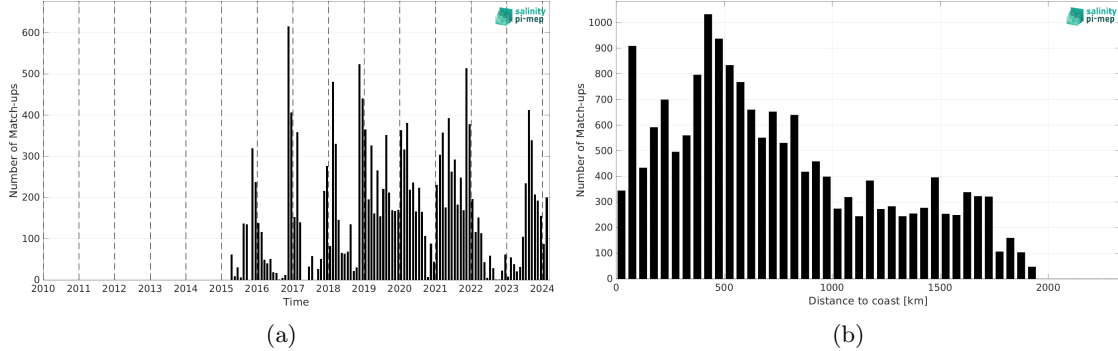
Figure 2: Number of match-ups between Marine mammals and SMAP SSS L2 v6 - 40 km (RSS) SSS as a function of time (a) and as function of the distance to coast (b) over the Roaring Forties and Furious Fifties Pi-MEP region and for the full satellite product period.
