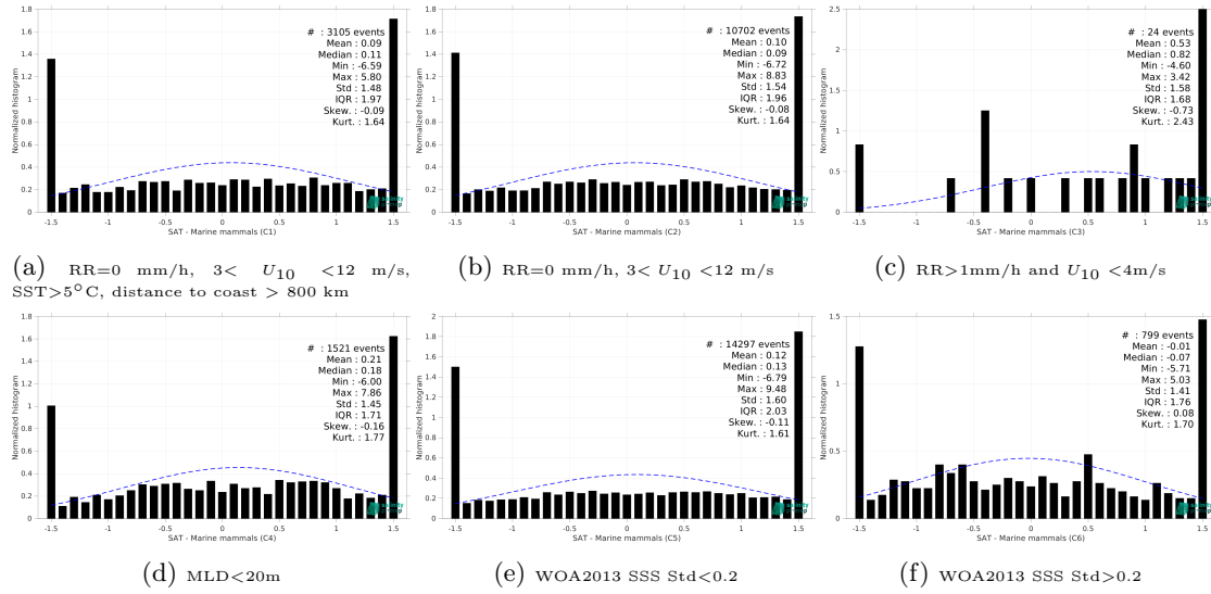
Figure 15: Normalized histogram of \Delta\text{SSS} (SMAP SSS L2 v6 - 40 km (RSS) - Marine mammals) for 6 different subdatasets corresponding to: RR=0 mm/h, 3 < U_{10} < 12 m/s, SST>5°C, distance to coast > 800 km (a), RR=0 mm/h, 3 < U_{10} < 12 m/s (b), RR>1mm/h and U_{10} < 4 m/s (c), MLD<20m (d), WOA2013 SSS Std<0.2 (e), WOA2013 SSS Std>0.2 (f).
