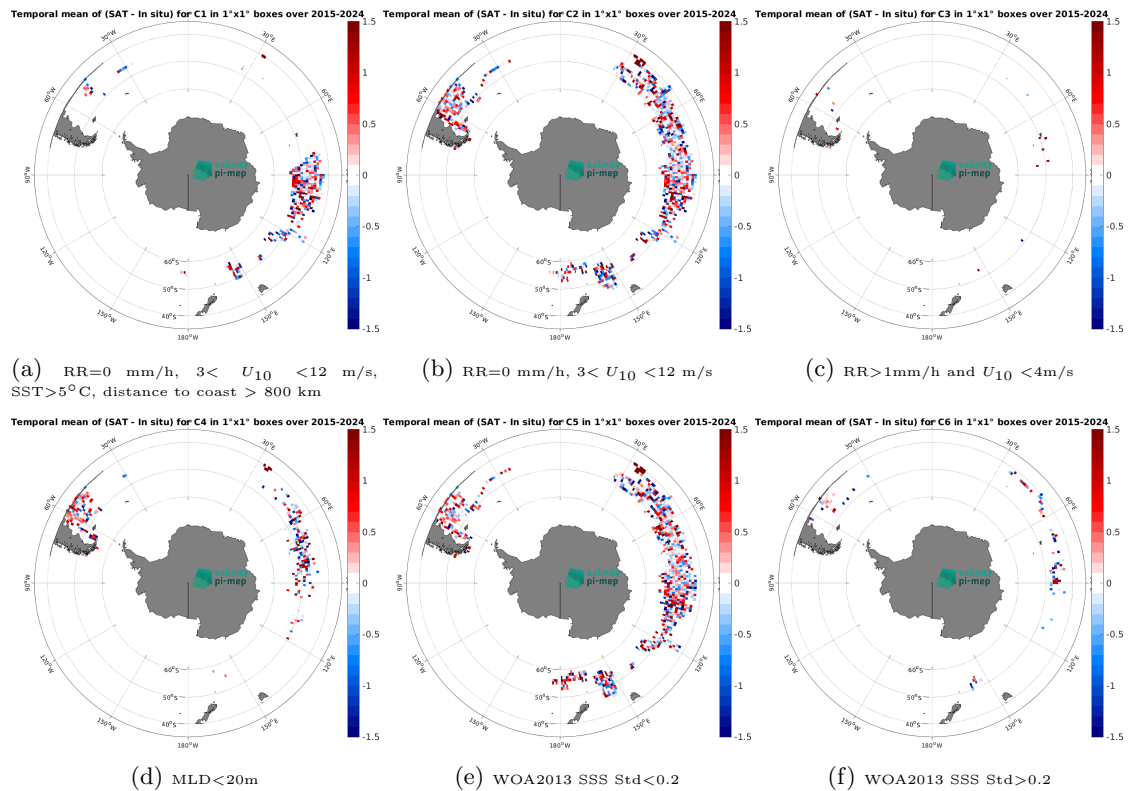
Figure 14: Temporal mean gridded over spatial boxes of size 1^\circ \times 1^\circ of \Delta SSS (SMAP SSS L2 v6 - 40 km (RSS) - Marine mammals) for 6 different subdatasets corresponding to:RR=0 mm/h, 3 < U_{10} < 12 m/s, SST>5°C, distance to coast > 800 km (a), RR=0 mm/h, 3 < U_{10} < 12 m/s (b), RR>1mm/h and U_{10} < 4 m/s (c),MLD<20m (d),WOA2013 SSS Std<0.2 (e),WOA2013 SSS Std>0.2 (f).
