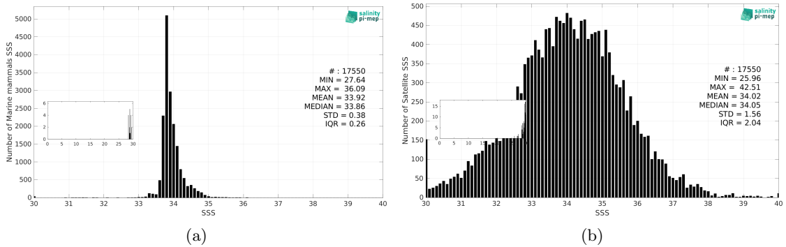
Figure 3: Histograms of SSS from Marine mammals (a) and SMAP SSS L2 v6 - 40 km (RSS) (b) considering all match-up pairs per bins of 0.1 over the Roaring Forties and Furious Fifties Pi-MEP region and for the full satellite product period.
