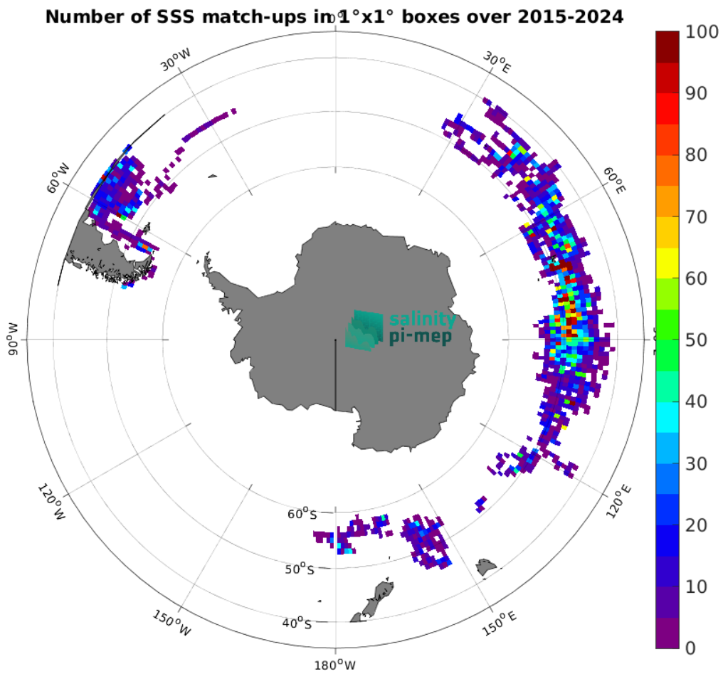
Figure 5: Number of SSS match-ups between Marine mammals SSS and the SMAP SSS L2 v6 - 40 km (RSS) SSS product for the Roaring Forties and Furious Fifties Pi-MEP region over 1^\circ \times 1^\circ boxes and for the full satellite product period.
