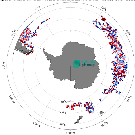
(e) MEAN( \Delta SSS) (Satellite - Marine mammals) 17
