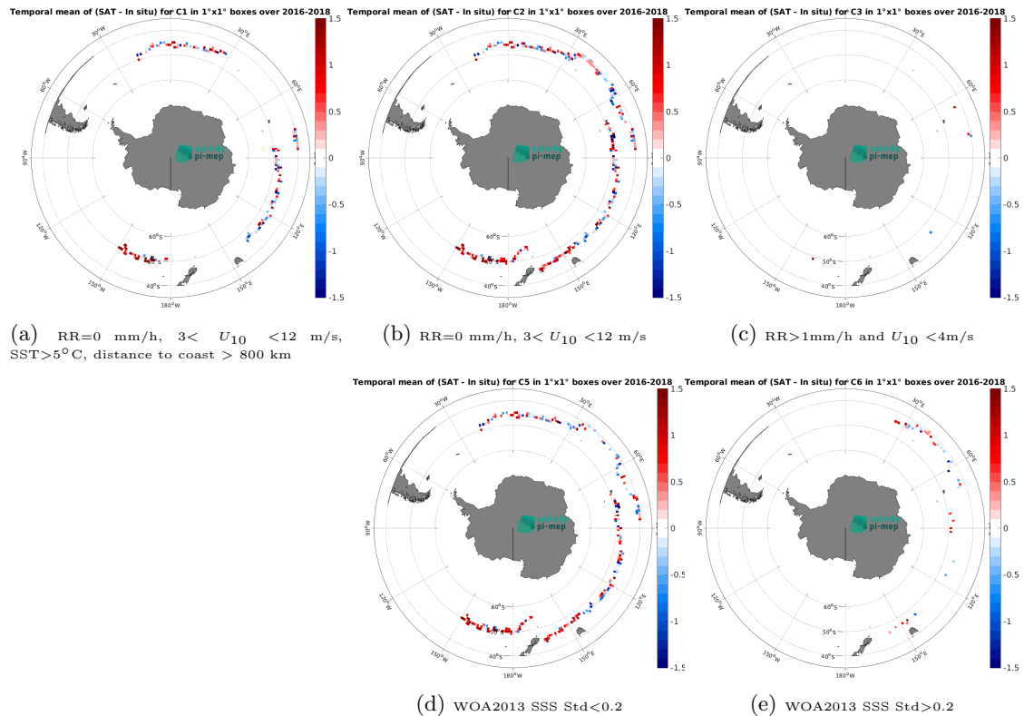
Figure 13: Temporal mean gridded over spatial boxes of size 1^\circ \times 1^\circ of \Delta SSS (SMAP SSS L2 v6 - 40 km (RSS) - Surface drifters) for 5 different subdatasets corresponding to:RR=0 mm/h, 3 < U_{10} < 12 m/s, SST >5^\circ\text{C} , distance to coast > 800 km (a), RR=0 mm/h, 3 < U_{10} < 12 m/s (b), RR >1 mm/h and U_{10} < 4 m/s (c), WOA2013 SSS Std <0.2 (d), WOA2013 SSS Std >0.2 (e).
