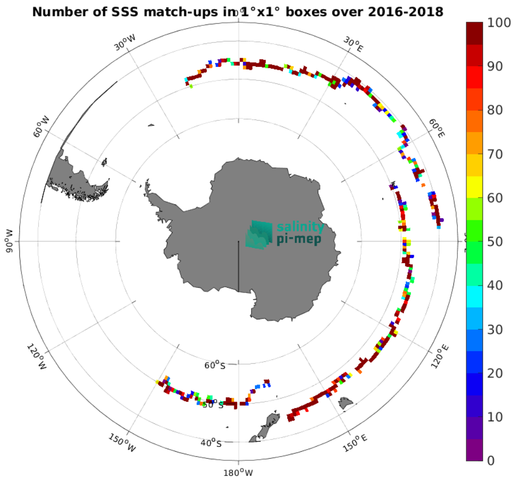
Figure 4: Number of SSS match-ups between Surface drifters SSS and the SMAP SSS L2 v6 - 40 km (RSS) SSS product for the Roaring Forties and Furious Fifties Pi-MEP region over 1^\circ \times 1^\circ boxes and for the full satellite product period.
