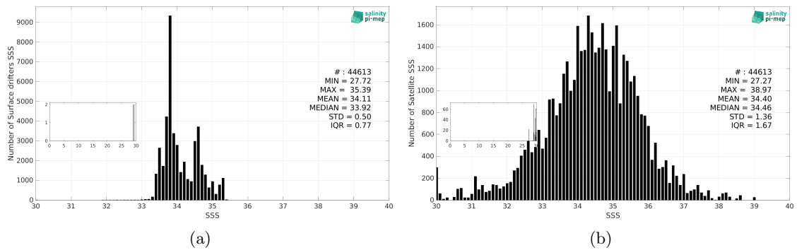
Figure 3: Histograms of SSS from Surface drifters (a) and SMAP SSS L2 v6 - 40 km (RSS) (b) considering all match-up pairs per bins of 0.1 over the Roaring Forties and Furious Fifties Pi-MEP region and for the full satellite product period.
