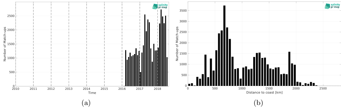
Figure 2: Number of match-ups between Surface drifters and SMAP SSS L2 v6 - 40 km (RSS) SSS as a function of time (a) and as function of the distance to coast (b) over the Roaring Forties and Furious Fifties Pi-MEP region and for the full satellite product period.
