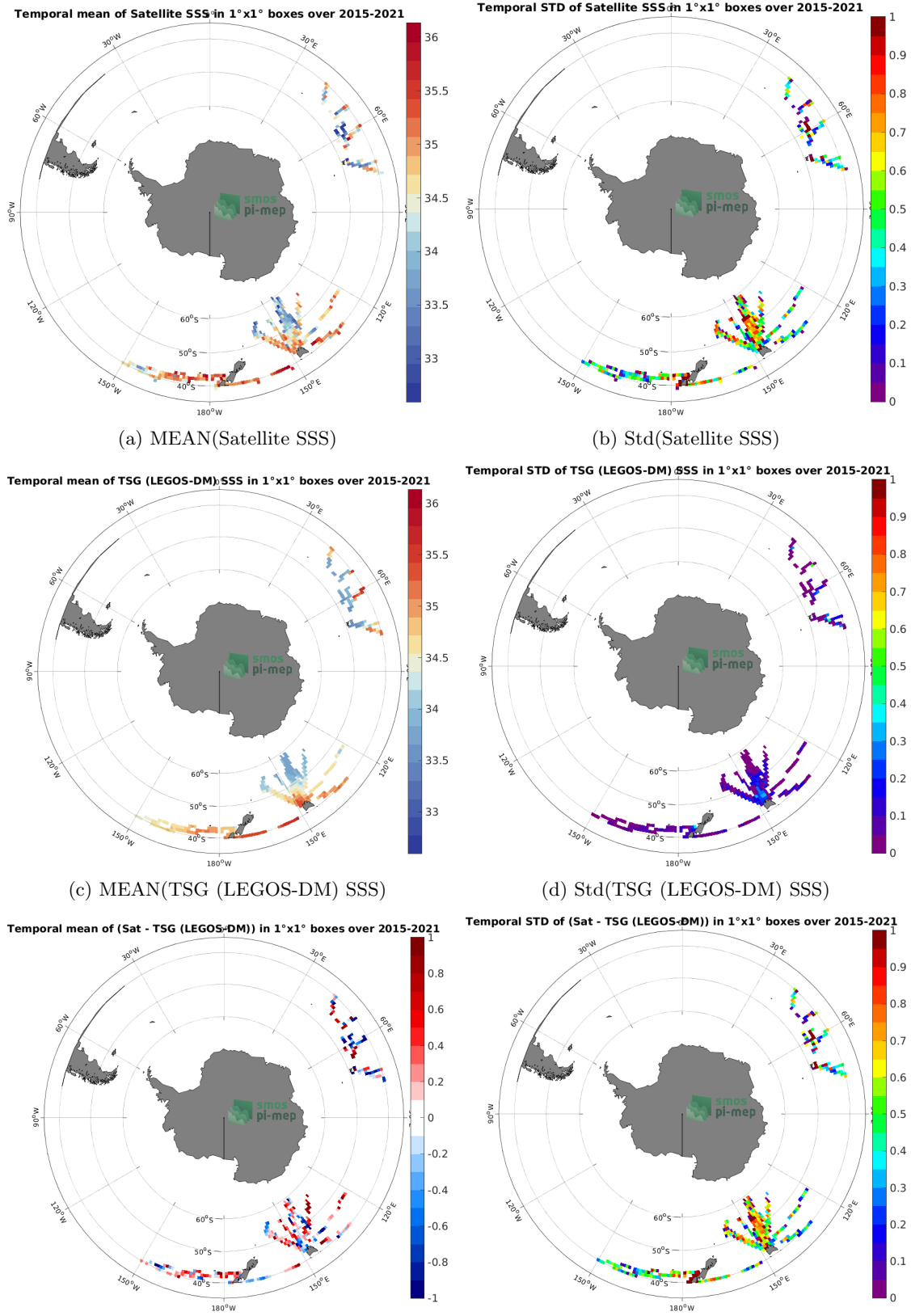
Figure 6: Temporal mean (left) and Std (right) of SSS from SMAP SSS L2 v5 (RSS) (top), TSG (LEGOS-DM) (middle), and of \Delta SSS (Satellite - TSG (LEGOS-DM)). Only match-up pairs are used to generate these maps.
