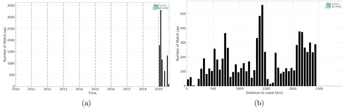
Figure 1: Number of match-ups between Saildrone and SMAP SSS L2 v5 (RSS) SSS as a function of time (a) and as function of the distance to coast (b) over the Roaring Forties and Furious Fifties Pi-MEP region and for the full satellite product period.
