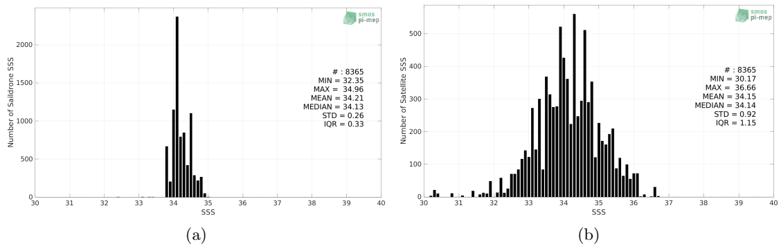
Figure 2: Histograms of SSS from Saildrone (a) and SMAP SSS L2 v5 (RSS) (b) considering all match-up pairs per bins of 0.1 over the Roaring Forties and Furious Fifties Pi-MEP region and for the full satellite product period.
