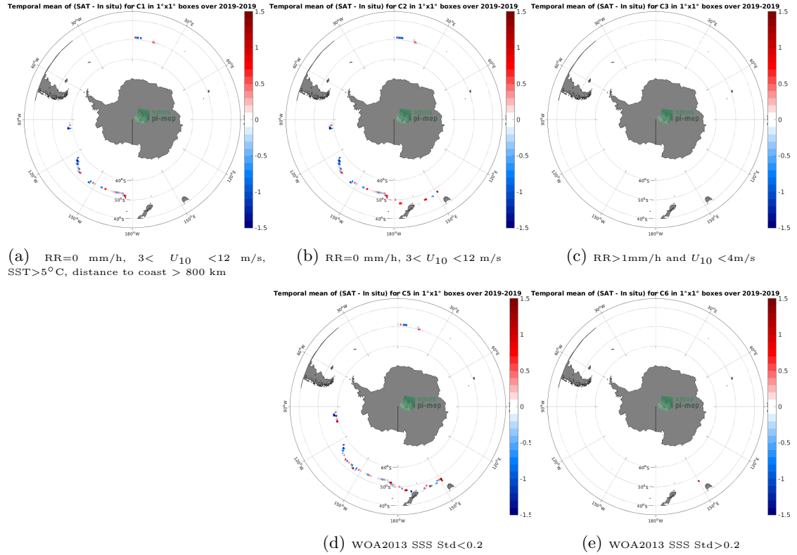
Figure 12: Temporal mean gridded over spatial boxes of size 1^{\circ}\times 1^{\circ} of \Delta\text{SSS} (SMAP SSS L2 v5 (RSS) - Saildrone) for 5 different subdatasets corresponding to:RR=0 mm/h, 3 < U_{10} < 12 m/s, SST >5^{\circ}\text{C} , distance to coast > 800 km (a), RR=0 mm/h, 3 < U_{10} < 12 m/s (b), RR >1 mm/h and U_{10} < 4 m/s (c), WOA2013 SSS Std <0.2 (d), WOA2013 SSS Std >0.2 (e).
