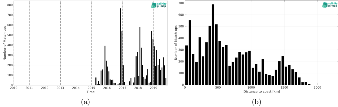
Figure 1: Number of match-ups between Marine mammals and SMAP SSS L2 v5 (RSS) SSS as a function of time (a) and as function of the distance to coast (b) over the Roaring Forties and Furious Fifties Pi-MEP region and for the full satellite product period.
