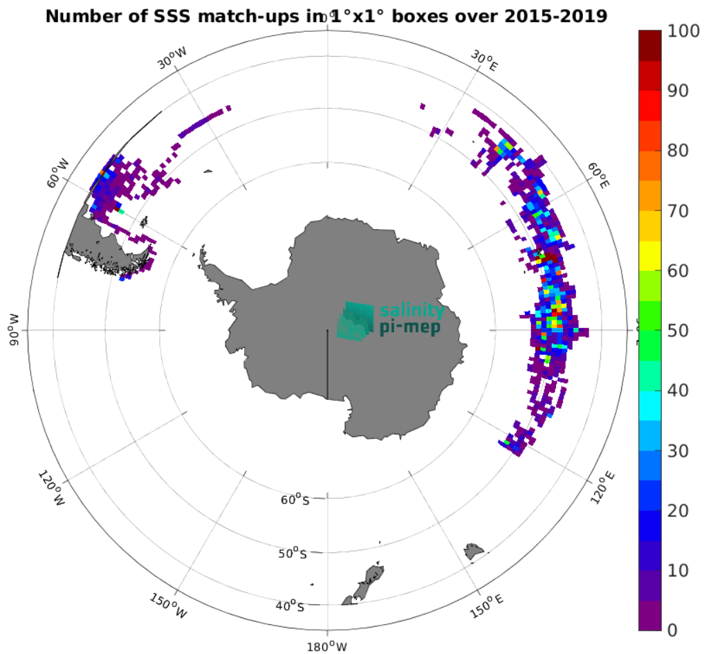
Figure 4: Number of SSS match-ups between Marine mammals SSS and the SMAP SSS L2 v5 (RSS) SSS product for the Roaring Forties and Furious Fifties Pi-MEP region over 1^\circ \times 1^\circ boxes and for the full satellite product period.
