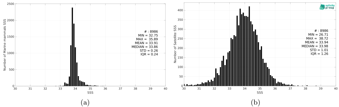
Figure 2: Histograms of SSS from Marine mammals (a) and SMAP SSS L2 v5 (RSS) (b) considering all match-up pairs per bins of 0.1 over the Roaring Forties and Furious Fifties Pi-MEP region and for the full satellite product period.
