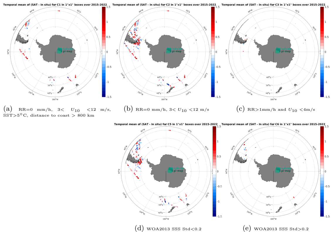
Figure 14: Temporal mean gridded over spatial boxes of size 1^\circ \times 1^\circ of \Delta SSS (SMAP SSS L2 v5.3 (RSS) - TSG (SAMOS)) for 5 different subdatasets corresponding to:RR=0 mm/h, 3 < U_{10} < 12 m/s, SST>5°C, distance to coast > 800 km (a), RR=0 mm/h, 3 < U_{10} < 12 m/s (b), RR>1mm/h and U_{10} < 4 m/s (c), WOA2013 SSS Std<0.2 (d), WOA2013 SSS Std>0.2 (e).
