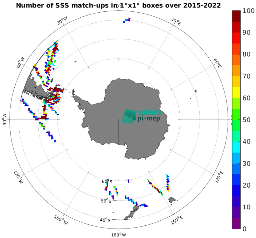
Figure 5: Number of SSS match-ups between TSG (SAMOS) SSS and the SMAP SSS L2 v5.3 (RSS) SSS product for the Roaring Forties and Furious Fifties Pi-MEP region over 1^\circ \times 1^\circ boxes and for the full satellite product period.
