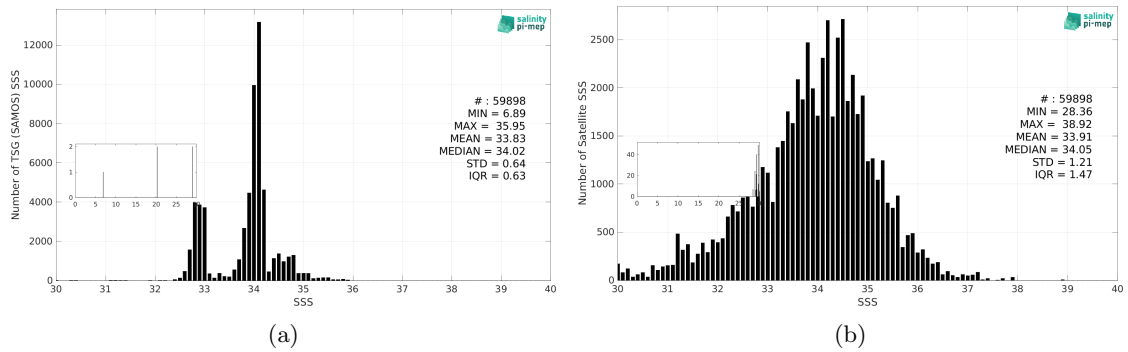
Figure 3: Histograms of SSS from TSG (SAMOS) (a) and SMAP SSS L2 v5.3 (RSS) (b) considering all match-up pairs per bins of 0.1 over the Roaring Forties and Furious Fifties Pi-MEP region and for the full satellite product period.
