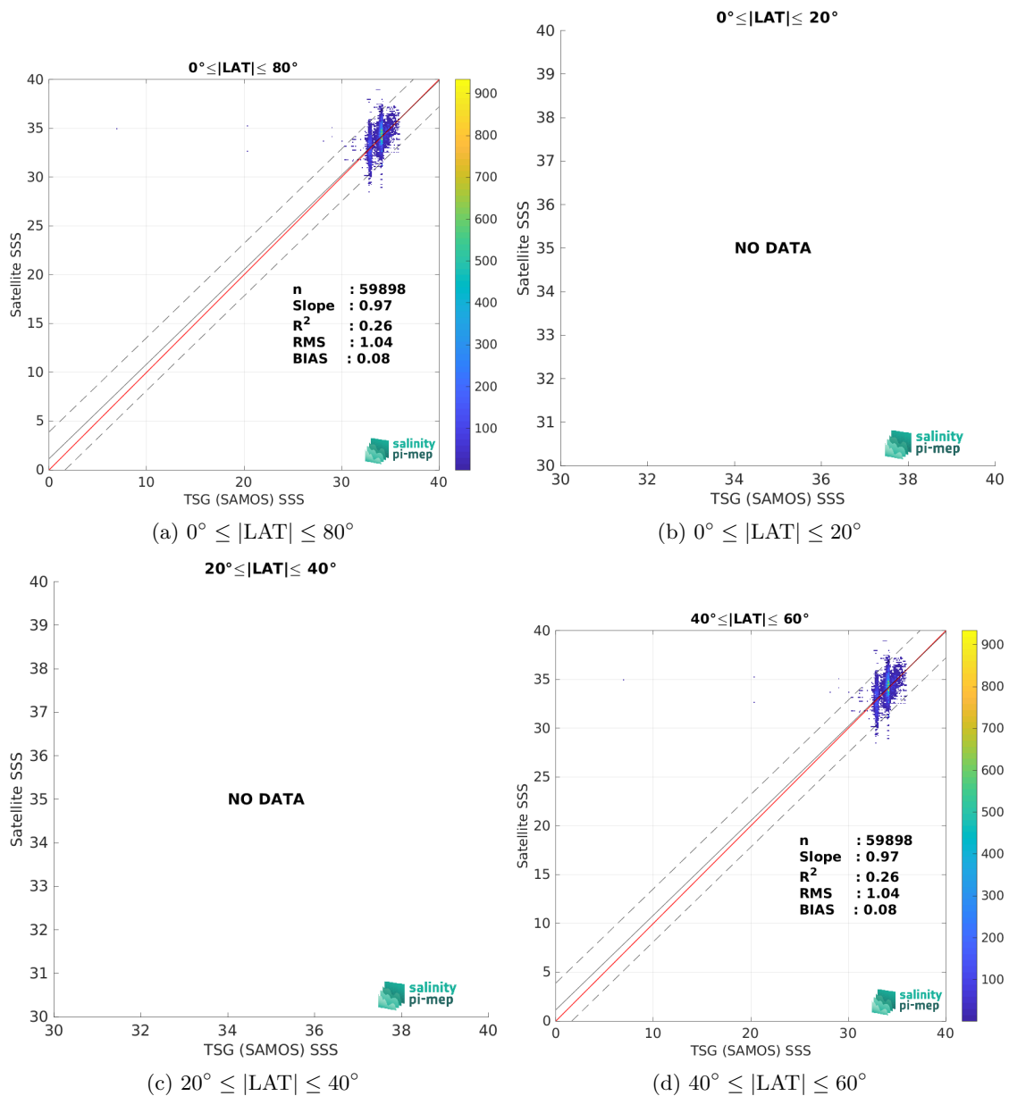
Figure 10: Contour maps of the concentration of SMAP SSS L2 v5.3 (RSS) SSS (y-axis) versus TSG (SAMOS) SSS (x-axis) at match-up pairs for different latitude bands. For each plot, the red line shows x=y . The black thin and dashed lines indicate a linear fit through the data cloud and the \pm 95\% confidence levels, respectively. The number match-up pairs n , the slope and R^2 coefficient of the linear fit, the root mean square (RMS) and the mean bias between satellite and in situ data are indicated for each latitude band in each plots.
