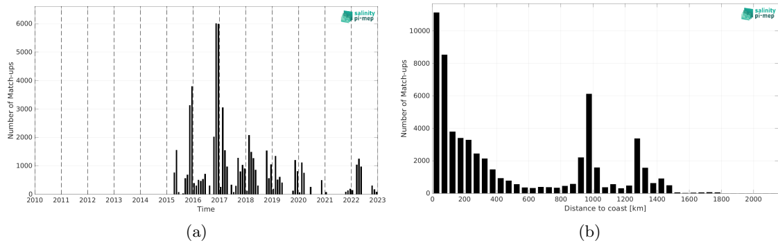
Figure 2: Number of match-ups between TSG (SAMOS) and SMAP SSS L2 v5.3 (RSS) SSS as a function of time (a) and as function of the distance to coast (b) over the Roaring Forties and Furious Fifties Pi-MEP region and for the full satellite product period.
