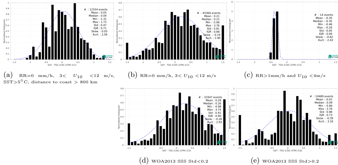
Figure 15: Normalized histogram of \Delta SSS (SMAP SSS L2 v5.3 (RSS) - TSG (CSIC-UTM)) for 5 different subdatasets corresponding to: RR=0 mm/h, 3 < U_{10} < 12 m/s, SST > 5°C, distance to coast > 800 km (a), RR=0 mm/h, 3 < U_{10} < 12 m/s (b), RR > 1 mm/h and U_{10} < 4 m/s (c), WOA2013 SSS Std < 0.2 (d), WOA2013 SSS Std > 0.2 (e).
