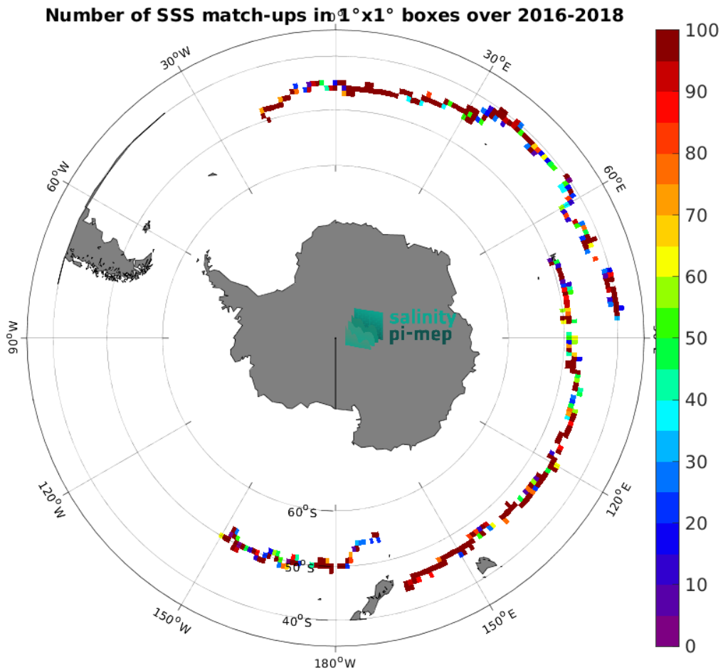
Figure 4: Number of SSS match-ups between Surface drifters SSS and the SMAP SSS L2 v5.3 (RSS) SSS product for the Roaring Forties and Furious Fifties Pi-MEP region over 1^\circ \times 1^\circ boxes and for the full satellite product period.
