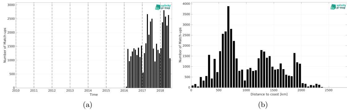
Figure 2: Number of match-ups between Surface drifters and SMAP SSS L2 v5.3 (RSS) SSS as a function of time (a) and as function of the distance to coast (b) over the Roaring Forties and Furious Fifties Pi-MEP region and for the full satellite product period.
