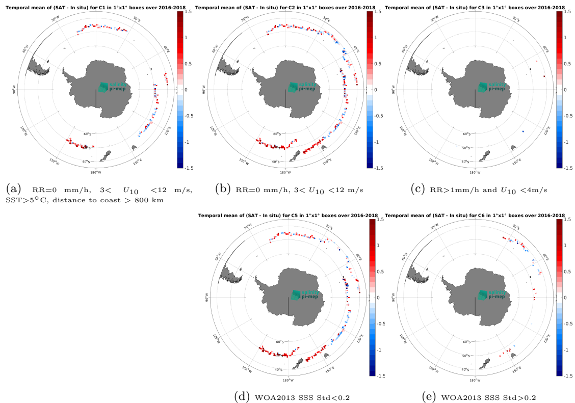
Figure 13: Temporal mean gridded over spatial boxes of size 1^\circ \times 1^\circ of \Delta SSS (SMAP SSS L2 v5.3 (RSS) - Surface drifters) for 5 different subdatasets corresponding to:RR=0 mm/h, 3 < U_{10} < 12 m/s, SST > 5^\circ\text{C} , distance to coast > 800 km (a), RR=0 mm/h, 3 < U_{10} < 12 m/s (b), RR > 1 mm/h and U_{10} < 4 m/s (c), WOA2013 SSS Std < 0.2 (d), WOA2013 SSS Std > 0.2 (e).
