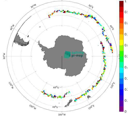
(f) Std( \Delta SSS) (Satellite - Surface drifters)
