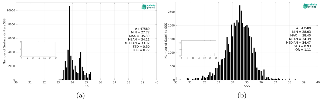
Figure 3: Histograms of SSS from Surface drifters (a) and SMAP SSS L2 v5.3 (RSS) (b) considering all match-up pairs per bins of 0.1 over the Roaring Forties and Furious Fifties Pi-MEP region and for the full satellite product period.
