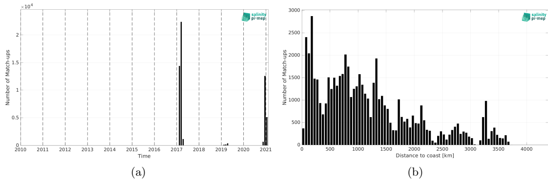
Figure 2: Number of match-ups between TSG (GOSUD-Sailing-ship) and SMAP SSS L2 v5.3 - 40 km (RSS) SSS as a function of time (a) and as function of the distance to coast (b) over the Roaring Forties and Furious Fifties Pi-MEP region and for the full satellite product period.
