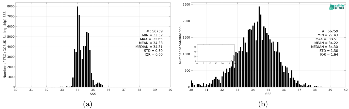
Figure 3: Histograms of SSS from TSG (GOSUD-Sailing-ship) (a) and SMAP SSS L2 v5.3 - 40 km (RSS) (b) considering all match-up pairs per bins of 0.1 over the Roaring Forties and Furious Fifties Pi-MEP region and for the full satellite product period.
