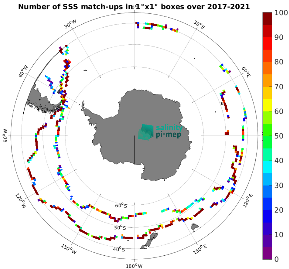
Figure 5: Number of SSS match-ups between TSG (GOSUD-Sailing-ship) SSS and the SMAP SSS L2 v5.3 - 40 km (RSS) SSS product for the Roaring Forties and Furious Fifties Pi-MEP region over 1^\circ \times 1^\circ boxes and for the full satellite product period.
