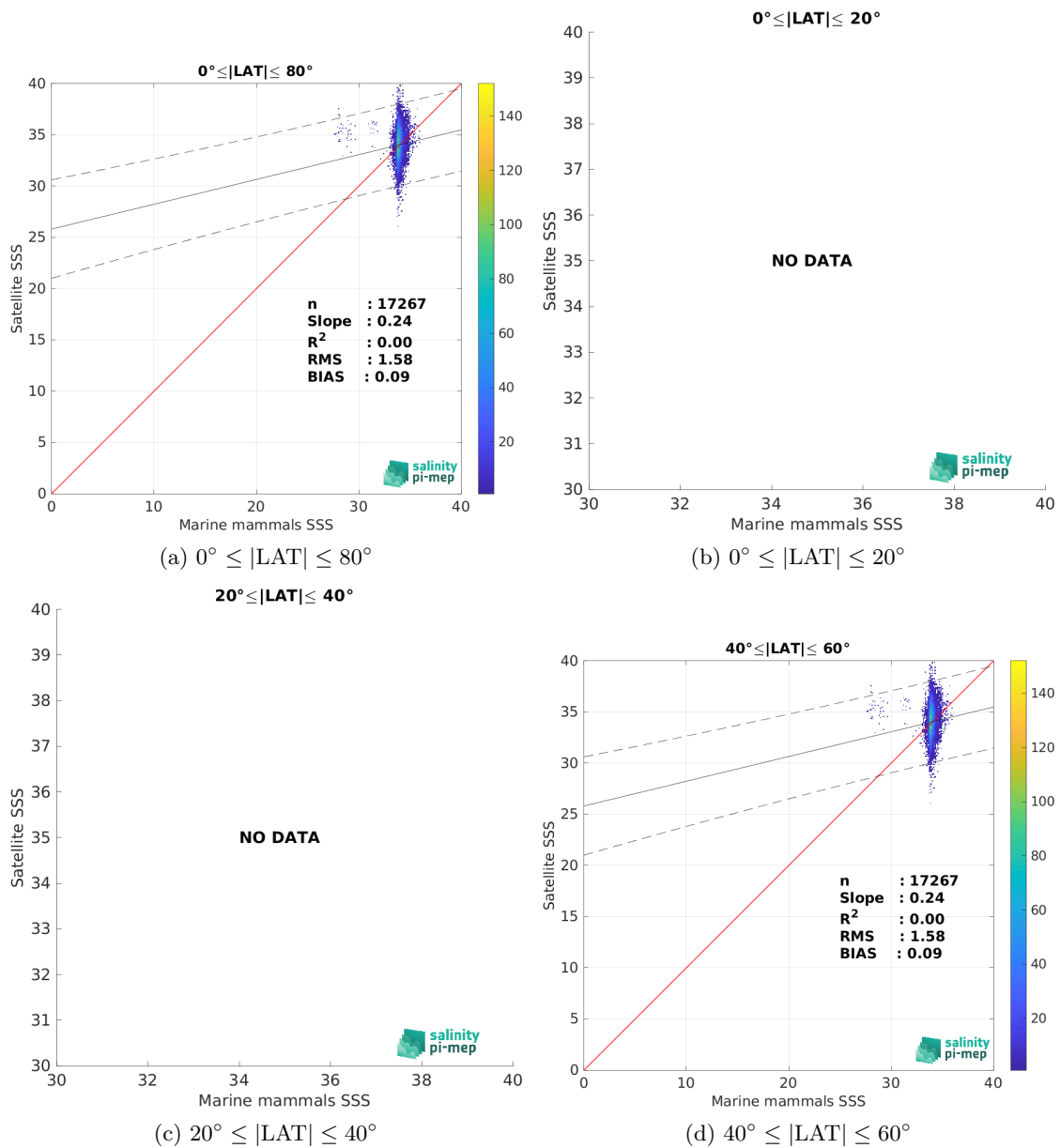
Figure 10: Contour maps of the concentration of SMAP SSS L2 v5.3 - 40 km (RSS) SSS (y-axis) versus Marine mammals SSS (x-axis) at match-up pairs for different latitude bands. For each plot, the red line shows x=y . The black thin and dashed lines indicate a linear fit through the data cloud and the \pm 95\% confidence levels, respectively. The number match-up pairs n , the slope and R^2 coefficient of the linear fit, the root mean square (RMS) and the mean bias between satellite and in situ data are indicated for each latitude band in each plots.
