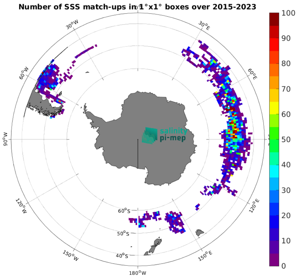
Figure 5: Number of SSS match-ups between Marine mammals SSS and the SMAP SSS L2 v5.3 - 40 km (RSS) SSS product for the Roaring Forties and Furious Fifties Pi-MEP region over 1^\circ \times 1^\circ boxes and for the full satellite product period.
