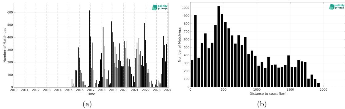
Figure 2: Number of match-ups between Marine mammals and SMAP SSS L2 v5.3 - 40 km (RSS) SSS as a function of time (a) and as function of the distance to coast (b) over the Roaring Forties and Furious Fifties Pi-MEP region and for the full satellite product period.
