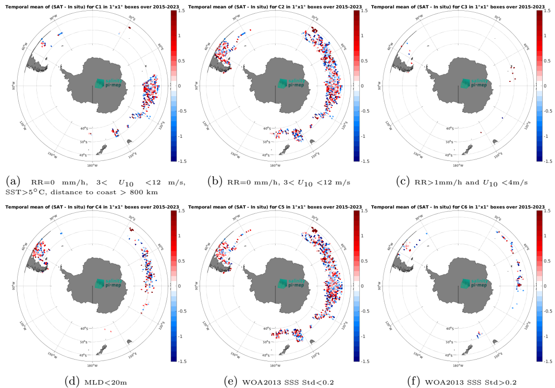
Figure 14: Temporal mean gridded over spatial boxes of size 1^\circ \times 1^\circ of \Delta SSS (SMAP SSS L2 v5.3 - 40 km (RSS) - Marine mammals) for 6 different subdatasets corresponding to: RR=0 mm/h, 3 < U_{10} < 12 m/s, SST > 5°C, distance to coast > 800 km (a), RR=0 mm/h, 3 < U_{10} < 12 m/s (b), RR > 1mm/h and U_{10} < 4 m/s (c), MLD < 20m (d), WOA2013 SSS Std < 0.2 (e), WOA2013 SSS Std > 0.2 (f).
