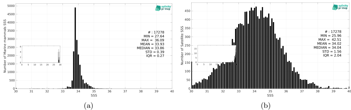
Figure 3: Histograms of SSS from Marine mammals (a) and SMAP SSS L2 v5.3 - 40 km (RSS) (b) considering all match-up pairs per bins of 0.1 over the Roaring Forties and Furious Fifties Pi-MEP region and for the full satellite product period.
