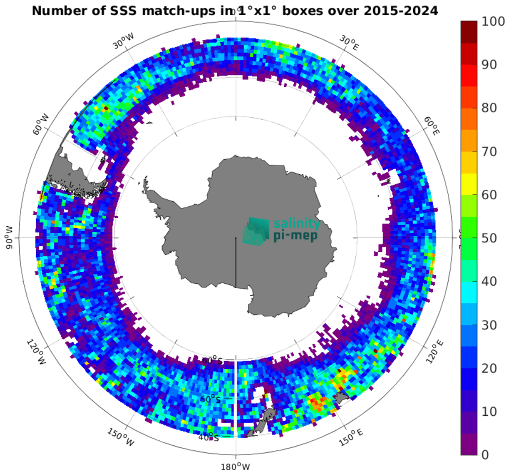
Figure 5: Number of SSS match-ups between Argo SSS and the SMAP SSS L2 v5.3 - 40 km (RSS) SSS product for the Roaring Forties and Furious Fifties Pi-MEP region over 1^\circ \times 1^\circ boxes and for the full satellite product period.
