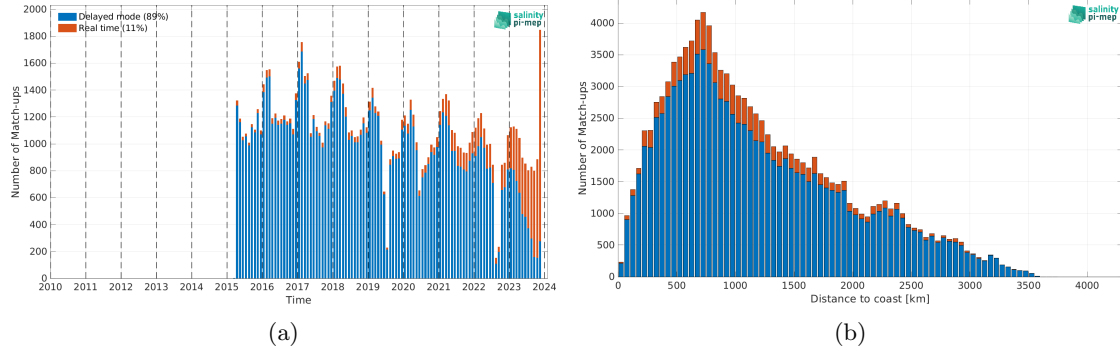
Figure 2: Number of match-ups between Argo and SMAP SSS L2 v5.3 - 40 km (RSS) SSS as a function of time (a) and as function of the distance to coast (b) over the Roaring Forties and Furious Fifties Pi-MEP region and for the full satellite product period.
