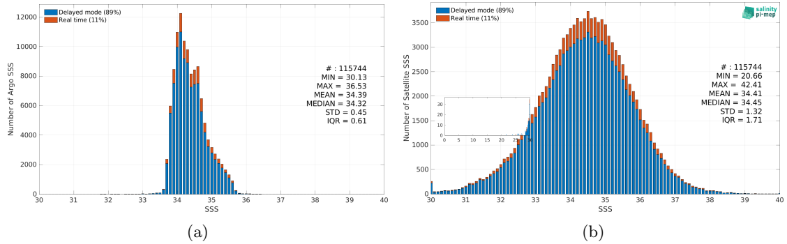
Figure 3: Histograms of SSS from Argo (a) and SMAP SSS L2 v5.3 - 40 km (RSS) (b) considering all match-up pairs per bins of 0.1 over the Roaring Forties and Furious Fifties Pi-MEP region and for the full satellite product period.
