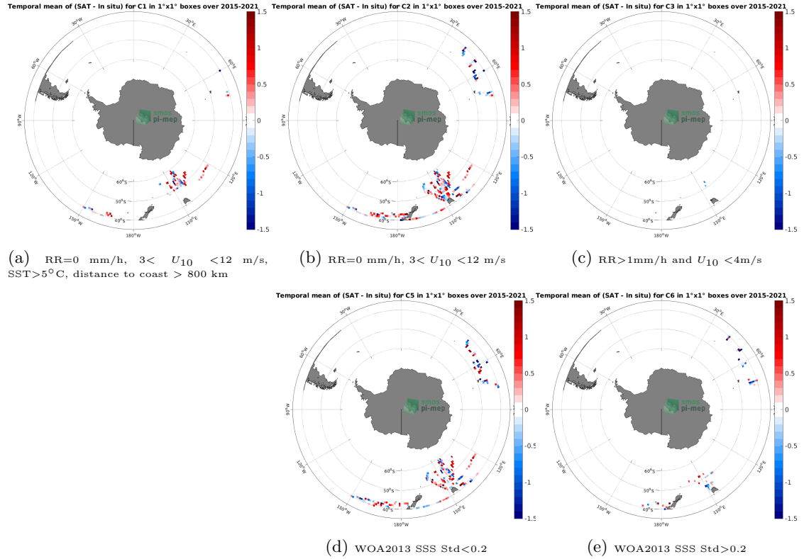
Figure 12: Temporal mean gridded over spatial boxes of size 1^{\circ}\times 1^{\circ} of \Delta\text{SSS} (SMAP SSS L2 v5 - 40 km (RSS) - TSG (LEGOS-DM)) for 5 different subdatasets corresponding to:RR=0 mm/h, 3 < U_{10} < 12 m/s, SST >5^{\circ}\text{C} , distance to coast > 800 km (a), RR=0 mm/h, 3 < U_{10} < 12 m/s (b), RR >1 mm/h and U_{10} < 4 m/s (c), WOA2013 SSS Std <0.2 (d), WOA2013 SSS Std >0.2 (e).
