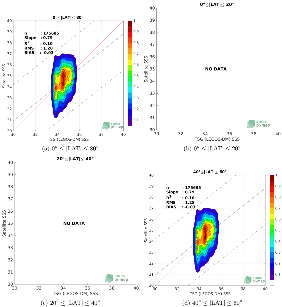
Figure 9: Contour maps of the concentration of SMAP SSS L2 v5 - 40 km (RSS) SSS (y-axis) versus TSG (LEGOS-DM) SSS (x-axis) at match-up pairs for different latitude bands. For each plot, the red line shows x=y . The black thin and dashed lines indicate a linear fit through the data cloud and the \pm 95\% confidence levels, respectively. The number match-up pairs n , the slope and R^2 coefficient of the linear fit, the root mean square (RMS) and the mean bias between satellite and in situ data are indicated for each latitude band in each plot.
