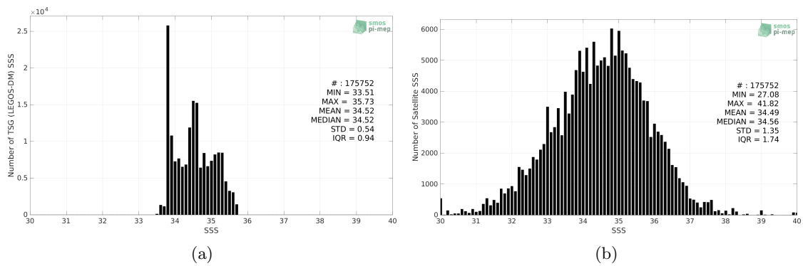
Figure 2: Histograms of SSS from TSG (LEGOS-DM) (a) and SMAP SSS L2 v5 - 40 km (RSS) (b) considering all match-up pairs per bins of 0.1 over the Roaring Forties and Furious Fifties Pi-MEP region and for the full satellite product period.
