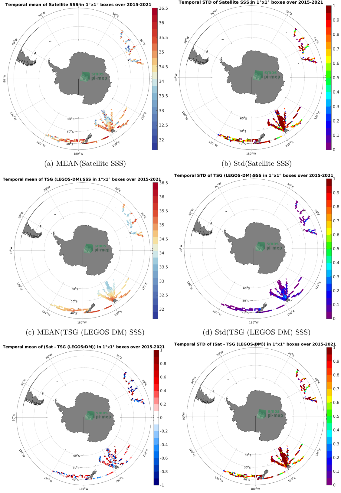
Figure 6: Temporal mean (left) and Std (right) of SSS from SMAP SSS L2 v5 - 40 km (RSS) (top), TSG (LEGOS-DM) (middle), and of \Delta SSS (Satellite - TSG (LEGOS-DM)). Only match-up pairs are used to generate these maps.
