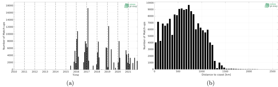
Figure 1: Number of match-ups between TSG (LEGOS-DM) and SMAP SSS L2 v5 - 40 km (RSS) SSS as a function of time (a) and as function of the distance to coast (b) over the Roaring Forties and Furious Fifties Pi-MEP region and for the full satellite product period.
