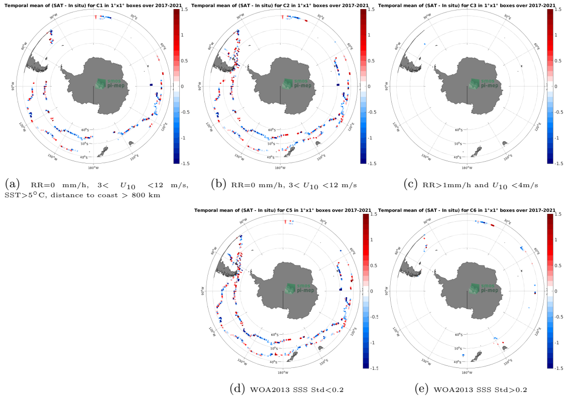
Figure 12: Temporal mean gridded over spatial boxes of size 1^\circ \times 1^\circ of \Delta SSS (SMAP SSS L2 v5 - 40 km (RSS) - TSG (GOSUD-Sailing-ship)) for 5 different subdatasets corresponding to:RR=0 mm/h, 3 < U_{10} < 12 m/s, SST>5°C, distance to coast > 800 km (a), RR=0 mm/h, 3 < U_{10} < 12 m/s (b), RR>1mm/h and U_{10} < 4 m/s (c), WOA2013 SSS Std<0.2 (d), WOA2013 SSS Std>0.2 (e).
