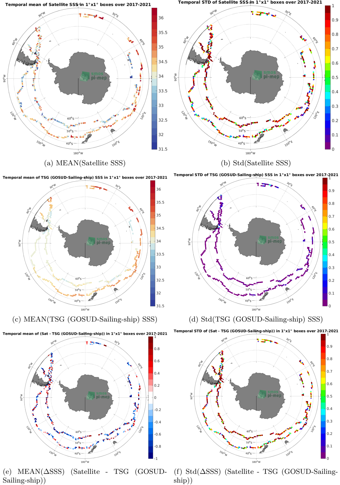
Figure 6: Temporal mean (left) and Std (right), of SSS from SMAP SSS L2 v5 - 40 km (RSS) (top), TSG (GOSUD-Sailing-ship) (middle), and of \Delta SSS (Satellite - TSG (GOSUD-Sailing-ship)). Only match-up pairs are used to generate these maps.
