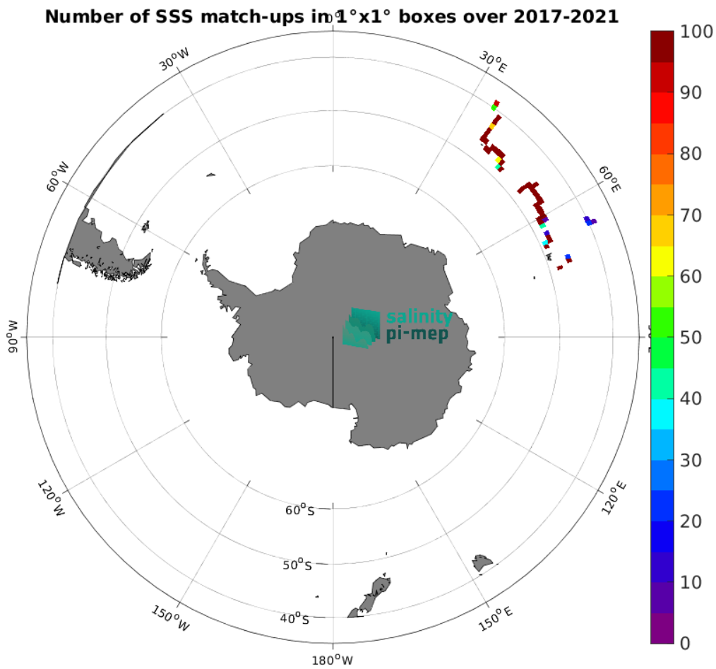
Figure 4: Number of SSS match-ups between TSG (GOSUD-Research-vessel) SSS and the SMAP SSS L2 v5 - 40 km (RSS) SSS product for the Roaring Forties and Furious Fifties Pi-MEP region over 1^{\circ} \times 1^{\circ} boxes and for the full satellite product period.
