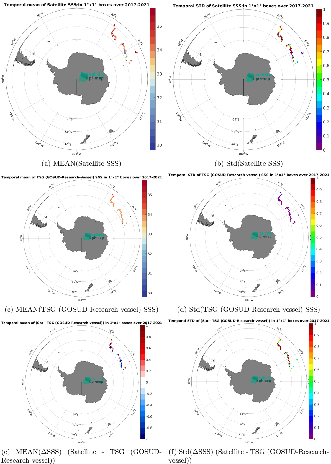
Figure 6: Temporal mean (left) and Std (right) of SSS from SMAP SSS L2 v5 - 40 km (RSS) (top), TSG (GOSUD-Research-vessel) (middle), and of \Delta SSS (Satellite - TSG (GOSUD-Research-vessel)). Only match-up pairs are used to generate these maps.
