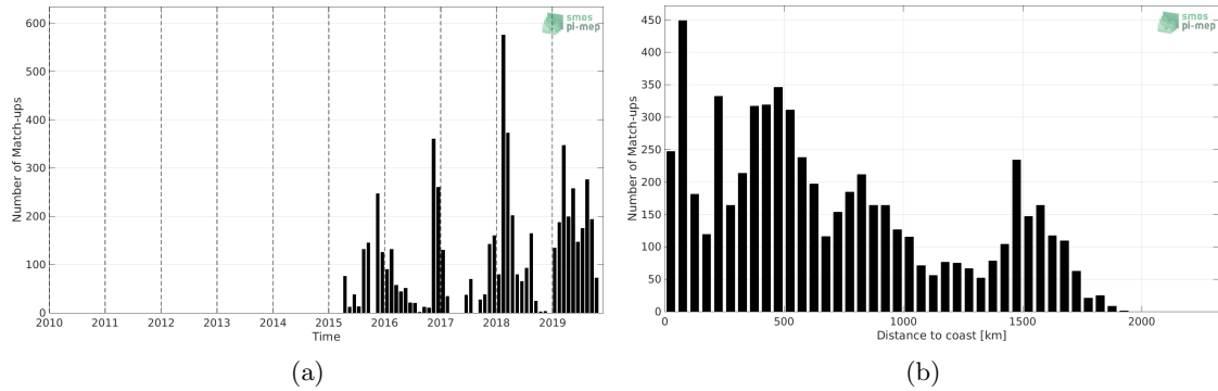
Figure 1: Number of match-ups between Marine mammals and SMAP SSS L2 v4 (RSS) SSS as a function of time (a) and as function of the distance to coast (b) over the Roaring Forties and Furious Fifties Pi-MEP region and for the full satellite product period.
