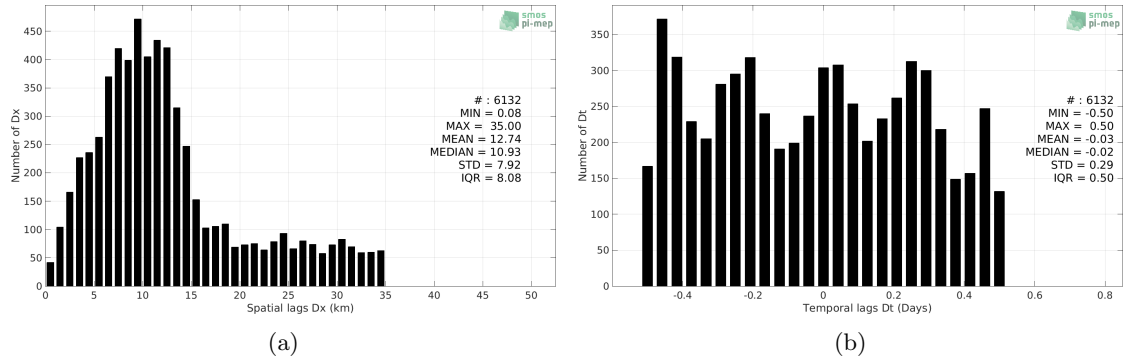
Figure 5: Histograms of the spatial (a) and temporal (b) lags between the location/time of the Marine mammals measurement and the date of the corresponding SMAP SSS L2 v4 (RSS) SSS pixel.
