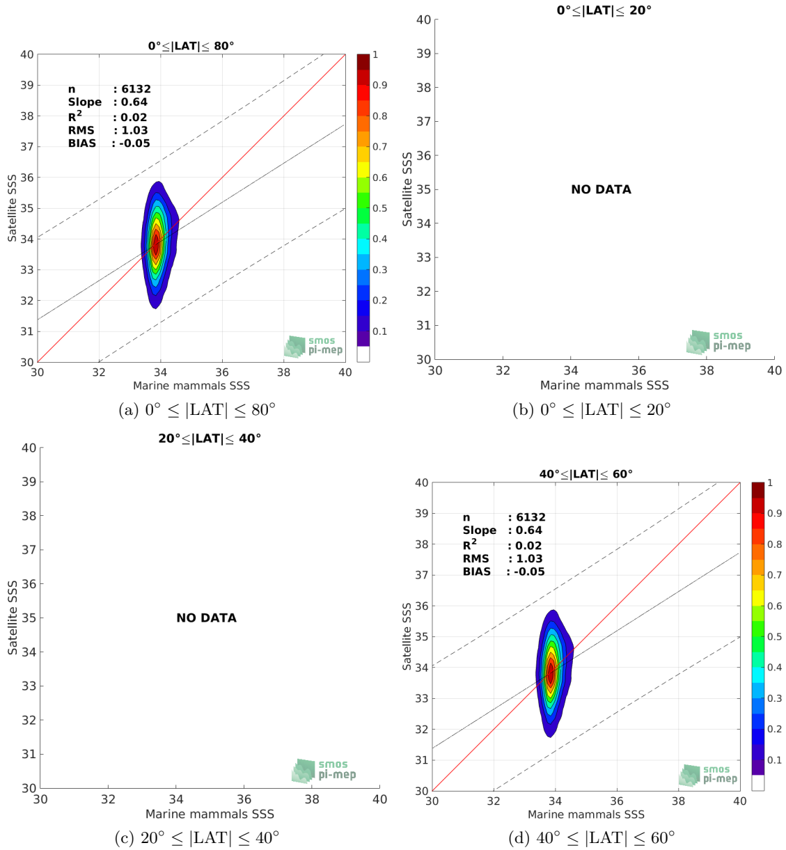
Figure 9: Contour maps of the concentration of SMAP SSS L2 v4 (RSS) SSS (y-axis) versus Marine mammals SSS (x-axis) at match-up pairs for different latitude bands. For each plot, the red line shows x=y . The black thin and dashed lines indicate a linear fit through the data cloud and the \pm 95\% confidence levels, respectively. The number match-up pairs n , the slope and R^2 coefficient of the linear fit, the root mean square (RMS) and the mean bias between satellite and in situ data are indicated for each latitude band in each plots.
