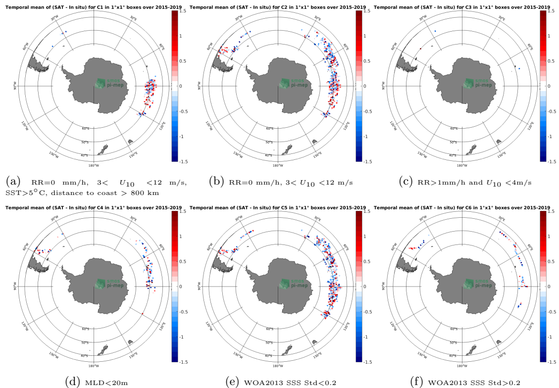
Figure 12: Temporal mean gridded over spatial boxes of size 1^{\circ}\times 1^{\circ} of \Delta\text{SSS} (SMAP SSS L2 v4 (RSS) - Marine mammals) for 6 different subdatasets corresponding to: \text{RR}=0 mm/h, 3 < U_{10} < 12 m/s, \text{SST}>5^{\circ}\text{C} , distance to coast > 800 km (a), \text{RR}=0 mm/h, 3 < U_{10} < 12 m/s (b), \text{RR}>1 mm/h and U_{10} < 4 m/s (c), \text{MLD}<20\text{m} (d), \text{WOA2013 SSS Std}<0.2 (e), \text{WOA2013 SSS Std}>0.2 (f).
