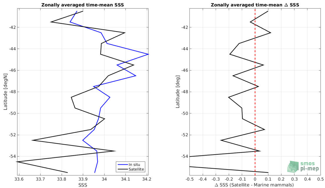
Figure 8: Left panel: Zonal mean SSS from SMAP SSS L2 v4 (RSS) satellite product (black) and from Marine mammals (blue). Right panel: Zonal mean of \Delta SSS (Satellite - Marine mammals) for all the collected Pi-MEP match-up pairs estimated over the full satellite product period.
