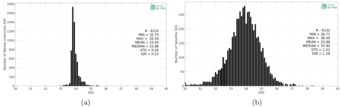
Figure 2: Histograms of SSS from Marine mammals (a) and SMAP SSS L2 v4 (RSS) (b) considering all match-up pairs per bins of 0.1 over the Roaring Forties and Furious Fifties Pi-MEP region and for the full satellite product period.
