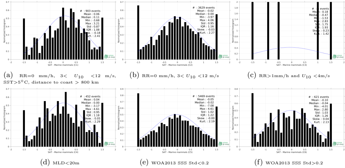
Figure 13: Normalized histogram of \Delta SSS (SMAP SSS L2 v4 (RSS) - Marine mammals) for 6 different subdatasets corresponding to: RR=0 mm/h, 3 < U_{10} < 12 m/s, SST>5°C, distance to coast > 800 km (a), RR=0 mm/h, 3 < U_{10} < 12 m/s (b), RR>1mm/h and U_{10} < 4 m/s (c), MLD<20m (d), WOA2013 SSS Std<0.2 (e), WOA2013 SSS Std>0.2 (f).
