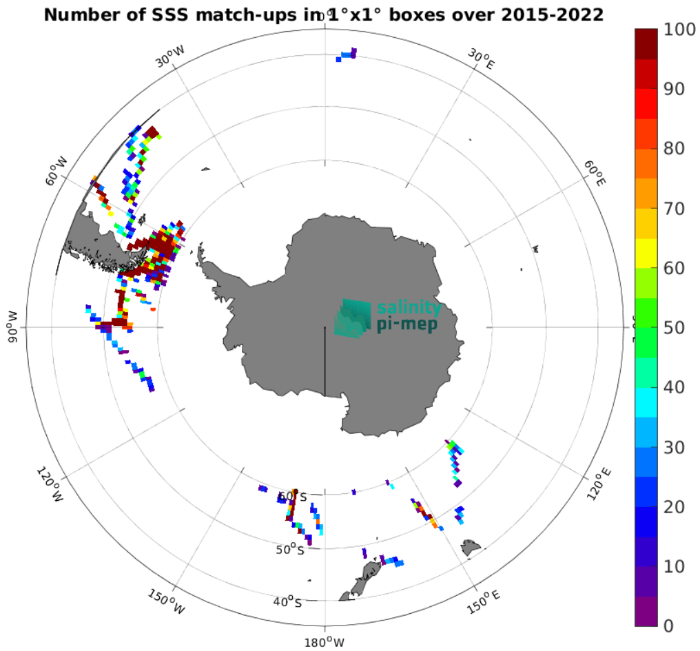
Figure 5: Number of SSS match-ups between TSG (SAMOS) SSS and the SMAP SSS L2 v5.0 (JPL) SSS product for the Roaring Forties and Furious Fifties Pi-MEP region over 1^\circ \times 1^\circ boxes and for the full satellite product period.
