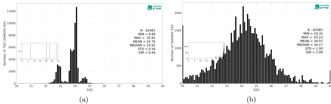
Figure 3: Histograms of SSS from TSG (SAMOS) (a) and SMAP SSS L2 v5.0 (JPL) (b) considering all match-up pairs per bins of 0.1 over the Roaring Forties and Furious Fifties Pi-MEP region and for the full satellite product period.
