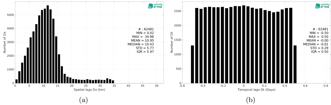
Figure 6: Histograms of the spatial (a) and temporal (b) lags between the location/time of the TSG (SAMOS) measurement and the date of the corresponding SMAP SSS L2 v5.0 (JPL) SSS pixel.
