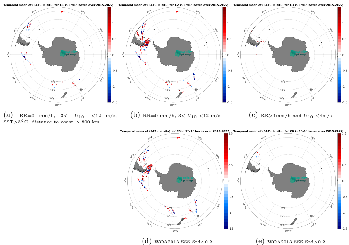
Figure 14: Temporal mean gridded over spatial boxes of size 1^\circ \times 1^\circ of \Delta SSS (SMAP SSS L2 v5.0 (JPL) - TSG (SAMOS)) for 5 different subdatasets corresponding to:RR=0 mm/h, 3 < U_{10} < 12 m/s, SST>5°C, distance to coast > 800 km (a), RR=0 mm/h, 3 < U_{10} < 12 m/s (b), RR>1mm/h and U_{10} < 4 m/s (c), WOA2013 SSS Std<0.2 (d), WOA2013 SSS Std>0.2 (e).
