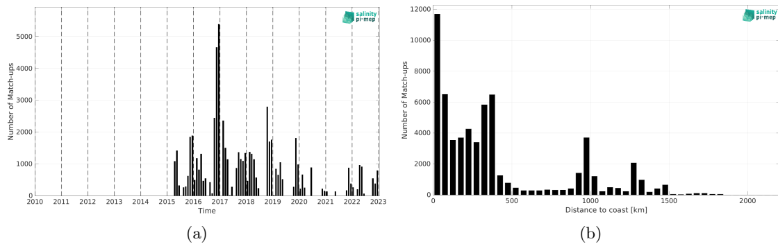
Figure 2: Number of match-ups between TSG (SAMOS) and SMAP SSS L2 v5.0 (JPL) SSS as a function of time (a) and as function of the distance to coast (b) over the Roaring Forties and Furious Fifties Pi-MEP region and for the full satellite product period.
