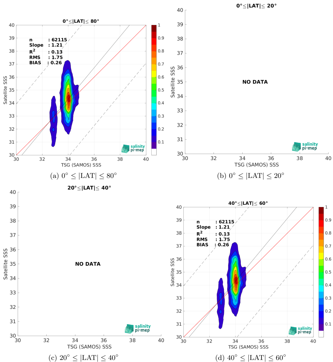
Figure 10: Contour maps of the concentration of SMAP SSS L2 v5.0 (JPL) SSS (y-axis) versus TSG (SAMOS) SSS (x-axis) at match-up pairs for different latitude bands. For each plot, the red line shows x=y . The black thin and dashed lines indicate a linear fit through the data cloud and the \pm 95\% confidence levels, respectively. The number match-up pairs n , the slope and R^2 coefficient of the linear fit, the root mean square (RMS) and the mean bias between satellite and in situ data are indicated for each latitude band in each plots.
