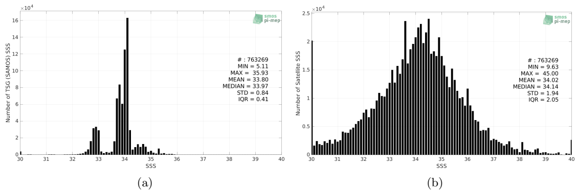
Figure 2: Histograms of SSS from TSG (SAMOS) (a) and SMAP SSS L2 v5.0 (JPL) (b) considering all match-up pairs per bins of 0.1 over the Roaring Forties and Furious Fifties Pi-MEP region and for the full satellite product period.
