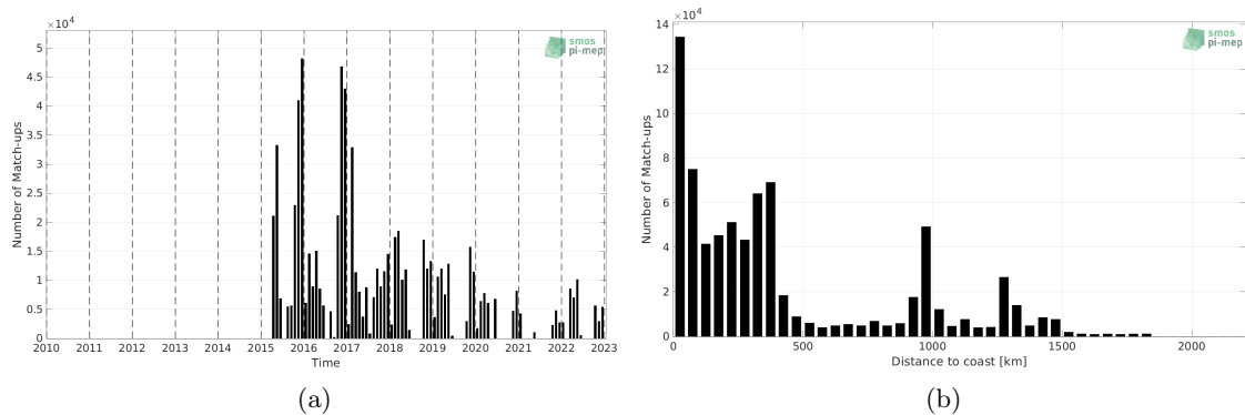
Figure 1: Number of match-ups between TSG (SAMOS) and SMAP SSS L2 v5.0 (JPL) SSS as a function of time (a) and as function of the distance to coast (b) over the Roaring Forties and Furious Fifties Pi-MEP region and for the full satellite product period.
