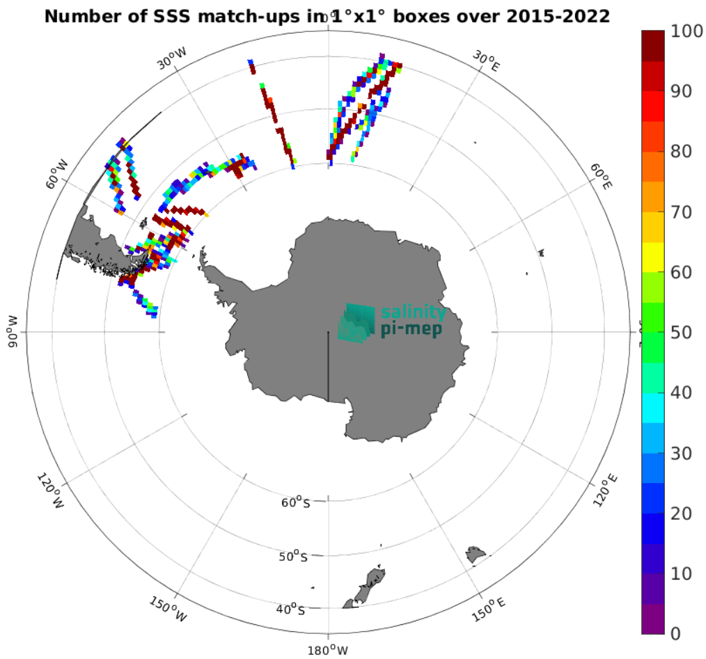
Figure 4: Number of SSS match-ups between TSG (Polarstern) SSS and the SMAP SSS L2 v5.0 (JPL) SSS product for the Roaring Forties and Furious Fifties Pi-MEP region over 1^\circ \times 1^\circ boxes and for the full satellite product period.
