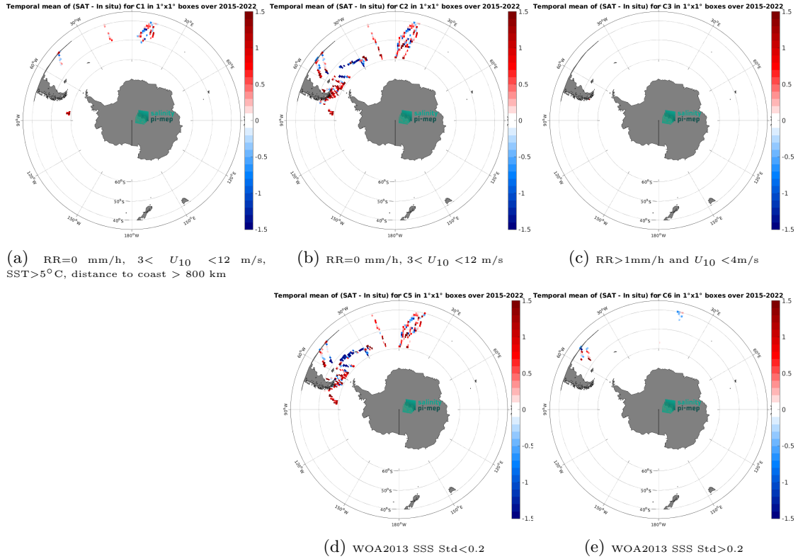
Figure 12: Temporal mean gridded over spatial boxes of size 1^{\circ}\times 1^{\circ} of \Delta\text{SSS} (SMAP SSS L2 v5.0 (JPL) - TSG (Polarstern)) for 5 different subdatasets corresponding to: \text{RR}=0 mm/h, 3 < U_{10} < 12 m/s, \text{SST}>5^{\circ}\text{C} , distance to coast > 800 km (a), \text{RR}=0 mm/h, 3 < U_{10} < 12 m/s (b), \text{RR}>1\text{mm/h} and U_{10} < 4\text{m/s} (c), WOA2013 SSS Std <0.2 (d), WOA2013 SSS Std >0.2 (e).
