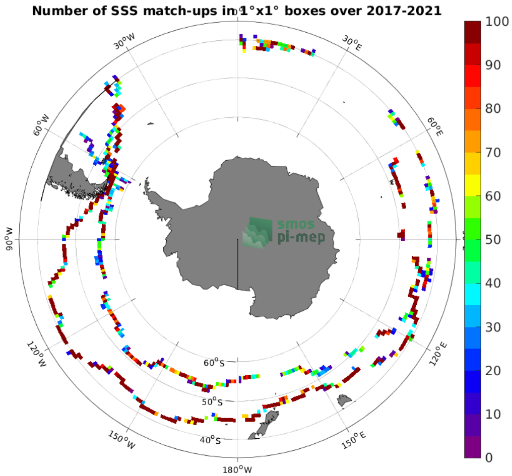
Figure 4: Number of SSS match-ups between TSG (GOSUD-Sailing-ship) SSS and the SMAP SSS L2 v5.0 (JPL) SSS product for the Roaring Forties and Furious Fifties Pi-MEP region over 1^\circ \times 1^\circ boxes and for the full satellite product period.
