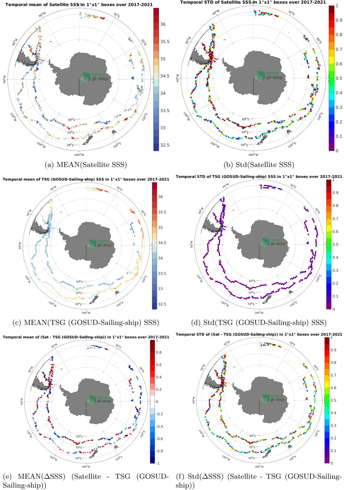
Figure 6: Temporal mean (left) and Std (right) of SSS from SMAP SSS L2 v5.0 (JPL) (top), TSG (GOSUD-Sailing-ship) (middle), and of \Delta SSS (Satellite - TSG (GOSUD-Sailing-ship)). Only match-up pairs are used to generate these maps.
