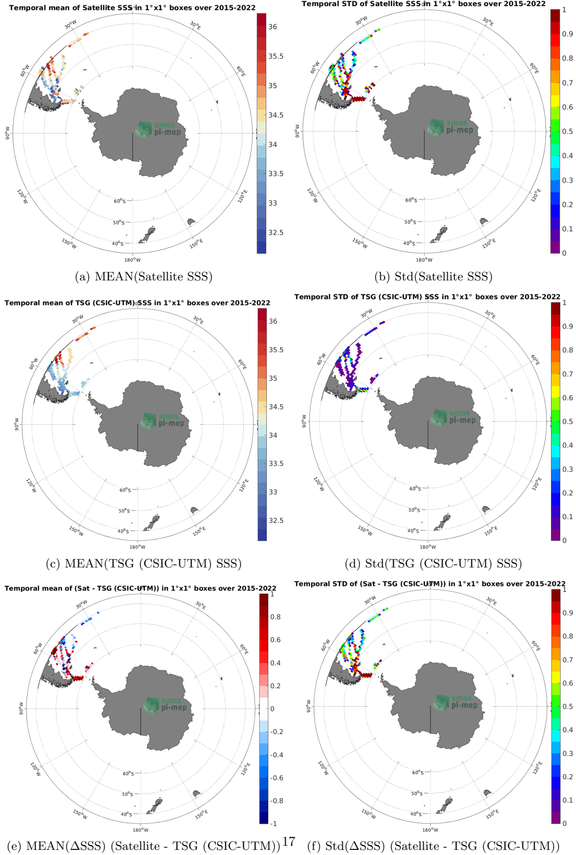
Figure 6: Temporal mean (left) and Std (right) of SSS from SMAP SSS L2 v5.0 (JPL) (top), TSG (CSIC-UTM) (middle), and of \Delta SSS (Satellite - TSG (CSIC-UTM)). Only match-up pairs are used to generate these maps.
