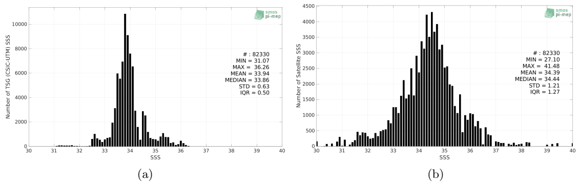
Figure 2: Histograms of SSS from TSG (CSIC-UTM) (a) and SMAP SSS L2 v5.0 (JPL) (b) considering all match-up pairs per bins of 0.1 over the Roaring Forties and Furious Fifties Pi-MEP region and for the full satellite product period.
