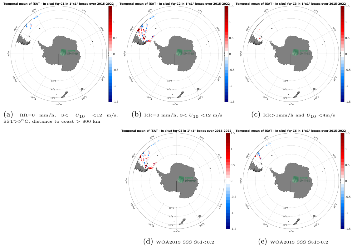
Figure 12: Temporal mean gridded over spatial boxes of size 1^{\circ}\times 1^{\circ} of \Delta\text{SSS} (SMAP SSS L2 v5.0 (JPL) - TSG (CSIC-UTM)) for 5 different subdatasets corresponding to:RR=0 mm/h, 3 < U_{10} < 12 m/s, SST >5^{\circ}\text{C} , distance to coast > 800 km (a), RR=0 mm/h, 3 < U_{10} < 12 m/s (b), RR >1 mm/h and U_{10} < 4 m/s (c), WOA2013 SSS Std <0.2 (d), WOA2013 SSS Std >0.2 (e).
