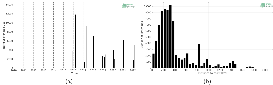
Figure 1: Number of match-ups between TSG (CSIC-UTM) and SMAP SSS L2 v5.0 (JPL) SSS as a function of time (a) and as function of the distance to coast (b) over the Roaring Forties and Furious Fifties Pi-MEP region and for the full satellite product period.
