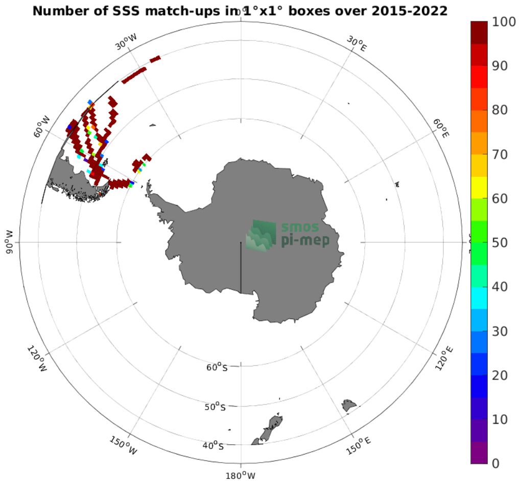
Figure 4: Number of SSS match-ups between TSG (CSIC-UTM) SSS and the SMAP SSS L2 v5.0 (JPL) SSS product for the Roaring Forties and Furious Fifties Pi-MEP region over 1^\circ \times 1^\circ boxes and for the full satellite product period.
