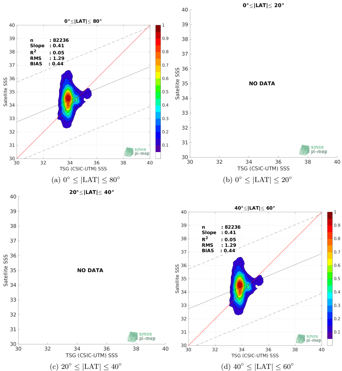
Figure 9: Contour maps of the concentration of SMAP SSS L2 v5.0 (JPL) SSS (y-axis) versus TSG (CSIC-UTM) SSS (x-axis) at match-up pairs for different latitude bands. For each plot, the red line shows x=y . The black thin and dashed lines indicate a linear fit through the data cloud and the \pm 95\% confidence levels, respectively. The number match-up pairs n , the slope and R^2 coefficient of the linear fit, the root mean square (RMS) and the mean bias between satellite and in situ data are indicated for each latitude band in each plot.
