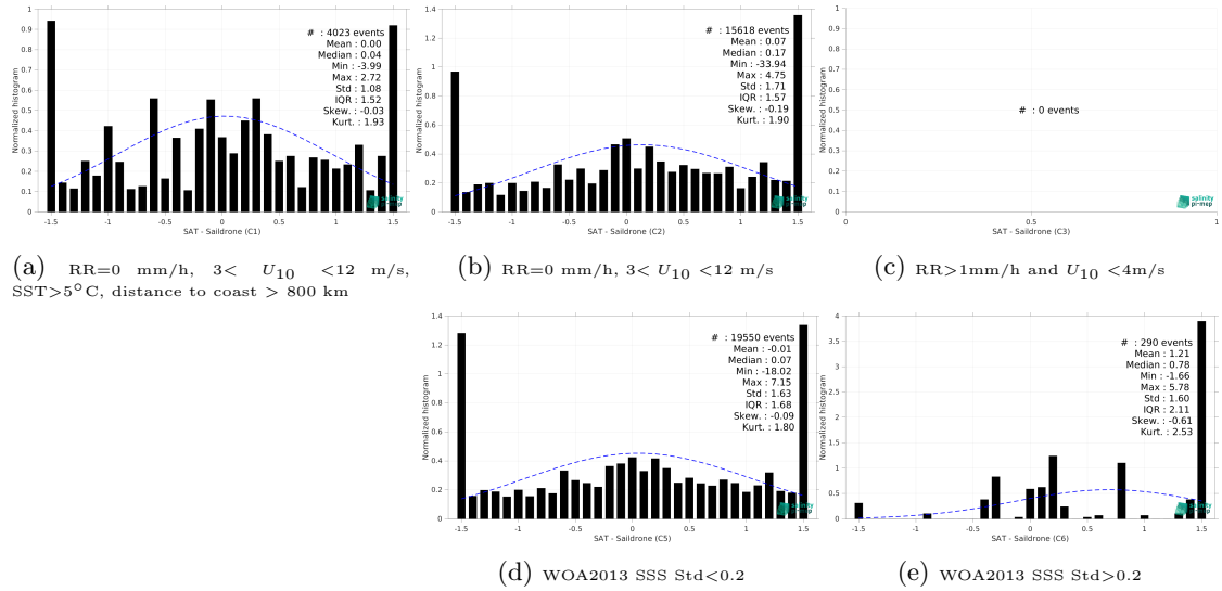
Figure 13: Normalized histogram of \Delta SSS (SMAP SSS L2 v5.0 (JPL) - Saildrone) for 5 different subdatasets corresponding to: RR=0 mm/h, 3 < U_{10} < 12 m/s, SST > 5°C, distance to coast > 800 km (a), RR=0 mm/h, 3 < U_{10} < 12 m/s (b), RR > 1mm/h and U_{10} < 4 m/s (c), WOA2013 SSS Std < 0.2 (d), WOA2013 SSS Std > 0.2 (e).
