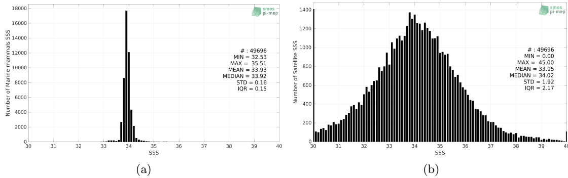
Figure 2: Histograms of SSS from Marine mammals (a) and SMAP SSS L2 v5.0 (JPL) (b) considering all match-up pairs per bins of 0.1 over the Roaring Forties and Furious Fifties Pi-MEP region and for the full satellite product period.
