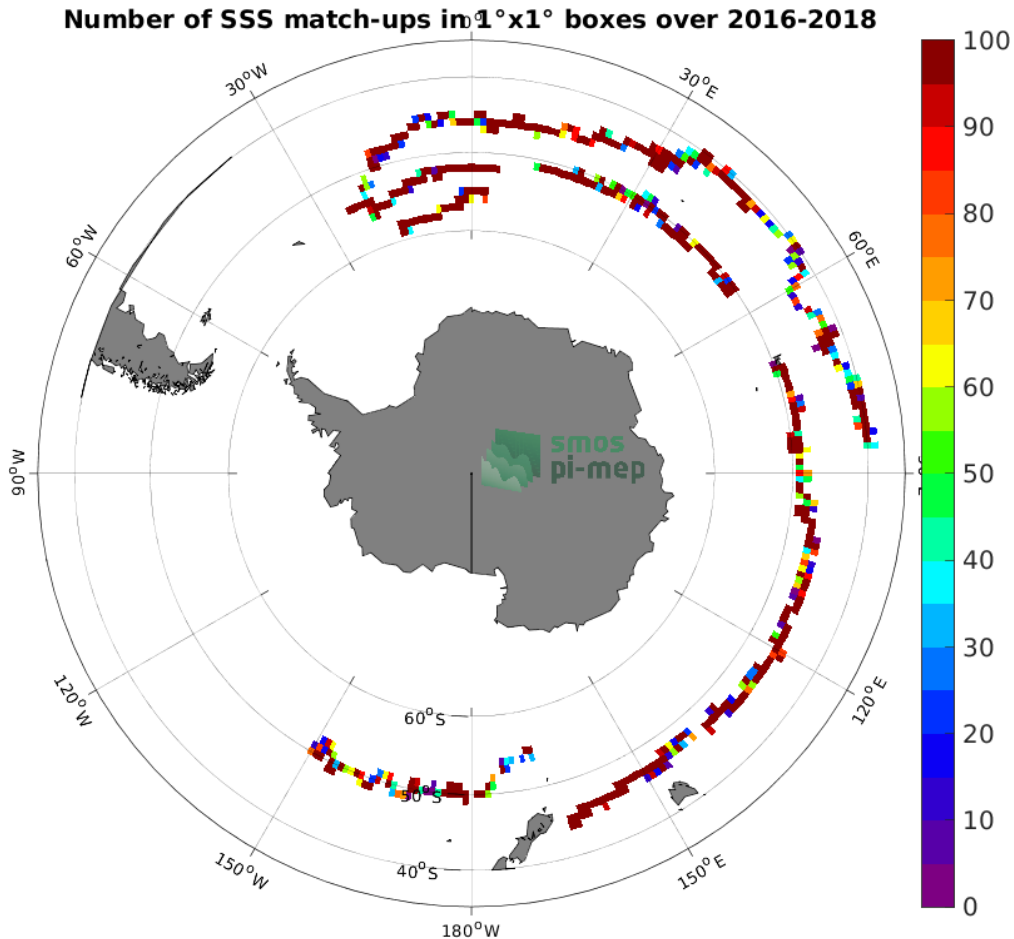
Figure 3: Number of SSS match-ups between Surface drifters SSS and the SMAP SSS L2 v5.0 (JPL) SSS product for the Roaring Forties and Furious Fifties Pi-MEP region over 1^\circ \times 1^\circ boxes and for the full satellite product period.
