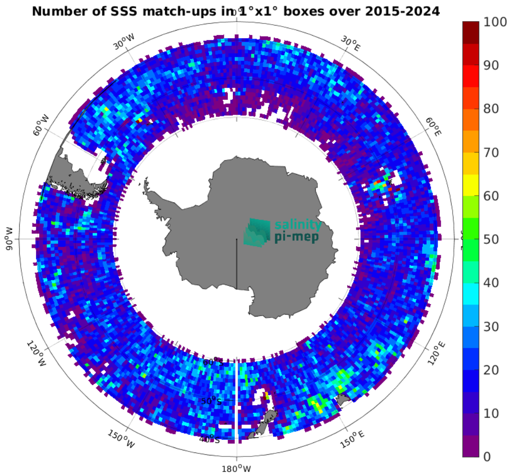
Figure 5: Number of SSS match-ups between Argo SSS and the SMAP SSS L2 v5.0 (JPL) SSS product for the Roaring Forties and Furious Fifties Pi-MEP region over 1^\circ \times 1^\circ boxes and for the full satellite product period.
