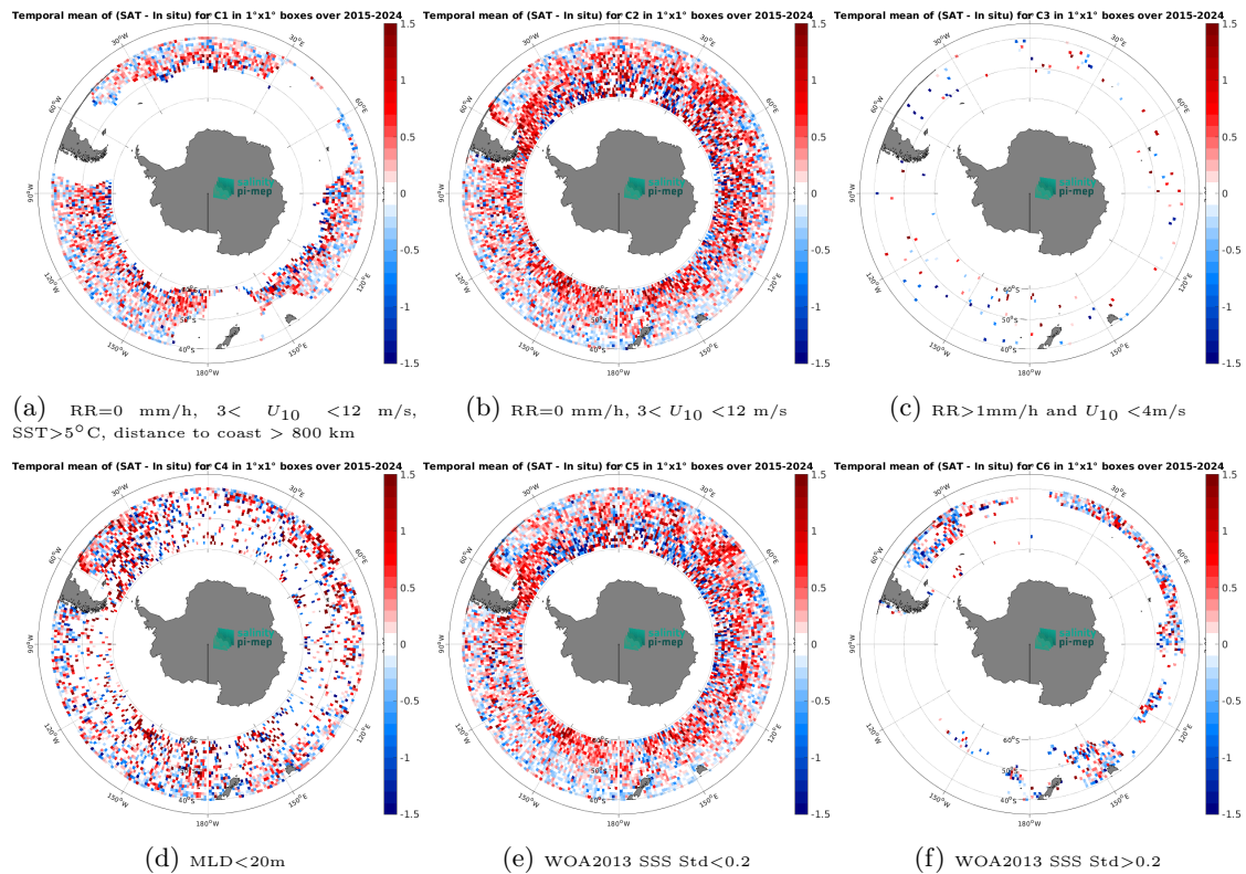
Figure 14: Temporal mean gridded over spatial boxes of size 1^\circ \times 1^\circ of \Delta SSS (SMAP SSS L2 v5.0 (JPL) - Argo) for 6 different subdatasets corresponding to:RR=0 mm/h, 3 < U_{10} < 12 m/s, SST>5°C, distance to coast > 800 km (a), RR=0 mm/h, 3 < U_{10} < 12 m/s (b), RR>1mm/h and U_{10} < 4 m/s (c),MLD<20m (d),WOA2013 SSS Std<0.2 (e),WOA2013 SSS Std>0.2 (f).
