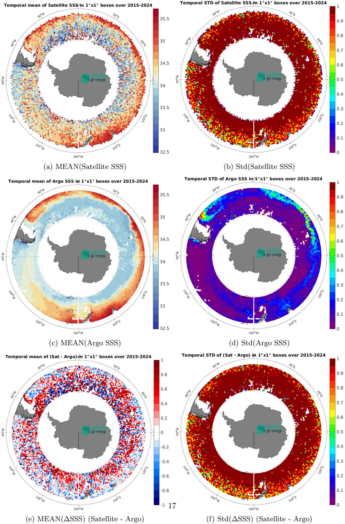
Figure 7: Temporal mean (left) and Std (right) of SSS from SMAP SSS L2 v5.0 (JPL) (top), Argo (middle), and of \Delta SSS (Satellite - Argo). Only match-up pairs are used to generate these maps.
