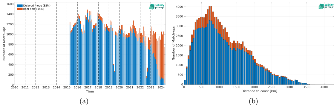
Figure 2: Number of match-ups between Argo and SMAP SSS L2 v5.0 (JPL) SSS as a function of time (a) and as function of the distance to coast (b) over the Roaring Forties and Furious Fifties Pi-MEP region and for the full satellite product period.
