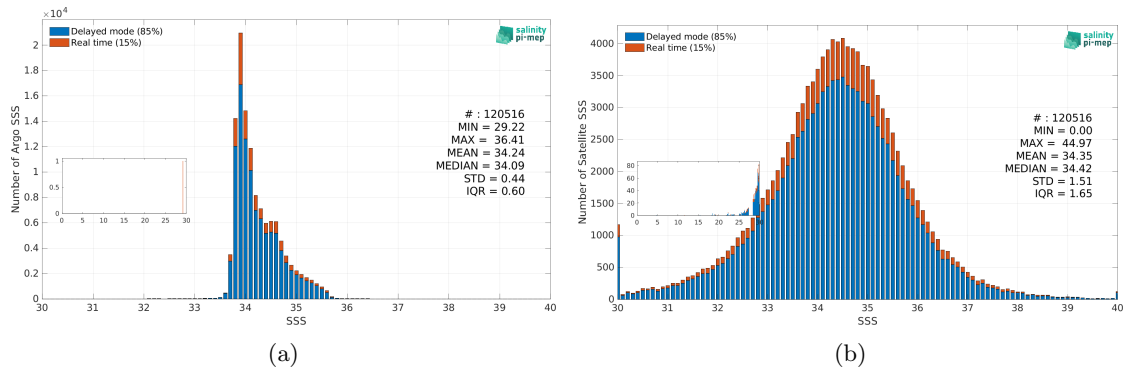
Figure 3: Histograms of SSS from Argo (a) and SMAP SSS L2 v5.0 (JPL) (b) considering all match-up pairs per bins of 0.1 over the Roaring Forties and Furious Fifties Pi-MEP region and for the full satellite product period.
