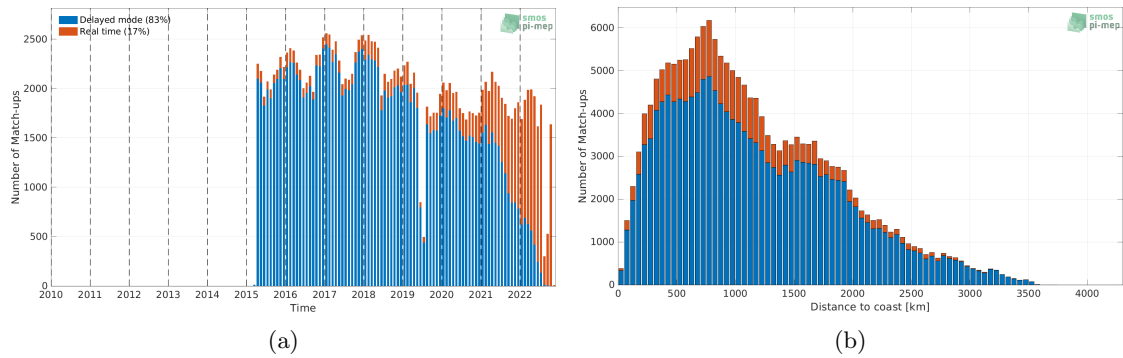
Figure 1: Number of match-ups between Argo and SMAP SSS L2 v5.0 (JPL) SSS as a function of time (a) and as function of the distance to coast (b) over the Roaring Forties and Furious Fifties Pi-MEP region and for the full satellite product period.
