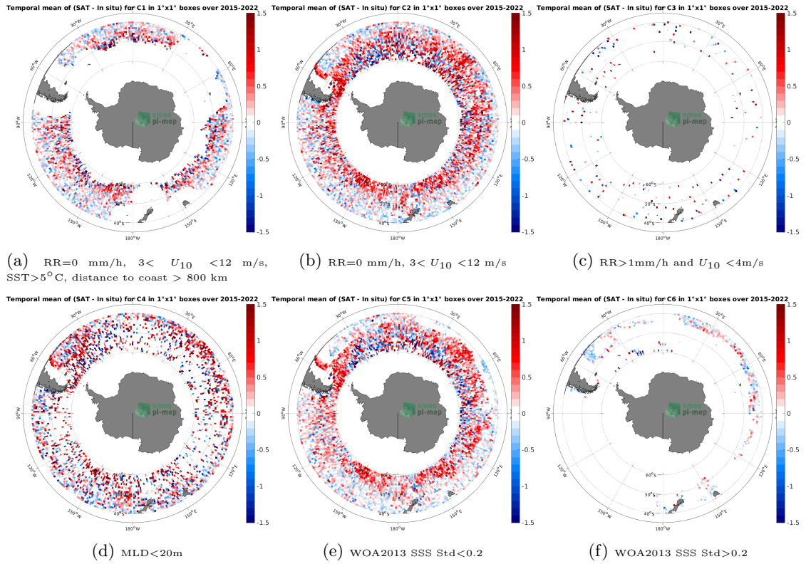
Figure 12: Temporal mean gridded over spatial boxes of size 1^{\circ}\times 1^{\circ} of \Delta\text{SSS} (SMAP SSS L2 v5.0 (JPL) - Argo) for 6 different subdatasets corresponding to:RR=0 mm/h, 3 < U_{10} < 12 m/s, SST > 5^{\circ}\text{C} , distance to coast > 800 km (a), RR=0 mm/h, 3 < U_{10} < 12 m/s (b), RR > 1\text{mm/h} and U_{10} < 4\text{m/s} (c),MLD < 20\text{m} (d),WOA2013 SSS Std < 0.2 (e),WOA2013 SSS Std > 0.2 (f).
