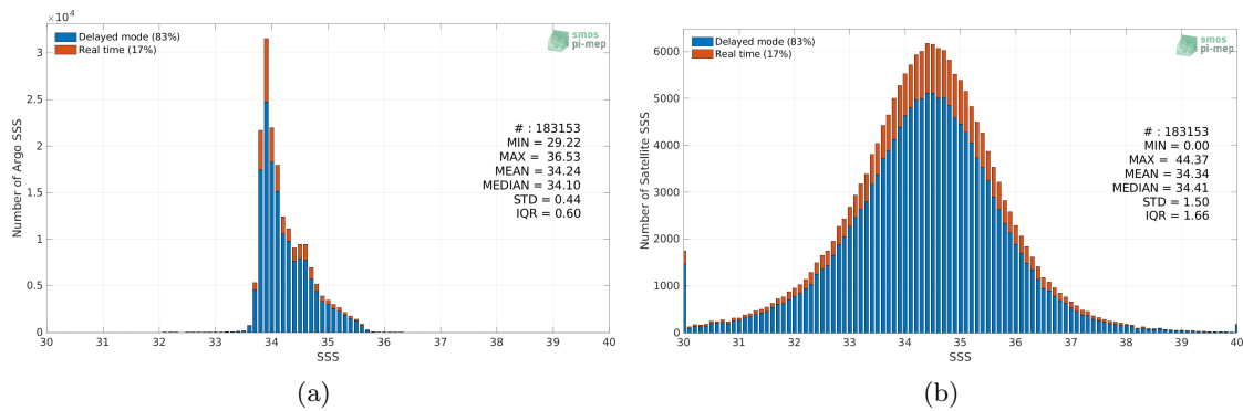
Figure 2: Histograms of SSS from Argo (a) and SMAP SSS L2 v5.0 (JPL) (b) considering all match-up pairs per bins of 0.1 over the Roaring Forties and Furious Fifties Pi-MEP region and for the full satellite product period.
