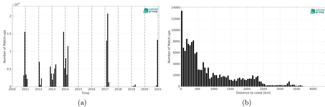
Figure 2: Number of match-ups between TSG (GOSUD-Sailing-ship) and ISAS SSS as a function of time (a) and as function of the distance to coast (b) over the Roaring Forties and Furious Fifties Pi-MEP region and for the full satellite product period.
