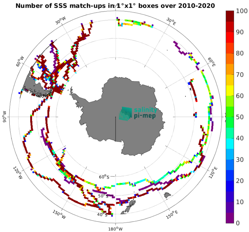
Figure 5: Number of SSS match-ups between TSG (GOSUD-Sailing-ship) SSS and the ISAS SSS product for the Roaring Forties and Furious Fifties Pi-MEP region over 1^\circ \times 1^\circ boxes and for the full satellite product period.
