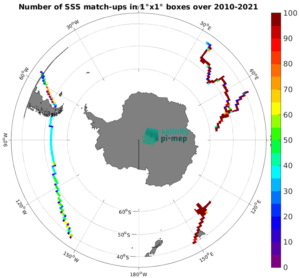
Figure 5: Number of SSS match-ups between TSG (GOSUD-Research-vessel) SSS and the ISAS SSS product for the Roaring Forties and Furious Fifties Pi-MEP region over 1^{\circ}\times 1^{\circ} boxes and for the full satellite product period.
