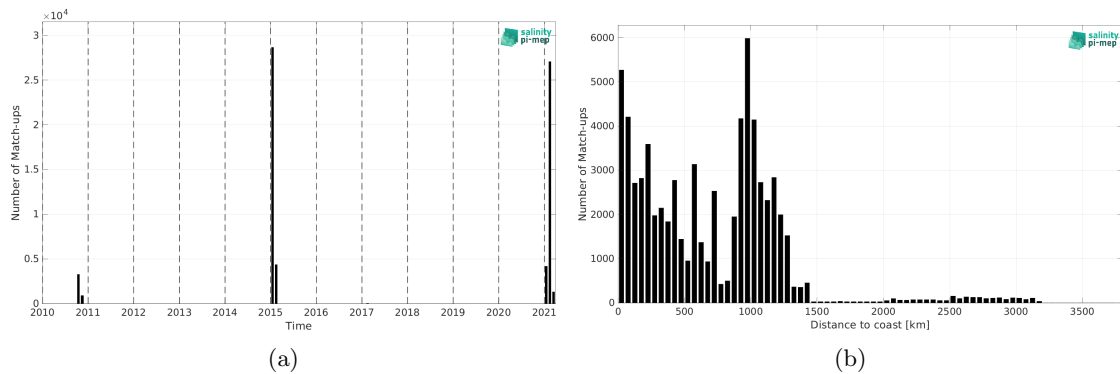
Figure 2: Number of match-ups between TSG (GOSUD-Research-vessel) and ISAS SSS as a function of time (a) and as function of the distance to coast (b) over the Roaring Forties and Furious Fifties Pi-MEP region and for the full satellite product period.
