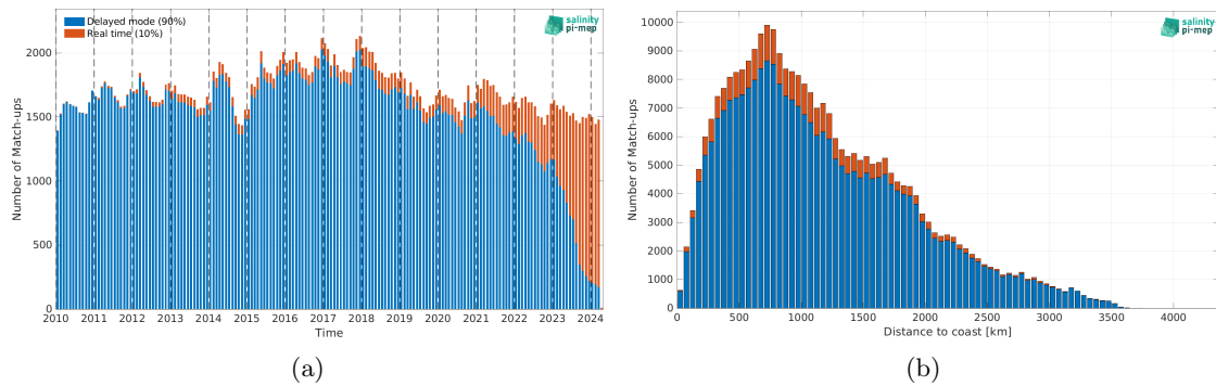
Figure 2: Number of match-ups between Argo and ISAS SSS as a function of time (a) and as function of the distance to coast (b) over the Roaring Forties and Furious Fifties Pi-MEP region and for the full satellite product period.
