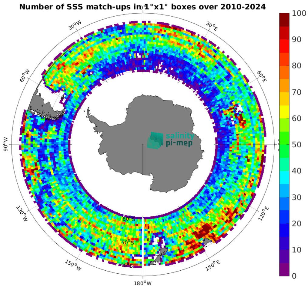
Figure 5: Number of SSS match-ups between Argo SSS and the ISAS SSS product for the Roaring Forties and Furious Fifties Pi-MEP region over 1^\circ \times 1^\circ boxes and for the full satellite product period.
