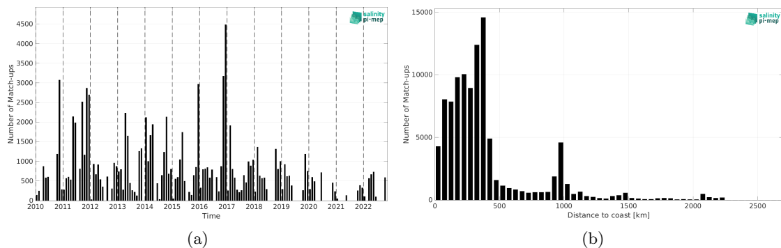
Figure 2: Number of match-ups between TSG (SAMOS) and CCI SSS L4 POLAR SH Merged-OI v4.41 - 7-day running (ESA) SSS as a function of time (a) and as function of the distance to coast (b) over the Roaring Forties and Furious Fifties Pi-MEP region and for the full satellite product period.
