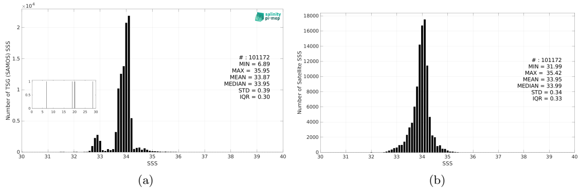
Figure 3: Histograms of SSS from TSG (SAMOS) (a) and CCI SSS L4 POLAR SH Merged-OI v4.41 - 7-day running (ESA) (b) considering all match-up pairs per bins of 0.1 over the Roaring Forties and Furious Fifties Pi-MEP region and for the full satellite product period.
