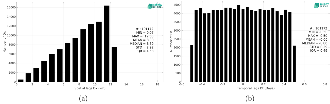
Figure 6: Histograms of the spatial (a) and temporal (b) lags between the location/time of the TSG (SAMOS) measurement and the date of the corresponding CCI SSS L4 POLAR SH Merged-OI v4.41 - 7-day running (ESA) SSS pixel.
