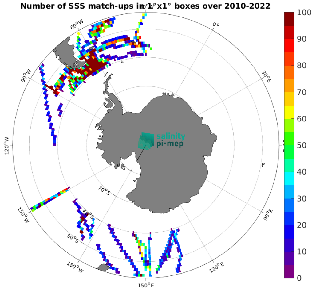
Figure 5: Number of SSS match-ups between TSG (SAMOS) SSS and the CCI SSS L4 POLAR SH Merged-OI v4.41 - 7-day running (ESA) SSS product for the Roaring Forties and Furious Fifties Pi-MEP region over 1^\circ \times 1^\circ boxes and for the full satellite product period.
