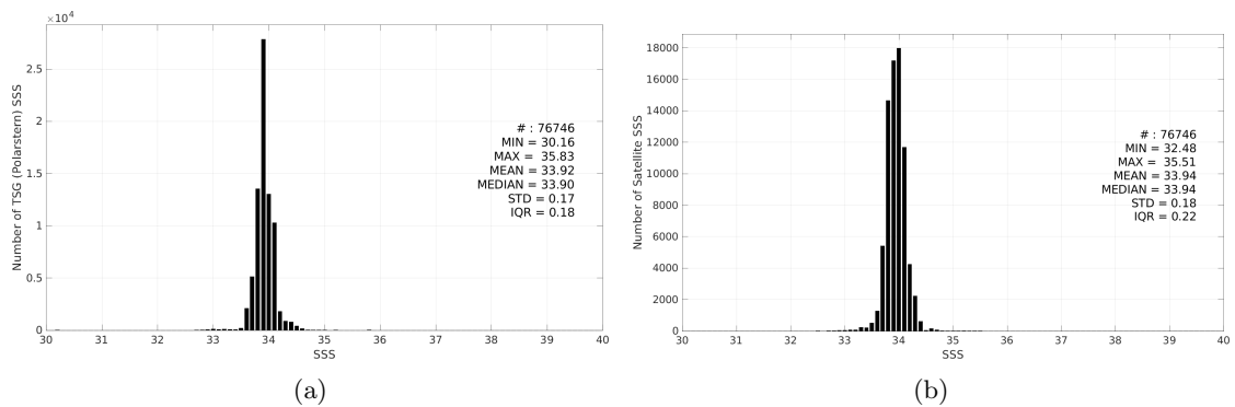
Figure 3: Histograms of SSS from TSG (Polarstern) (a) and CCI SSS L4 POLAR SH Merged-OI v4.41 - 7-day running (ESA) (b) considering all match-up pairs per bins of 0.1 over the Roaring Forties and Furious Fifties Pi-MEP region and for the full satellite product period.
