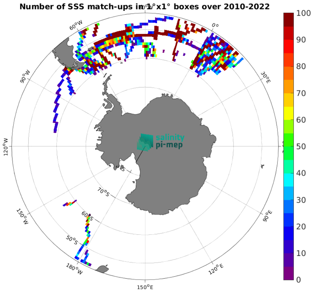
Figure 5: Number of SSS match-ups between TSG (Polarstern) SSS and the CCI SSS L4 POLAR SH Merged-OI v4.41 - 7-day running (ESA) SSS product for the Roaring Forties and Furious Fifties Pi-MEP region over 1^\circ \times 1^\circ boxes and for the full satellite product period.
