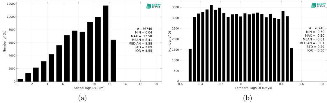
Figure 6: Histograms of the spatial (a) and temporal (b) lags between the location/time of the TSG (Polarstern) measurement and the date of the corresponding CCI SSS L4 POLAR SH Merged-OI v4.41 - 7-day running (ESA) SSS pixel.
