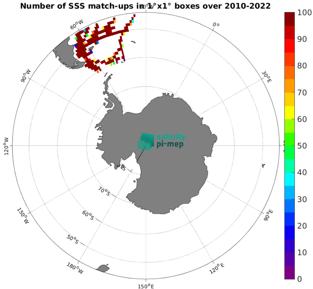
Figure 5: Number of SSS match-ups between TSG (CSIC-UTM) SSS and the CCI SSS L4 POLAR SH Merged-OI v4.41 - 7-day running (ESA) SSS product for the Roaring Forties and Furious Fifties Pi-MEP region over 1^\circ \times 1^\circ boxes and for the full satellite product period.
