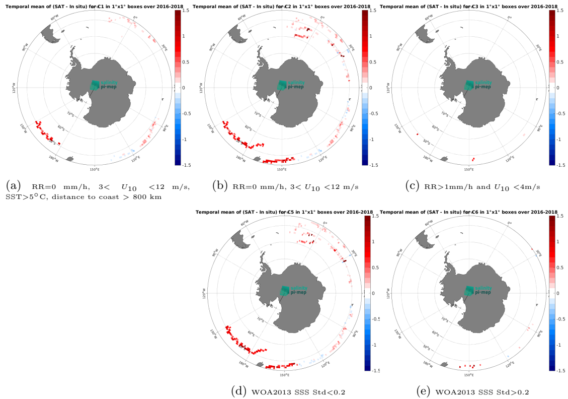
Figure 13: Temporal mean gridded over spatial boxes of size 1^\circ \times 1^\circ of \Delta\text{SSS} (CCI SSS L4 POLAR SH Merged-OI v4.41 - 7-day running (ESA) - Surface drifters) for 5 different subdatasets corresponding to:RR=0 mm/h, 3 < U_{10} < 12 m/s, SST >5^\circ\text{C} , distance to coast > 800 km (a), RR=0 mm/h, 3 < U_{10} < 12 m/s (b), RR >1 mm/h and U_{10} < 4 m/s (c), WOA2013 SSS Std <0.2 (d), WOA2013 SSS Std >0.2 (e).
