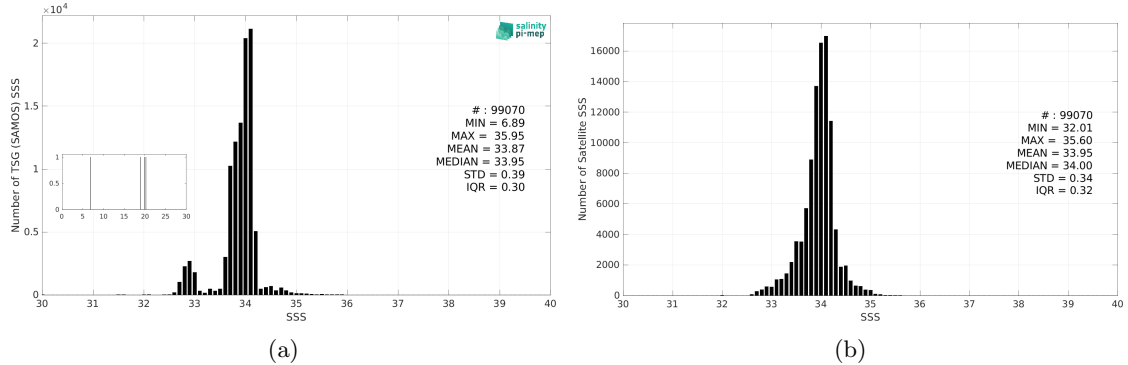
Figure 3: Histograms of SSS from TSG (SAMOS) (a) and CCI SSS L4 POLAR SH Merged-OI v4.41 - 30-day running (ESA) (b) considering all match-up pairs per bins of 0.1 over the Roaring Forties and Furious Fifties Pi-MEP region and for the full satellite product period.
