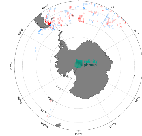
(e) MEAN( \Delta SSS) (Satellite - TSG (Polarstern)) 16
