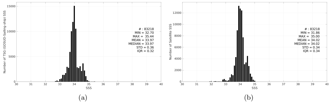
Figure 3: Histograms of SSS from TSG (GOSUD-Sailing-ship) (a) and CCI SSS L4 POLAR SH Merged-OI v4.41 - 30-day running (ESA) (b) considering all match-up pairs per bins of 0.1 over the Roaring Forties and Furious Fifties Pi-MEP region and for the full satellite product period.
