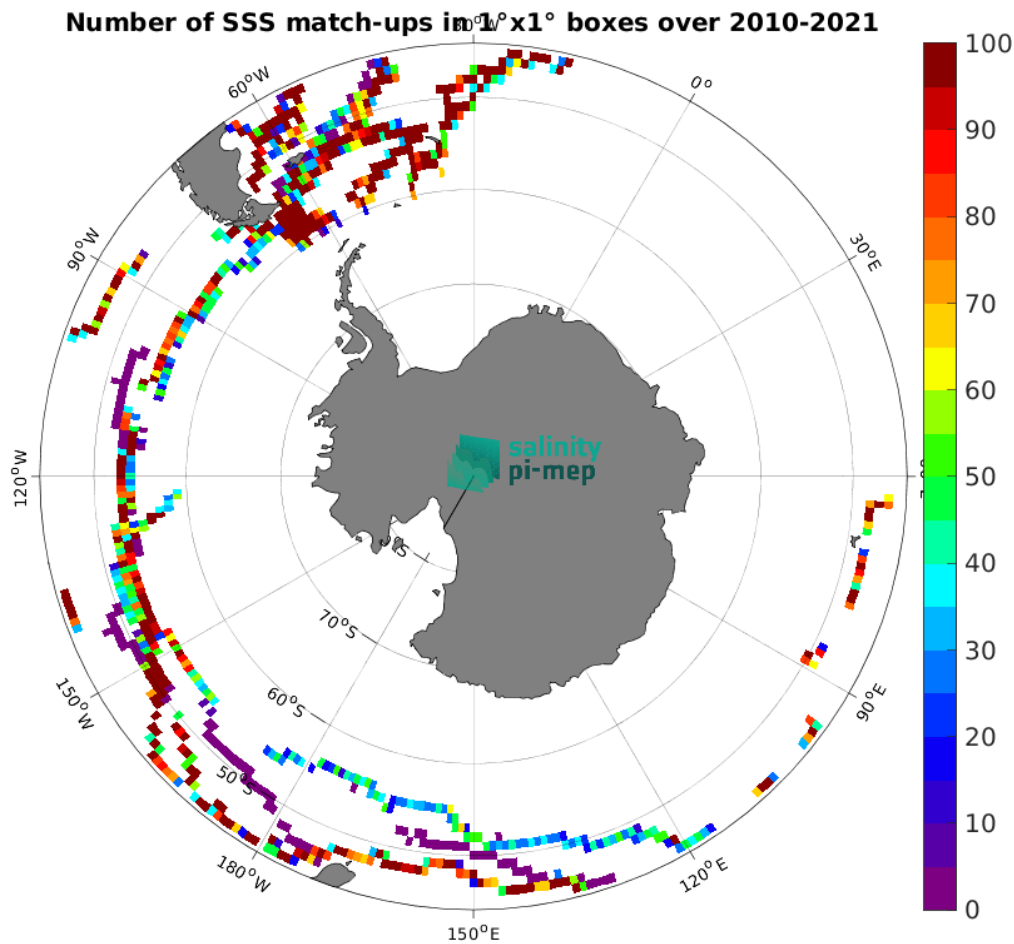
Figure 5: Number of SSS match-ups between TSG (GOSUD-Sailing-ship) SSS and the CCI SSS L4 POLAR SH Merged-OI v4.41 - 30-day running (ESA) SSS product for the Roaring Forties and Furious Fifties Pi-MEP region over 1^\circ \times 1^\circ boxes and for the full satellite product period.
