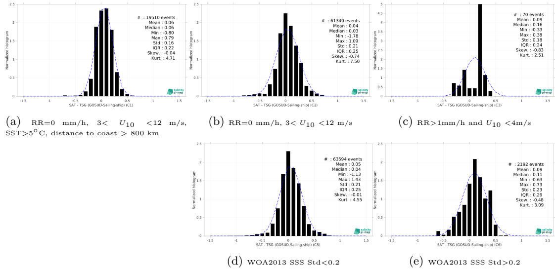
Figure 15: Normalized histogram of \Delta SSS (CCI SSS L4 POLAR SH Merged-OI v4.41 - 30-day running (ESA) - TSG (GOSUD-Sailing-ship)) for 5 different subdatasets corresponding to: RR=0 mm/h, 3 < U_{10} < 12 m/s, SST>5°C, distance to coast > 800 km (a), RR=0 mm/h, 3 < U_{10} < 12 m/s (b), RR>1mm/h and U_{10} < 4 m/s (c), WOA2013 SSS Std<0.2 (d), WOA2013 SSS Std>0.2 (e).
