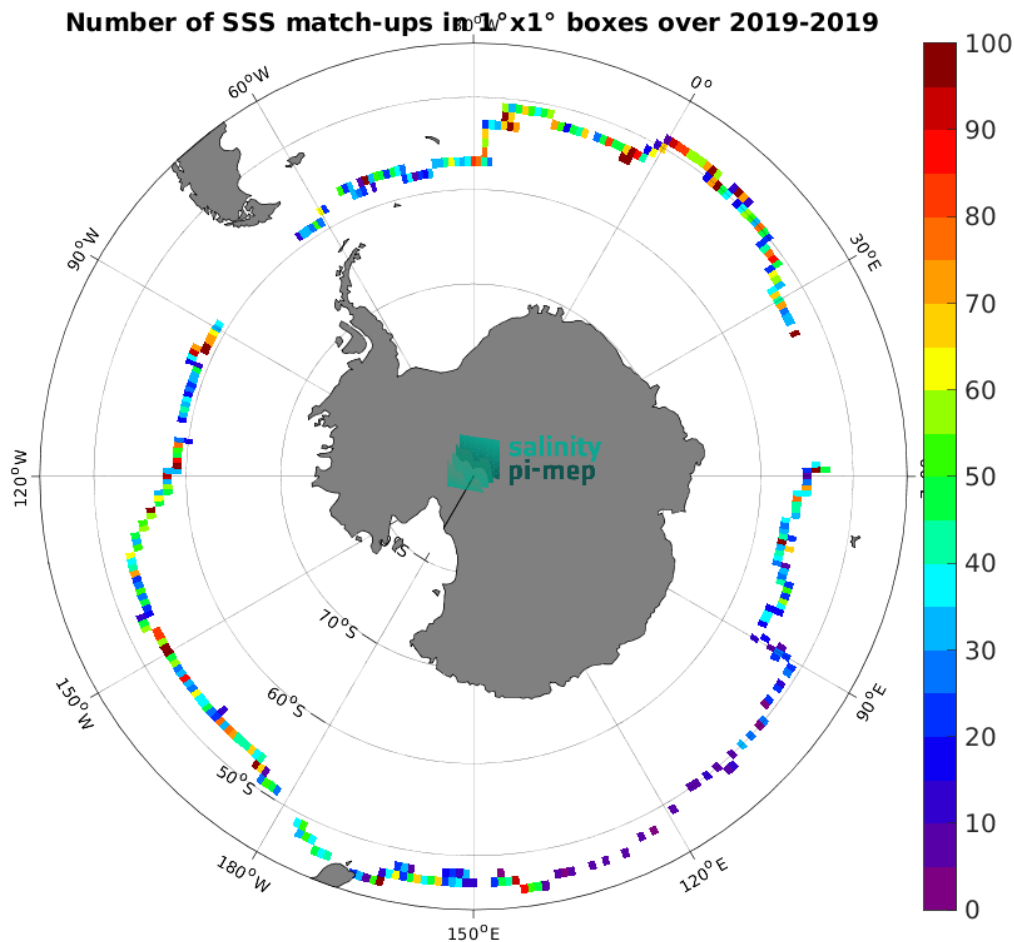
Figure 5: Number of SSS match-ups between Saildrone SSS and the CCI SSS L4 POLAR SH Merged-OI v4.41 - 30-day running (ESA) SSS product for the Roaring Forties and Furious Fifties Pi-MEP region over 1^\circ \times 1^\circ boxes and for the full satellite product period.
