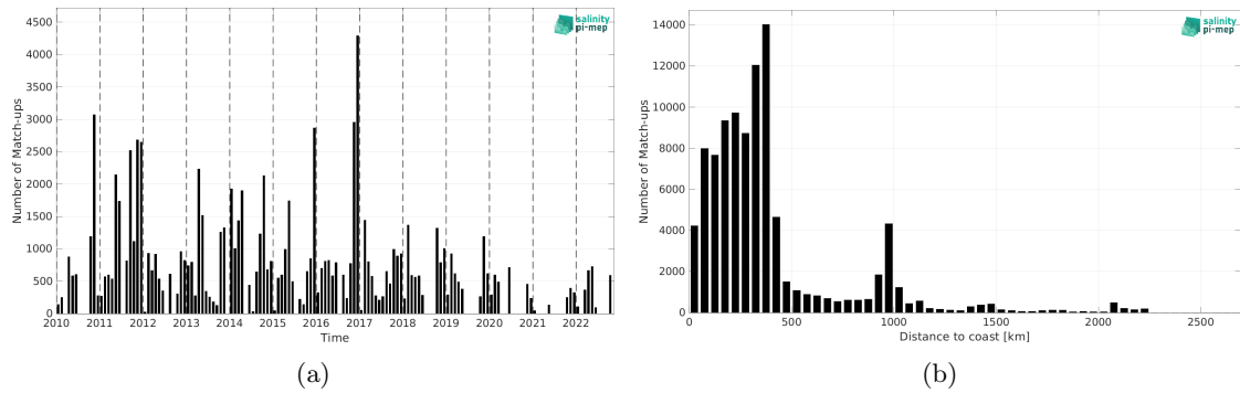
Figure 1: Number of match-ups between TSG (SAMOS) and CCI SSS L4 POLAR SH Merged-OI v4.4 - 7-day running (ESA) SSS as a function of time (a) and as function of the distance to coast (b) over the Roaring Forties and Furious Fifties Pi-MEP region and for the full satellite product period.
