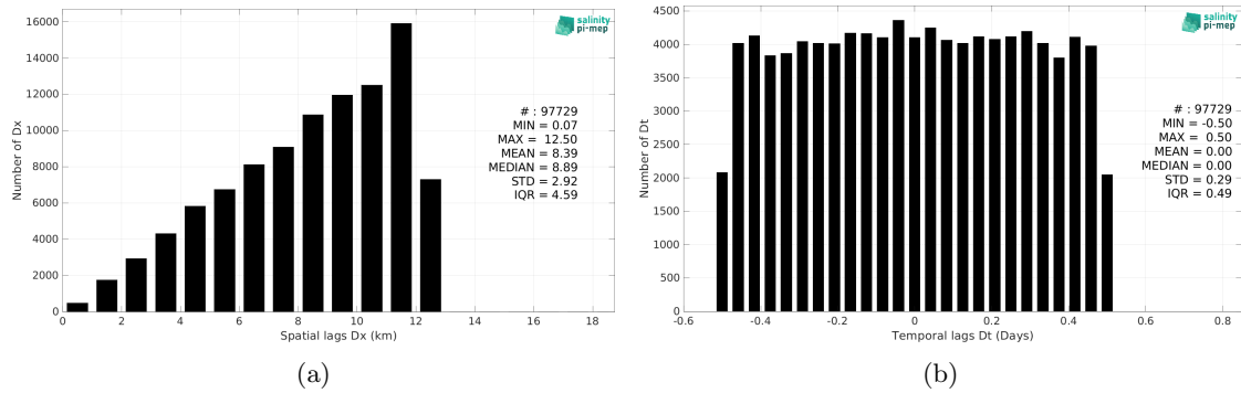
Figure 5: Histograms of the spatial (a) and temporal (b) lags between the location/time of the TSG (SAMOS) measurement and the date of the corresponding CCI SSS L4 POLAR SH Merged-OI v4.4 - 7-day running (ESA) SSS pixel.
