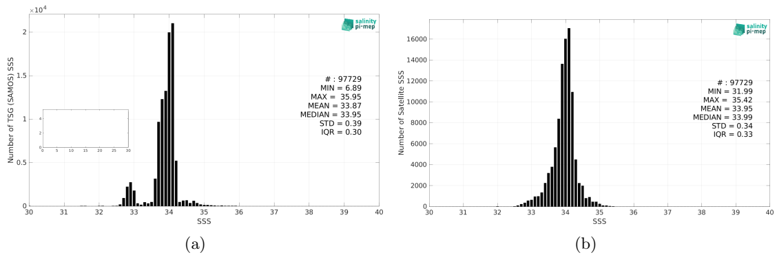
Figure 2: Histograms of SSS from TSG (SAMOS) (a) and CCI SSS L4 POLAR SH Merged-OI v4.4 - 7-day running (ESA) (b) considering all match-up pairs per bins of 0.1 over the Roaring Forties and Furious Fifties Pi-MEP region and for the full satellite product period.
