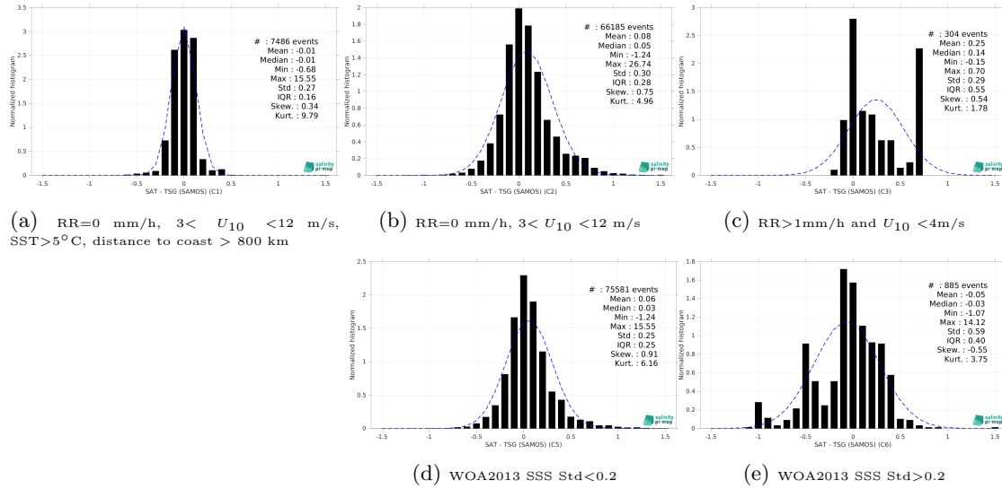
Figure 13: Normalized histogram of \Delta SSS (CCI SSS L4 POLAR SH Merged-OI v4.4 - 7-day running (ESA) - TSG (SAMOS)) for 5 different subdatasets corresponding to: RR=0 mm/h, 3 < U_{10} < 12 m/s, SST>5°C, distance to coast > 800 km (a), RR=0 mm/h, 3 < U_{10} < 12 m/s (b), RR>1mm/h and U_{10} < 4 m/s (c), WOA2013 SSS Std<0.2 (d), WOA2013 SSS Std>0.2 (e).
