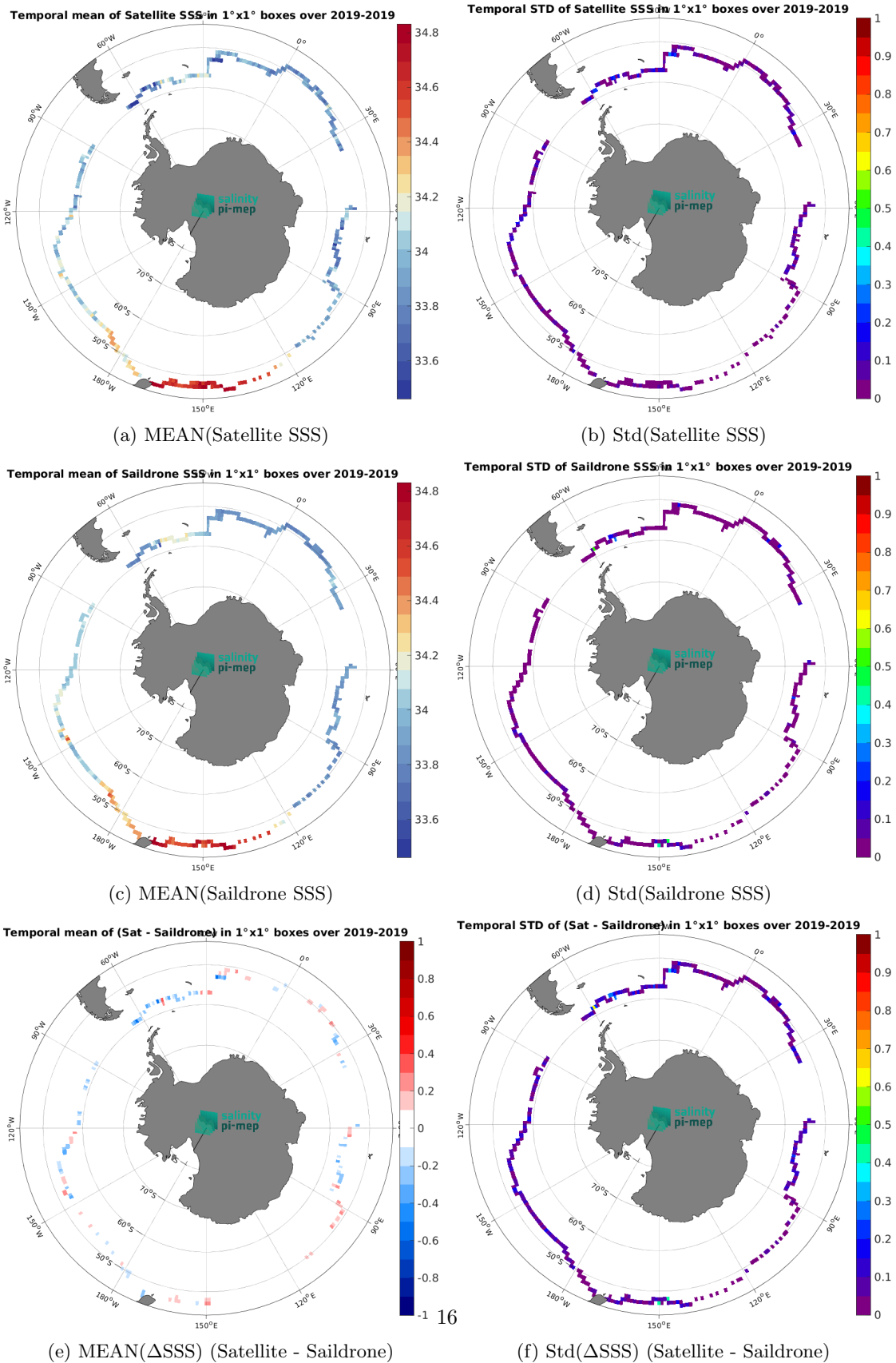
Figure 6: Temporal mean (left) and Std (right) of SSS from CCI SSS L4 POLAR SH Merged-OI v4.4 - 7-day running (ESA) (top), Saildrone (middle), and of \Delta SSS (Satellite - Saildrone). Only match-up pairs are used to generate these maps.
