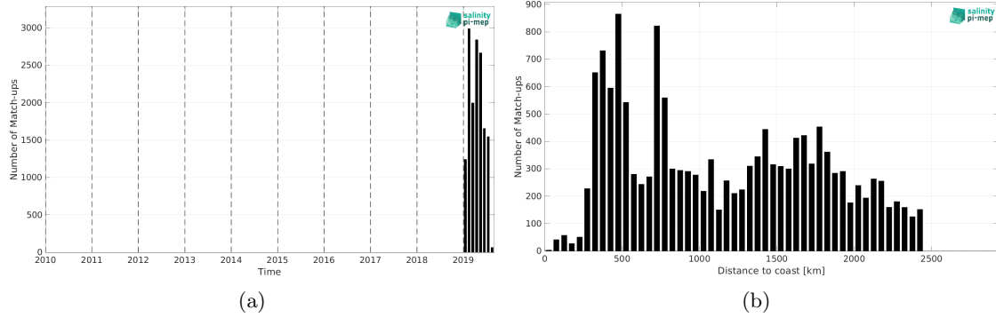
Figure 1: Number of match-ups between Saildrone and CCI SSS L4 POLAR SH Merged-OI v4.4 - 7-day running (ESA) SSS as a function of time (a) and as function of the distance to coast (b) over the Roaring Forties and Furious Fifties Pi-MEP region and for the full satellite product period.
