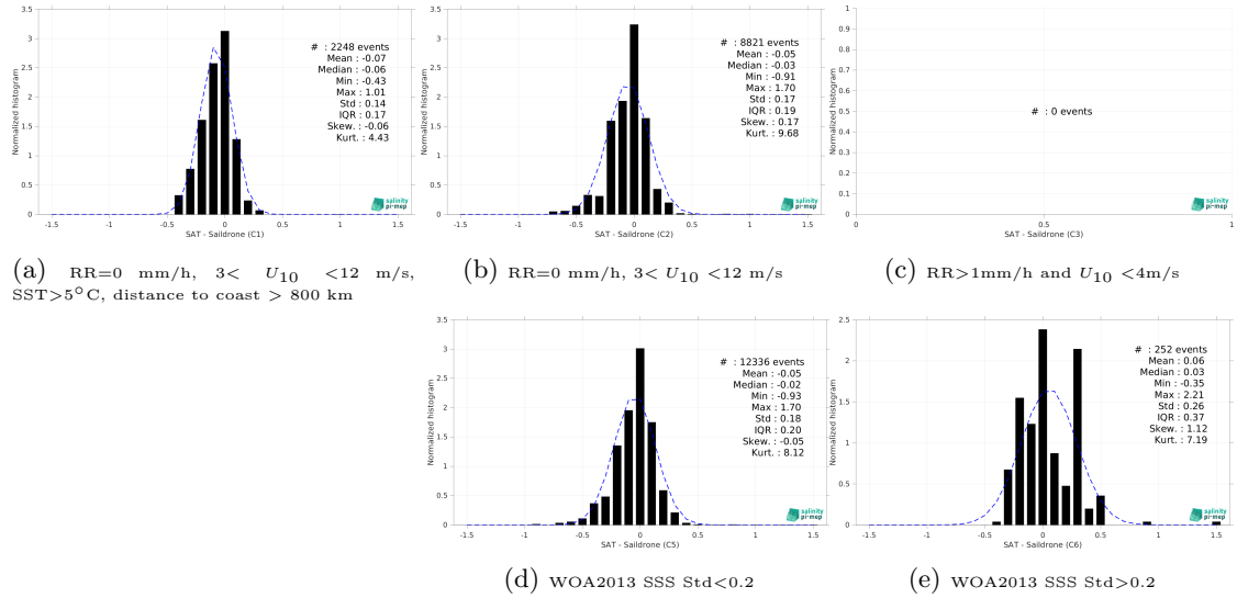
Figure 13: Normalized histogram of \Delta SSS (CCI SSS L4 POLAR SH Merged-OI v4.4 - 7-day running (ESA) - Saildrone) for 5 different subdatasets corresponding to: RR=0 mm/h, 3 < U_{10} < 12 m/s, SST > 5°C, distance to coast > 800 km (a), RR=0 mm/h, 3 < U_{10} < 12 m/s (b), RR > 1mm/h and U_{10} < 4 m/s (c), WOA2013 SSS Std < 0.2 (d), WOA2013 SSS Std > 0.2 (e).
