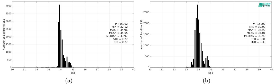
Figure 2: Histograms of SSS from Saildrone (a) and CCI SSS L4 POLAR SH Merged-OI v4.4 - 7-day running (ESA) (b) considering all match-up pairs per bins of 0.1 over the Roaring Forties and Furious Fifties Pi-MEP region and for the full satellite product period.
