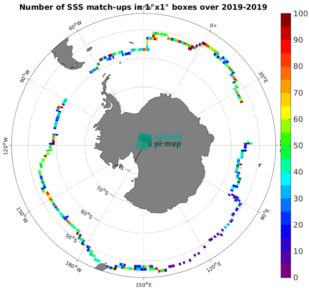
Figure 4: Number of SSS match-ups between Saildrone SSS and the CCI SSS L4 POLAR SH Merged-OI v4.4 - 7-day running (ESA) SSS product for the Roaring Forties and Furious Fifties Pi-MEP region over 1^\circ \times 1^\circ boxes and for the full satellite product period.
