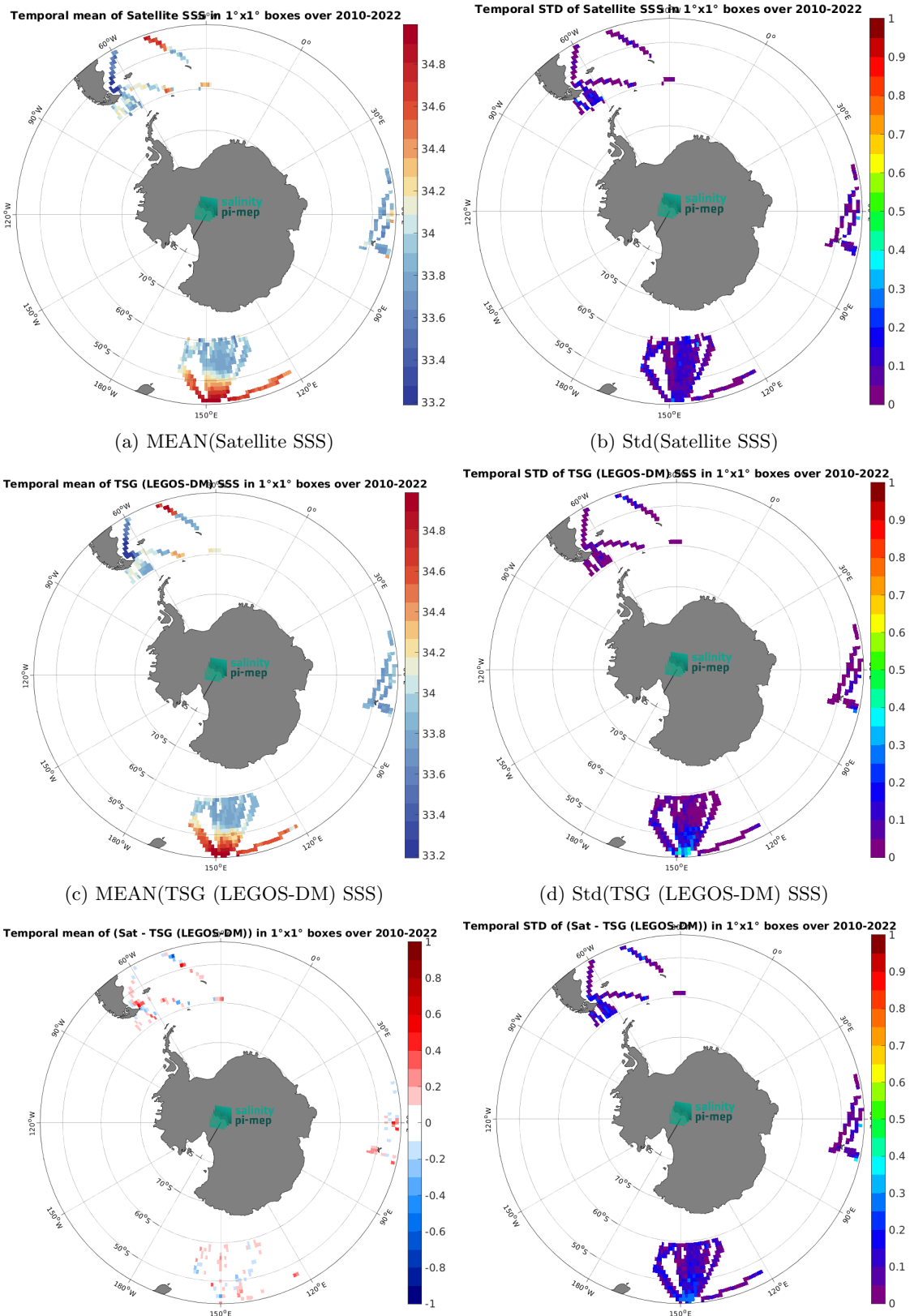
Figure 6: Temporal mean (left) and Std (right) of SSS from CCI SSS L4 POLAR SH Merged-OI v4.4 - 30-day running (ESA) (top), TSG (LEGOS-DM) (middle), and of \Delta SSS (Satellite - TSG (LEGOS-DM)). Only match-up pairs are used to generate these maps.
