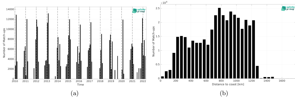
Figure 1: Number of match-ups between TSG (LEGOS-DM) and CCI SSS L4 POLAR SH Merged-OI v4.4 - 30-day running (ESA) SSS as a function of time (a) and as function of the distance to coast (b) over the Roaring Forties and Furious Fifties Pi-MEP region and for the full satellite product period.
