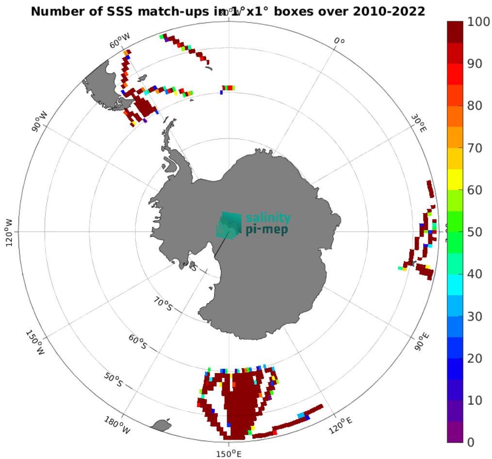
Figure 4: Number of SSS match-ups between TSG (LEGOS-DM) SSS and the CCI SSS L4 POLAR SH Merged-OI v4.4 - 30-day running (ESA) SSS product for the Roaring Forties and Furious Fifties Pi-MEP region over 1^\circ \times 1^\circ boxes and for the full satellite product period.
