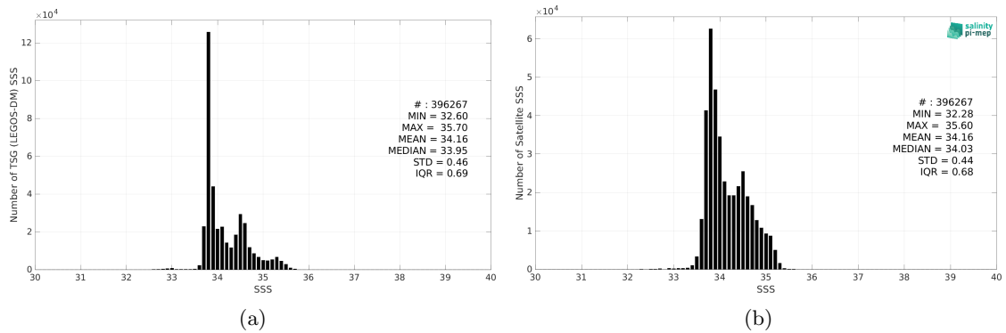
Figure 2: Histograms of SSS from TSG (LEGOS-DM) (a) and CCI SSS L4 POLAR SH Merged-OI v4.4 - 30-day running (ESA) (b) considering all match-up pairs per bins of 0.1 over the Roaring Forties and Furious Fifties Pi-MEP region and for the full satellite product period.
