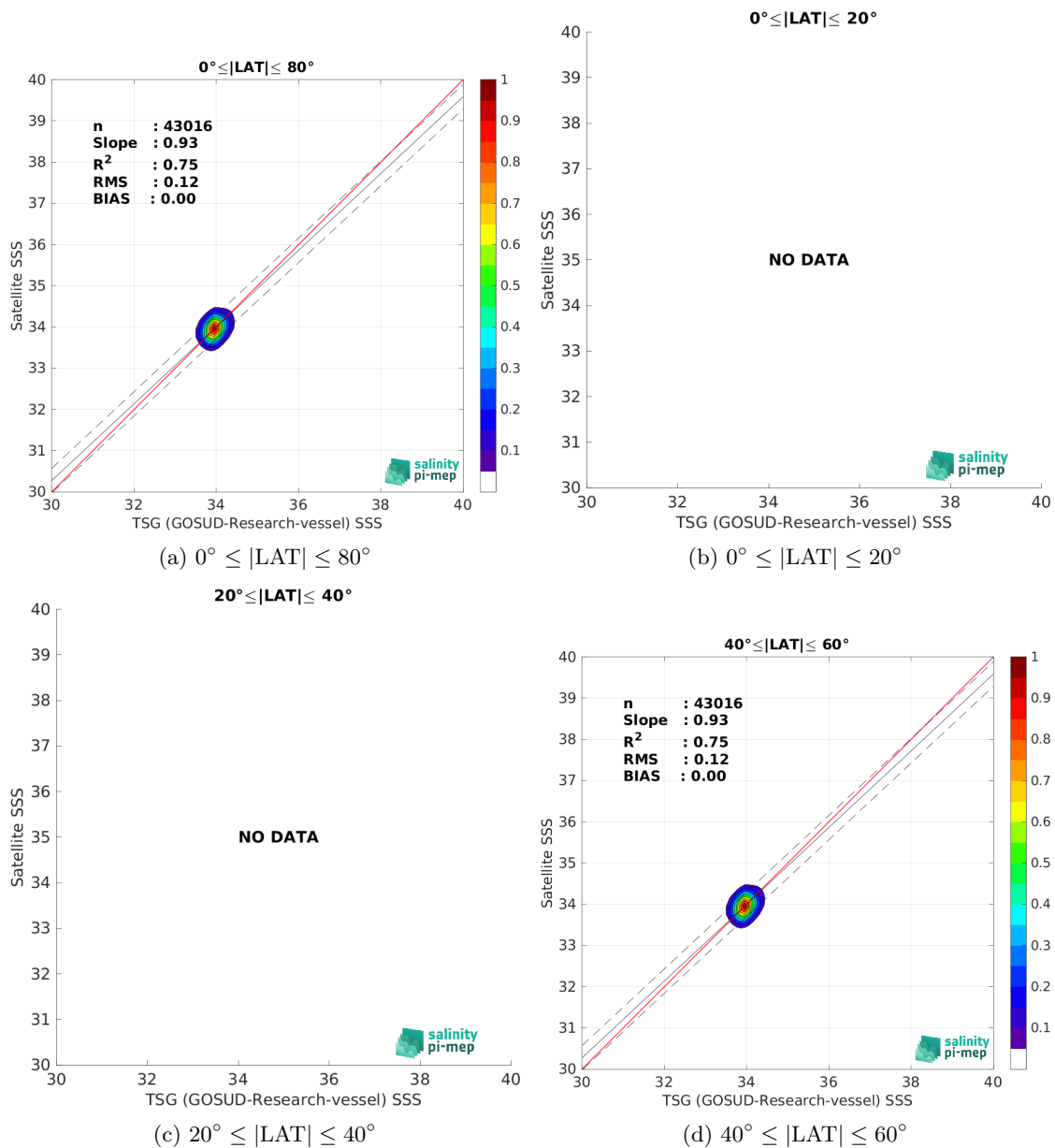
Figure 9: Contour maps of the concentration of CCI SSS L4 POLAR SH Merged-OI v4.4 - 30-day running (ESA) SSS (y-axis) versus TSG (GOSUD-Research-vessel) SSS (x-axis) at match-up pairs for different latitude bands. For each plot, the red line shows x=y . The black thin and dashed lines indicate a linear fit through the data cloud and the \pm 95\% confidence levels, respectively. The number match-up pairs n , the slope and R^2 coefficient of the linear fit, the root mean square (RMS) and the mean bias between satellite and in situ data are indicated for each latitude band in each plots.
