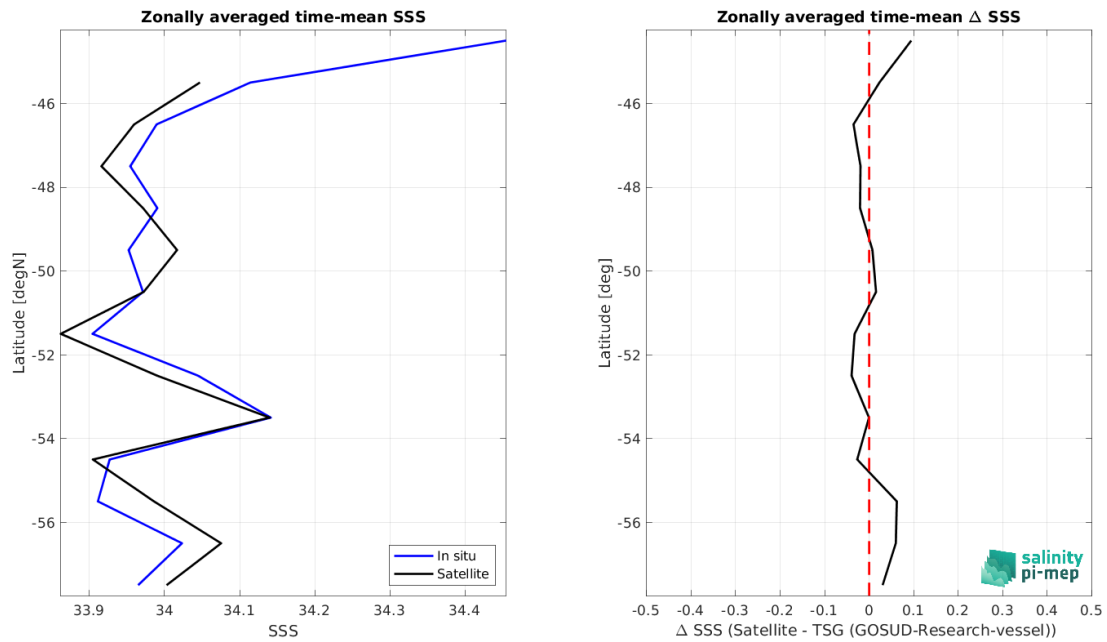
Figure 8: Left panel: Zonal mean SSS from CCI SSS L4 POLAR SH Merged-OI v4.4 - 30-day running (ESA) satellite product (black) and from TSG (GOSUD-Research-vessel) (blue). Right panel: Zonal mean of \Delta SSS (Satellite - TSG (GOSUD-Research-vessel)) for all the collected Pi-MEP match-up pairs estimated over the full satellite product period.
