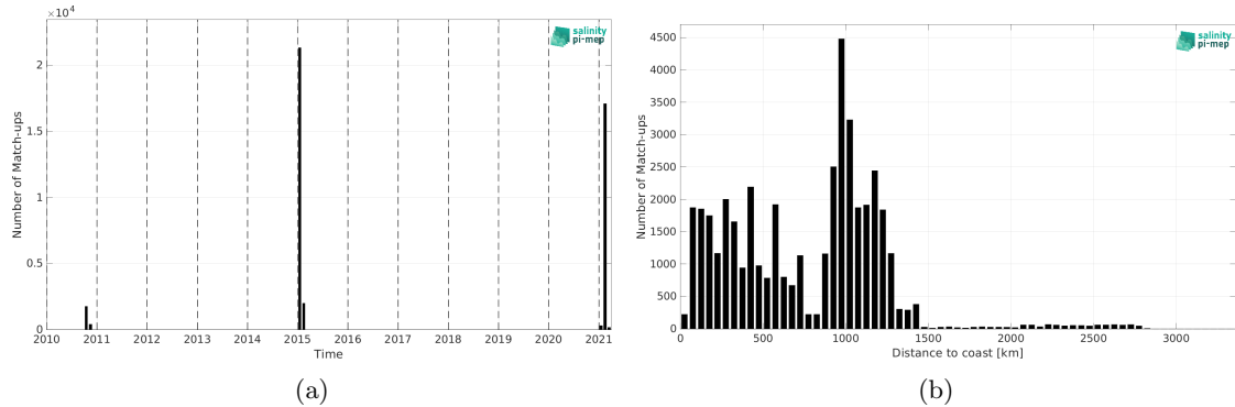
Figure 1: Number of match-ups between TSG (GOSUD-Research-vessel) and CCI SSS L4 POLAR SH Merged-OI v4.4 - 30-day running (ESA) SSS as a function of time (a) and as function of the distance to coast (b) over the Roaring Forties and Furious Fifties Pi-MEP region and for the full satellite product period.
