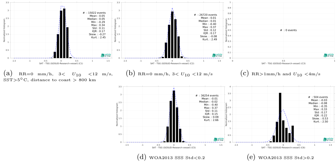
Figure 13: Normalized histogram of \Delta SSS (CCI SSS L4 POLAR SH Merged-OI v4.4 - 30-day running (ESA) - TSG (GOSUD-Research-vessel)) for 5 different subdatasets corresponding to: RR=0 mm/h, 3 < U_{10} < 12 m/s, SST>5°C, distance to coast > 800 km (a), RR=0 mm/h, 3 < U_{10} < 12 m/s (b), RR>1mm/h and U_{10} < 4 m/s (c), WOA2013 SSS Std<0.2 (d), WOA2013 SSS Std>0.2 (e).
