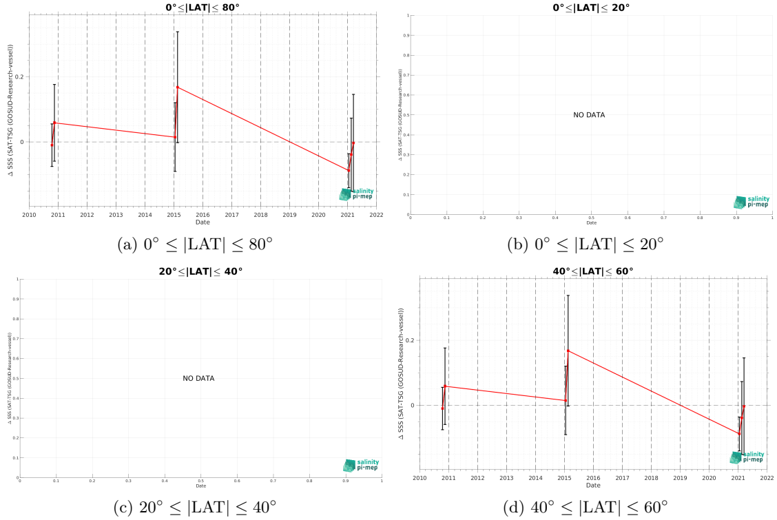
Figure 10: Monthly median (red curves) of \Delta SSS (Satellite - in situ ) between CCI SSS L4 POLAR SH Merged-OI v4.4 - 30-day running (ESA) and TSG (GOSUD-Research-vessel) SSS as function of time for all the collected Pi-MEP match-up pairs estimated over the Roaring Forties and Furious Fifties Pi-MEP region and for the full satellite product period are shown for different latitude bands: (a) 80^{\circ}\text{S}-80^{\circ}\text{N} , (b) 20^{\circ}\text{S}-20^{\circ}\text{N} , (c) 40^{\circ}\text{S}-20^{\circ}\text{S} and 20^{\circ}\text{N}-40^{\circ}\text{N} and (d) 60^{\circ}\text{S}-40^{\circ}\text{S} and 40^{\circ}\text{N}-60^{\circ}\text{N} .
