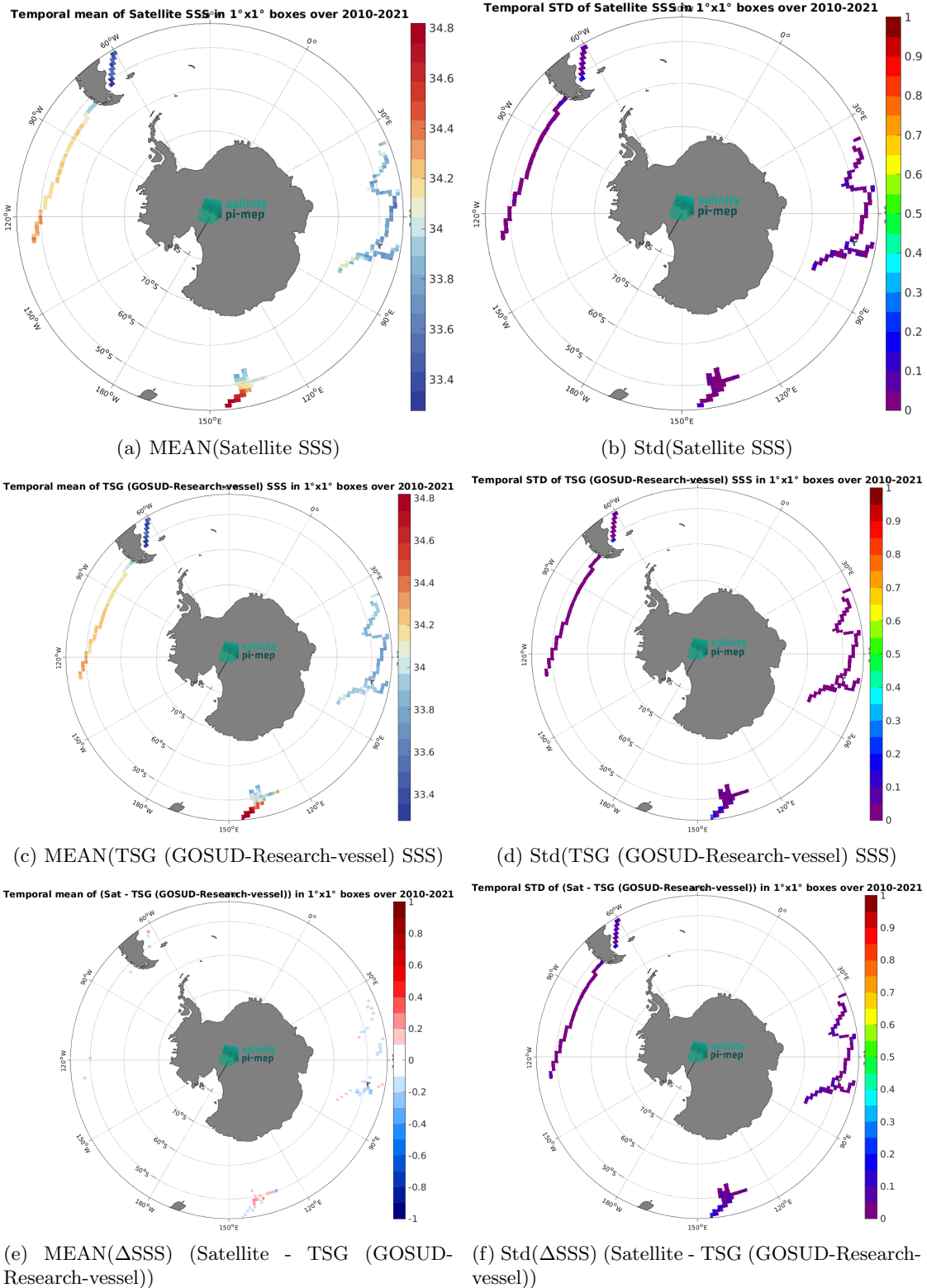
Figure 6: Temporal mean (left) and Std (right) of SSS from CCI SSS L4 POLAR SH Merged-OI v4.4 - 30-day running (ESA) (top), TSG (GOSUD-Research-vessel) (middle), and of \Delta SSS (Satellite - TSG (GOSUD-Research-vessel)). Only match-up pairs are used to generate these maps.
