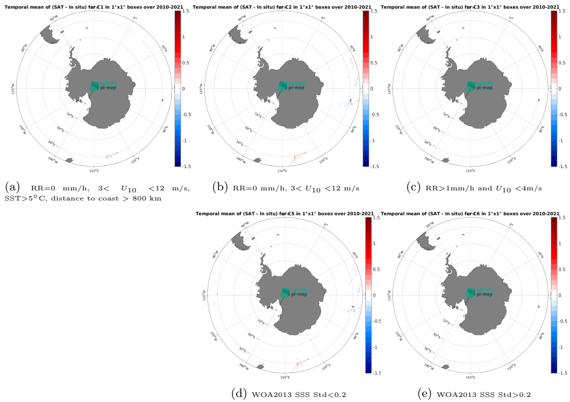
Figure 12: Temporal mean gridded over spatial boxes of size 1°×1° of \Delta SSS (CCI SSS L4 POLAR SH Merged-OI v4.4 - 30-day running (ESA) - TSG (GOSUD-Research-vessel)) for 5 different subdatasets corresponding to:RR=0 mm/h, 3 < U_{10} < 12 m/s, SST>5°C, distance to coast > 800 km (a), RR=0 mm/h, 3 < U_{10} < 12 m/s (b), RR>1mm/h and U_{10} < 4 m/s (c), WOA2013 SSS Std<0.2 (d), WOA2013 SSS Std>0.2 (e).
