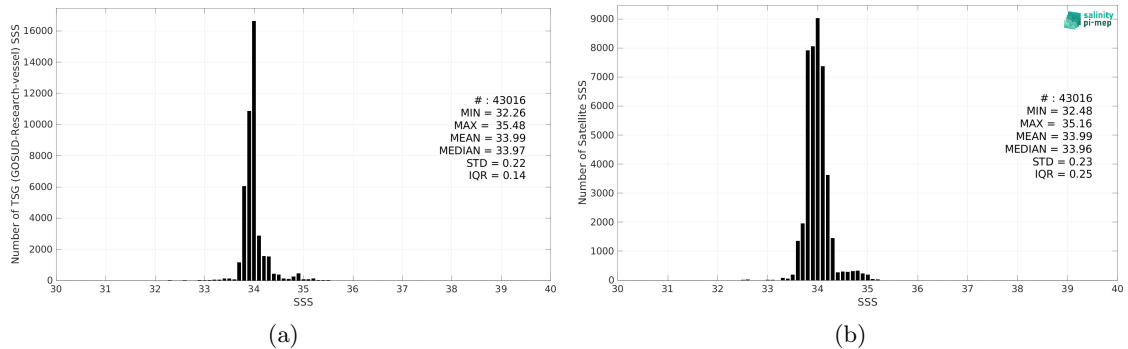
Figure 2: Histograms of SSS from TSG (GOSUD-Research-vessel) (a) and CCI SSS L4 POLAR SH Merged-OI v4.4 - 30-day running (ESA) (b) considering all match-up pairs per bins of 0.1 over the Roaring Forties and Furious Fifties Pi-MEP region and for the full satellite product period.
