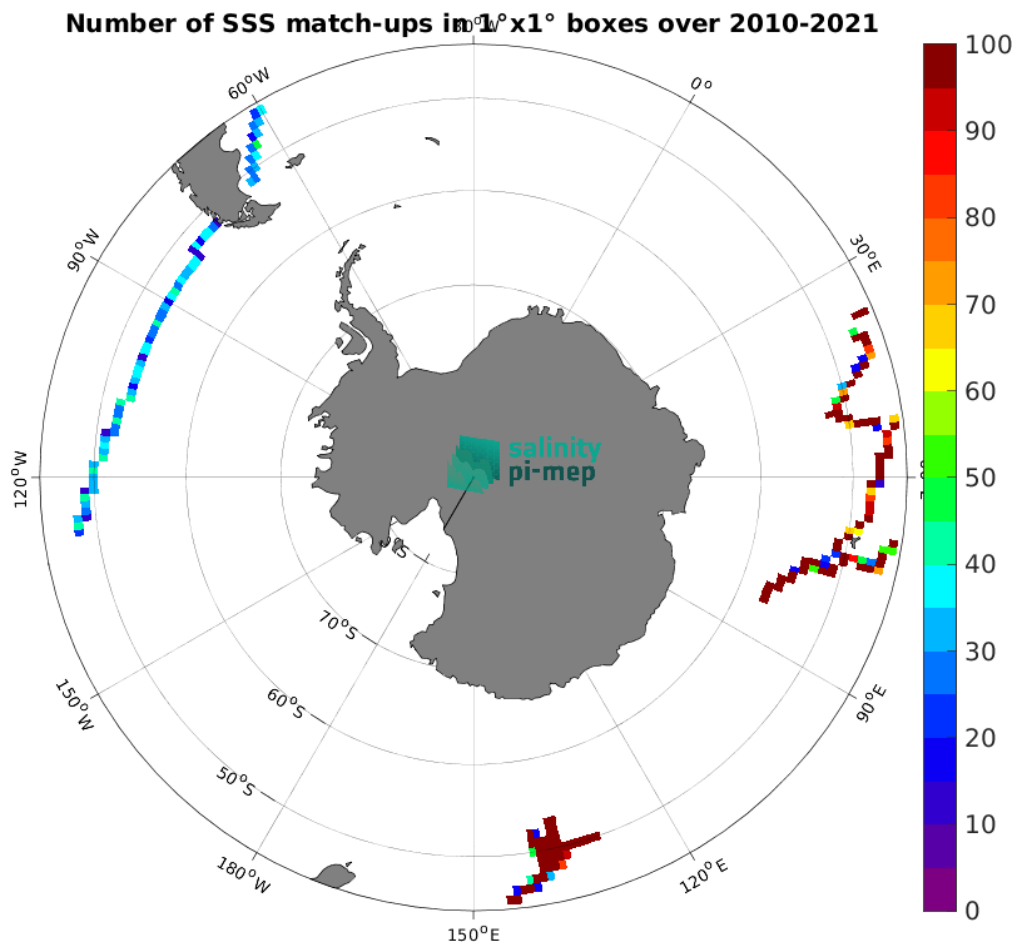
Figure 4: Number of SSS match-ups between TSG (GOSUD-Research-vessel) SSS and the CCI SSS L4 POLAR SH Merged-OI v4.4 - 30-day running (ESA) SSS product for the Roaring Forties and Furious Fifties Pi-MEP region over 1^\circ \times 1^\circ boxes and for the full satellite product period.
