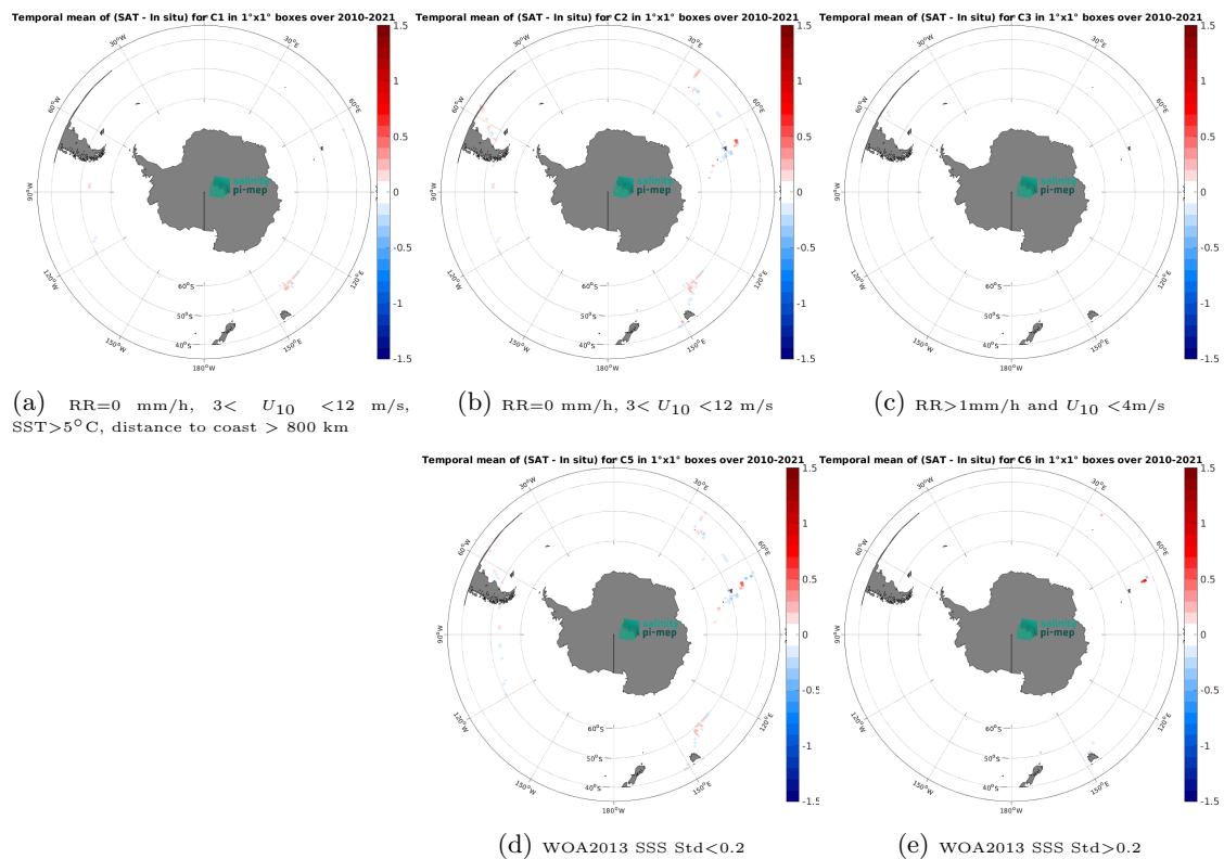
Figure 14: Temporal mean gridded over spatial boxes of size 1^\circ \times 1^\circ of \Delta\text{SSS} (CCI SSS L4 Merged-OI v5.5 - 7-day running (ESA) - TSG (GOSUD-Research-vessel)) for 5 different subdatasets corresponding to: RR=0 mm/h, 3 < U_{10} < 12 m/s, SST > 5°C, distance to coast > 800 km (a), RR=0 mm/h, 3 < U_{10} < 12 m/s (b), RR > 1mm/h and U_{10} < 4 m/s (c), WOA2013 SSS Std < 0.2 (d), WOA2013 SSS Std > 0.2 (e).
