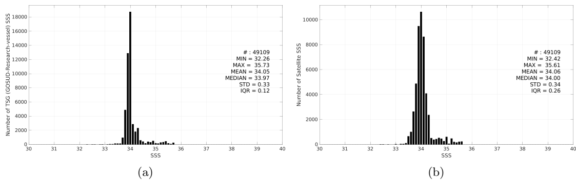
Figure 3: Histograms of SSS from TSG (GOSUD-Research-vessel) (a) and CCI SSS L4 Merged-OI v5.5 - 7-day running (ESA) (b) considering all match-up pairs per bins of 0.1 over the Roaring Forties and Furious Fifties Pi-MEP region and for the full satellite product period.
