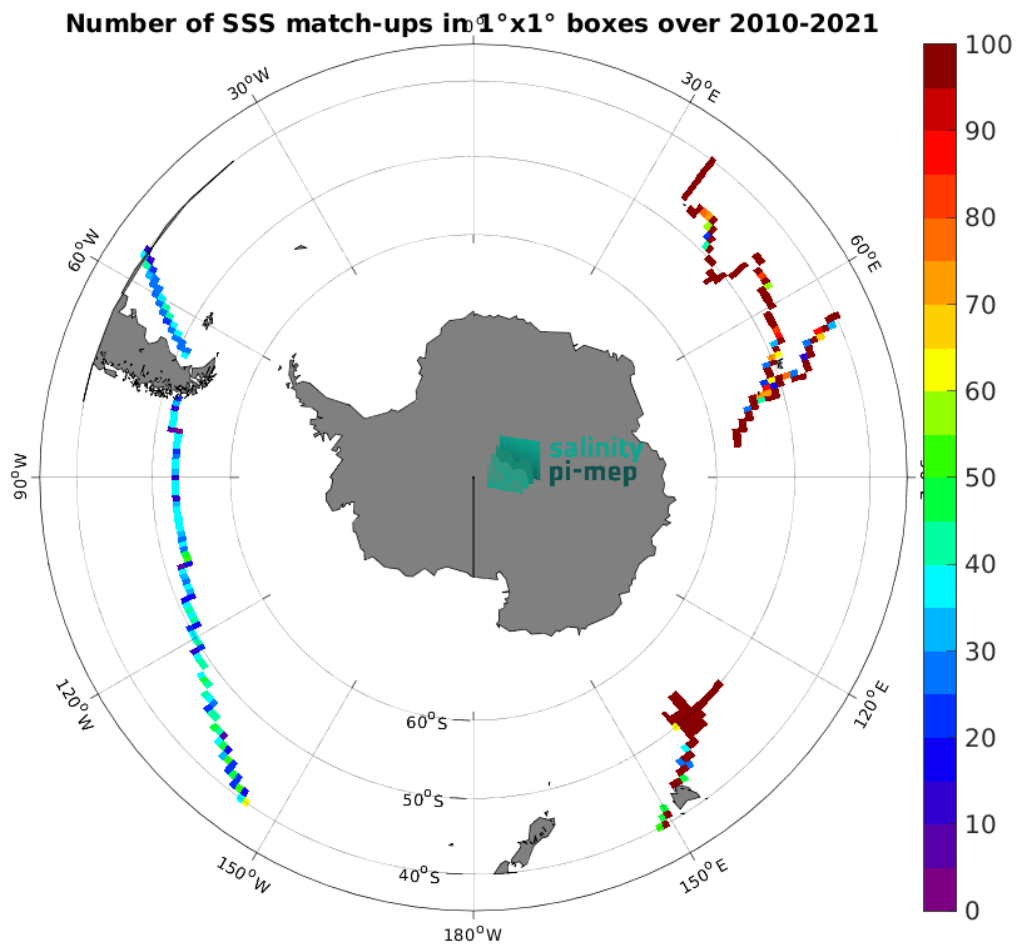
Figure 5: Number of SSS match-ups between TSG (GOSUD-Research-vessel) SSS and the CCI SSS L4 Merged-OI v5.5 - 7-day running (ESA) SSS product for the Roaring Forties and Furious Fifties Pi-MEP region over 1^{\circ} \times 1^{\circ} boxes and for the full satellite product period.
