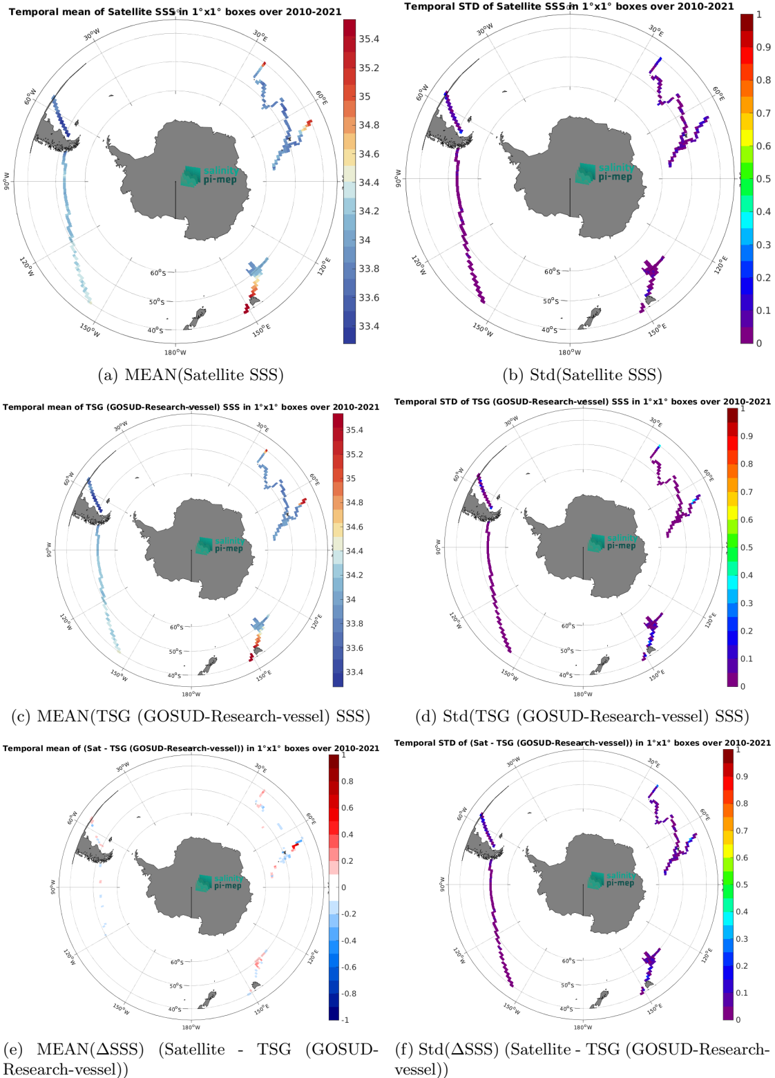
Figure 7: Temporal mean (left) and Std (right) of SSS from CCI SSS L4 Merged-OI v5.5 - 7-day running (ESA) (top), TSG (GOSUD-Research-vessel) (middle), and of \Delta SSS (Satellite - TSG (GOSUD-Research-vessel)). Only match-up pairs are used to generate these maps.
