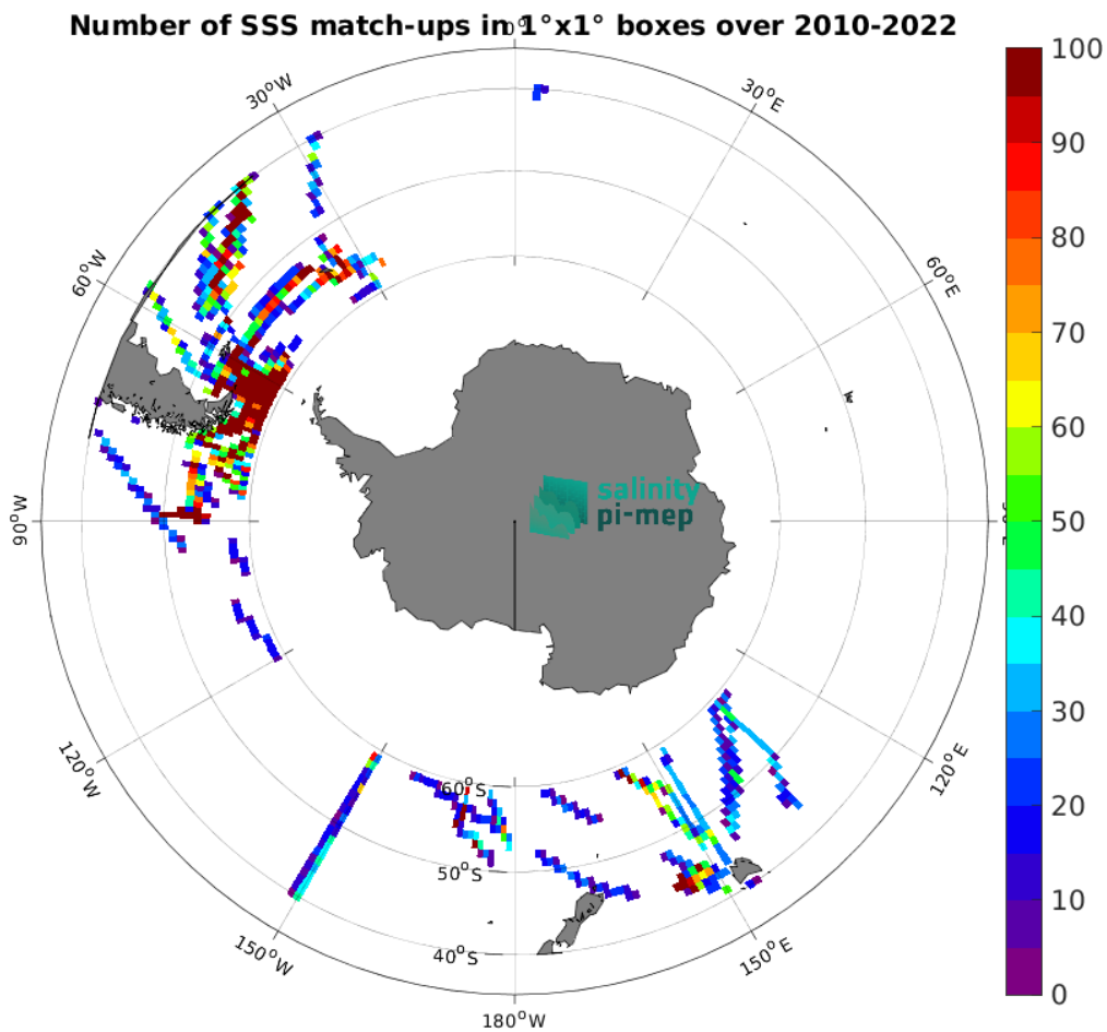
Figure 5: Number of SSS match-ups between TSG (SAMOS) SSS and the CCI SSS L4 Merged-OI v5.5 - 30-day running (ESA) SSS product for the Roaring Forties and Furious Fifties Pi-MEP region over 1^\circ \times 1^\circ boxes and for the full satellite product period.
