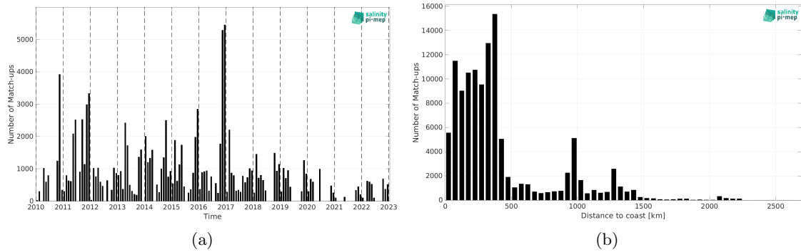
Figure 2: Number of match-ups between TSG (SAMOS) and CCI SSS L4 Merged-OI v5.5 - 30-day running (ESA) SSS as a function of time (a) and as function of the distance to coast (b) over the Roaring Forties and Furious Fifties Pi-MEP region and for the full satellite product period.
