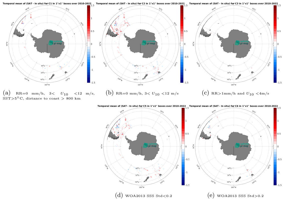
Figure 14: Temporal mean gridded over spatial boxes of size 1^\circ \times 1^\circ of \Delta\text{SSS} (CCI SSS L4 Merged-OI v5.5 - 30-day running (ESA) - TSG (SAMOS)) for 5 different subdatasets corresponding to: RR=0 mm/h, 3 < U_{10} < 12 m/s, SST > 5°C, distance to coast > 800 km (a), RR=0 mm/h, 3 < U_{10} < 12 m/s (b), RR > 1mm/h and U_{10} < 4 m/s (c), WOA2013 SSS Std < 0.2 (d), WOA2013 SSS Std > 0.2 (e).
