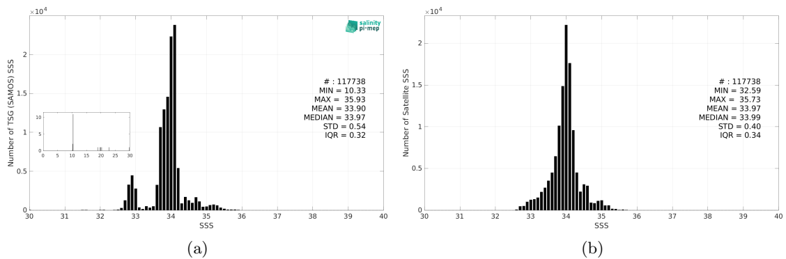
Figure 3: Histograms of SSS from TSG (SAMOS) (a) and CCI SSS L4 Merged-OI v5.5 - 30-day running (ESA) (b) considering all match-up pairs per bins of 0.1 over the Roaring Forties and Furious Fifties Pi-MEP region and for the full satellite product period.
