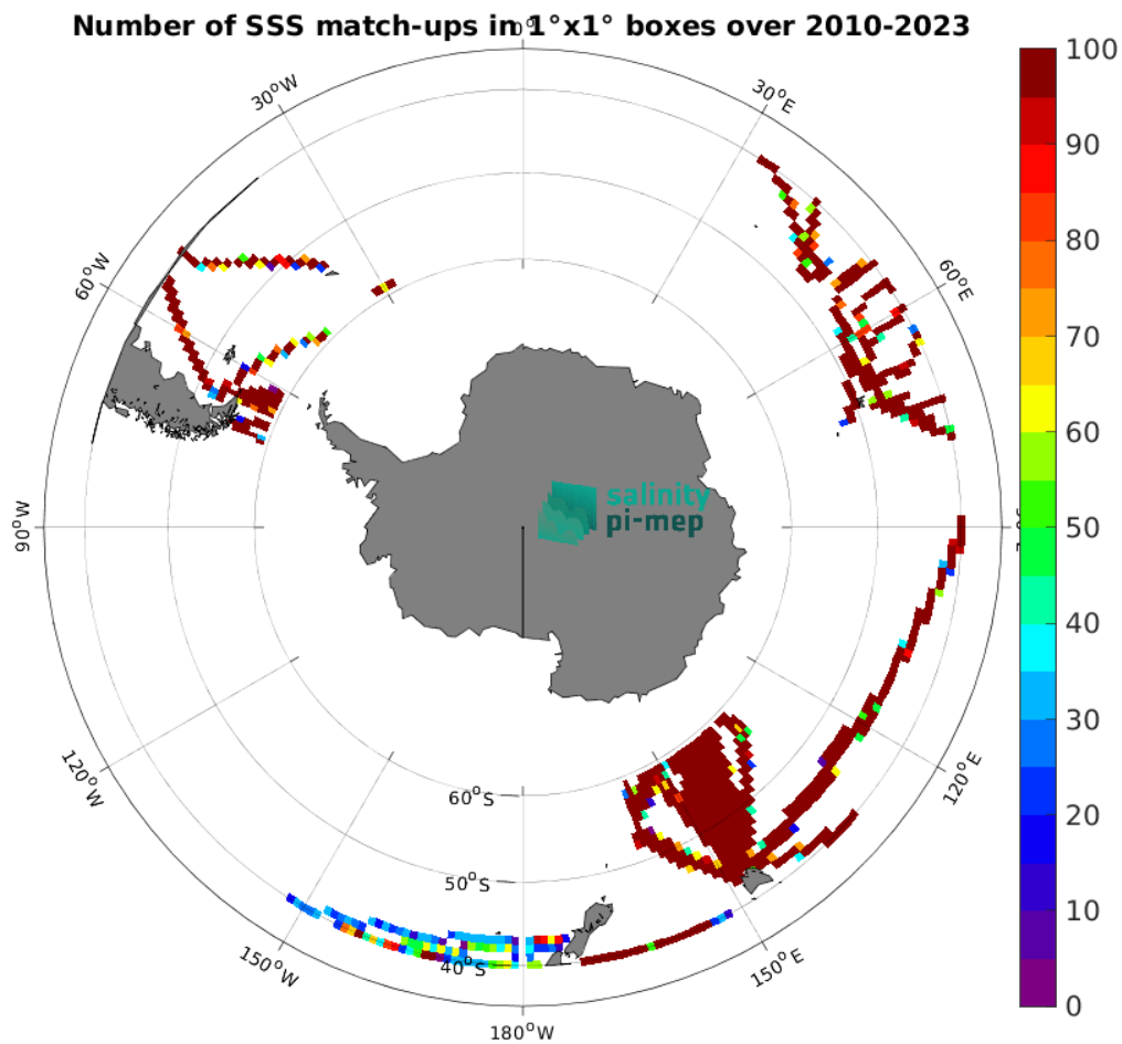
Figure 5: Number of SSS match-ups between TSG (LEGOS-DM) SSS and the CCI SSS L4 Merged-OI v5.5 - 30-day running (ESA) SSS product for the Roaring Forties and Furious Fifties Pi-MEP region over 1^\circ \times 1^\circ boxes and for the full satellite product period.
