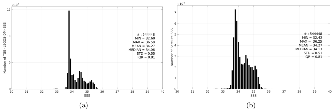
Figure 3: Histograms of SSS from TSG (LEGOS-DM) (a) and CCI SSS L4 Merged-OI v5.5 - 30-day running (ESA) (b) considering all match-up pairs per bins of 0.1 over the Roaring Forties and Furious Fifties Pi-MEP region and for the full satellite product period.
