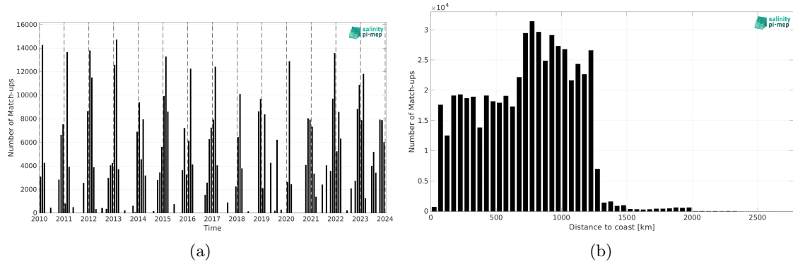
Figure 2: Number of match-ups between TSG (LEGOS-DM) and CCI SSS L4 Merged-OI v5.5 - 30-day running (ESA) SSS as a function of time (a) and as function of the distance to coast (b) over the Roaring Forties and Furious Fifties Pi-MEP region and for the full satellite product period.
