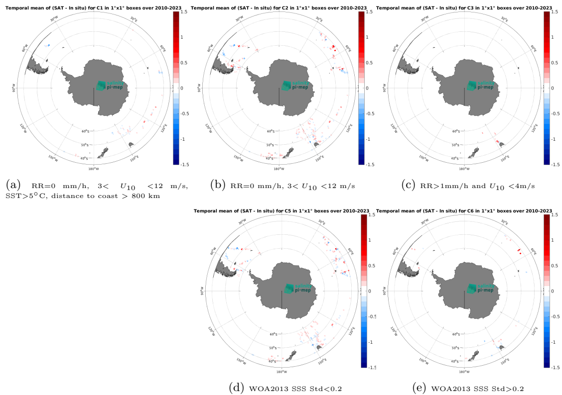
Figure 14: Temporal mean gridded over spatial boxes of size 1^\circ \times 1^\circ of \Delta SSS (CCI SSS L4 Merged-OI v5.5 - 30-day running (ESA) - TSG (LEGOS-DM)) for 5 different subdatasets corresponding to:RR=0 mm/h, 3 < U_{10} < 12 m/s, SST>5°C, distance to coast > 800 km (a), RR=0 mm/h, 3 < U_{10} < 12 m/s (b), RR>1mm/h and U_{10} < 4 m/s (c), WOA2013 SSS Std<0.2 (d), WOA2013 SSS Std>0.2 (e).
