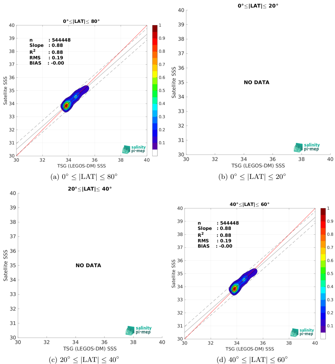
Figure 10: Contour maps of the concentration of CCI SSS L4 Merged-OI v5.5 - 30-day running (ESA) SSS (y-axis) versus TSG (LEGOS-DM) SSS (x-axis) at match-up pairs for different latitude bands. For each plot, the red line shows x=y . The black thin and dashed lines indicate a linear fit through the data cloud and the \pm 95\% confidence levels, respectively. The number match-up pairs n , the slope and R^2 coefficient of the linear fit, the root mean square (RMS) and the mean bias between satellite and in situ data are indicated for each latitude band in each plots.
