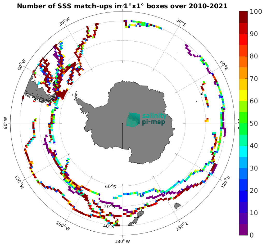
Figure 5: Number of SSS match-ups between TSG (GOSUD-Sailing-ship) SSS and the CCI SSS L4 Merged-OI v5.5 - 30-day running (ESA) SSS product for the Roaring Forties and Furious Fifties Pi-MEP region over 1^\circ \times 1^\circ boxes and for the full satellite product period.
