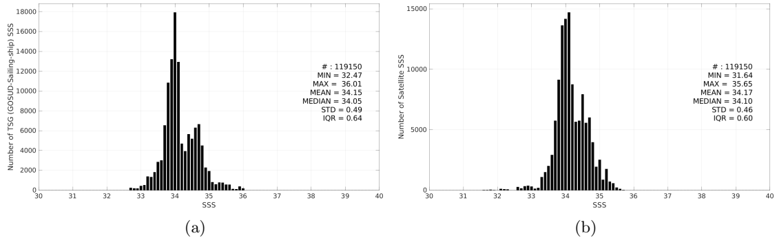
Figure 3: Histograms of SSS from TSG (GOSUD-Sailing-ship) (a) and CCI SSS L4 Merged-OI v5.5 - 30-day running (ESA) (b) considering all match-up pairs per bins of 0.1 over the Roaring Forties and Furious Fifties Pi-MEP region and for the full satellite product period.
