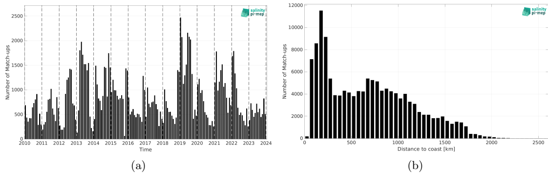
Figure 2: Number of match-ups between Marine mammals and CCI SSS L4 Merged-OI v5.5 - 30-day running (ESA) SSS as a function of time (a) and as function of the distance to coast (b) over the Roaring Forties and Furious Fifties Pi-MEP region and for the full satellite product period.
