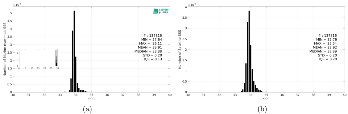
Figure 3: Histograms of SSS from Marine mammals (a) and CCI SSS L4 Merged-OI v5.5 - 30-day running (ESA) (b) considering all match-up pairs per bins of 0.1 over the Roaring Forties and Furious Fifties Pi-MEP region and for the full satellite product period.
