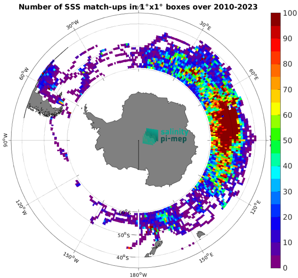
Figure 5: Number of SSS match-ups between Marine mammals SSS and the CCI SSS L4 Merged-OI v5.5 - 30-day running (ESA) SSS product for the Roaring Forties and Furious Fifties Pi-MEP region over 1^\circ \times 1^\circ boxes and for the full satellite product period.
