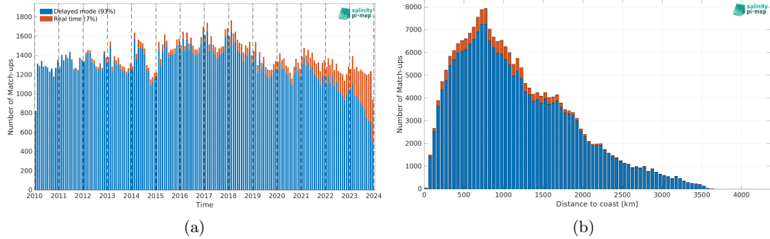
Figure 2: Number of match-ups between Argo and CCI SSS L4 Merged-OI v5.5 - 30-day running (ESA) SSS as a function of time (a) and as function of the distance to coast (b) over the Roaring Forties and Furious Fifties Pi-MEP region and for the full satellite product period.
