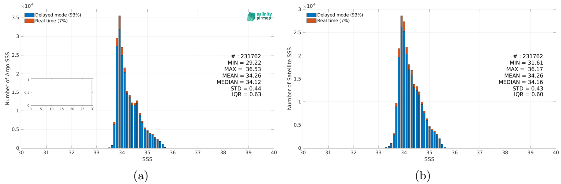
Figure 3: Histograms of SSS from Argo (a) and CCI SSS L4 Merged-OI v5.5 - 30-day running (ESA) (b) considering all match-up pairs per bins of 0.1 over the Roaring Forties and Furious Fifties Pi-MEP region and for the full satellite product period.
