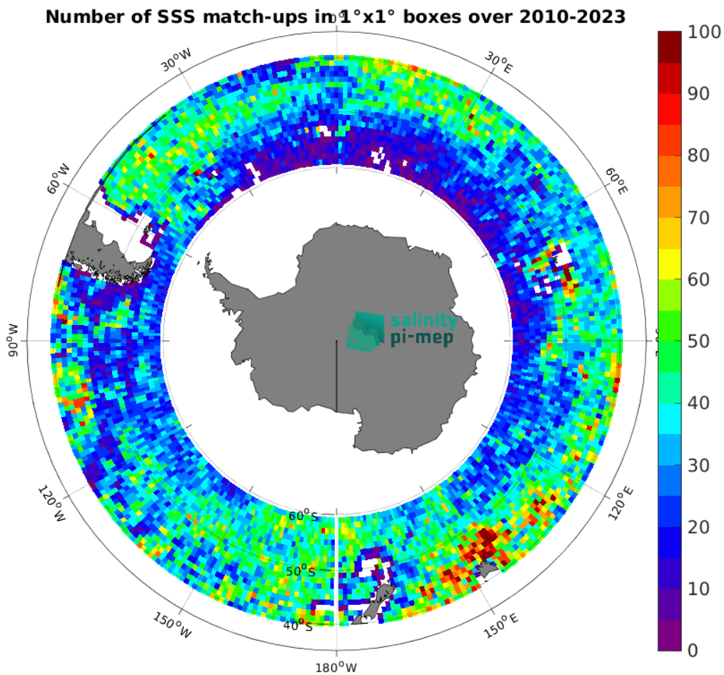
Figure 5: Number of SSS match-ups between Argo SSS and the CCI SSS L4 Merged-OI v5.5 - 30-day running (ESA) SSS product for the Roaring Forties and Furious Fifties Pi-MEP region over 1^{\circ} \times 1^{\circ} boxes and for the full satellite product period.
