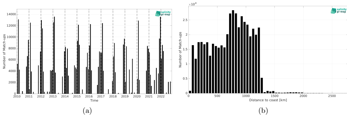
Figure 2: Number of match-ups between TSG (LEGOS-DM) and CCI SSS L4 Merged-OI v4.41 - 7-day running (ESA) SSS as a function of time (a) and as function of the distance to coast (b) over the Roaring Forties and Furious Fifties Pi-MEP region and for the full satellite product period.
