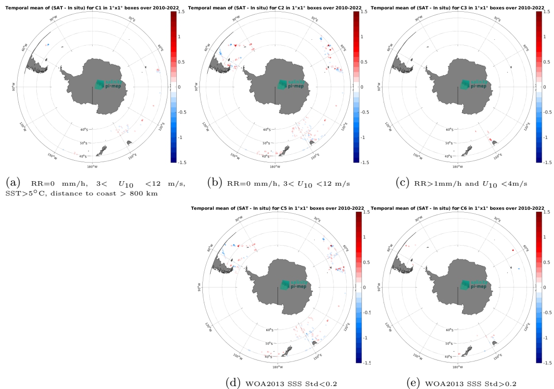
Figure 14: Temporal mean gridded over spatial boxes of size 1^\circ \times 1^\circ of \Delta\text{SSS} (CCI SSS L4 Merged-OI v4.41 - 7-day running (ESA) - TSG (LEGOS-DM)) for 5 different subdatasets corresponding to:RR=0 mm/h, 3 < U_{10} < 12 m/s, SST>5°C, distance to coast > 800 km (a), RR=0 mm/h, 3 < U_{10} < 12 m/s (b), RR>1mm/h and U_{10} < 4 m/s (c), WOA2013 SSS Std<0.2 (d), WOA2013 SSS Std>0.2 (e).
