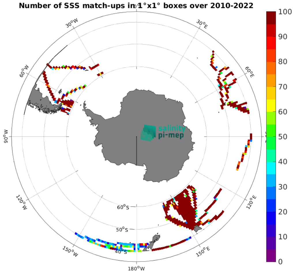
Figure 5: Number of SSS match-ups between TSG (LEGOS-DM) SSS and the CCI SSS L4 Merged-OI v4.41 - 7-day running (ESA) SSS product for the Roaring Forties and Furious Fifties Pi-MEP region over 1^\circ \times 1^\circ boxes and for the full satellite product period.
