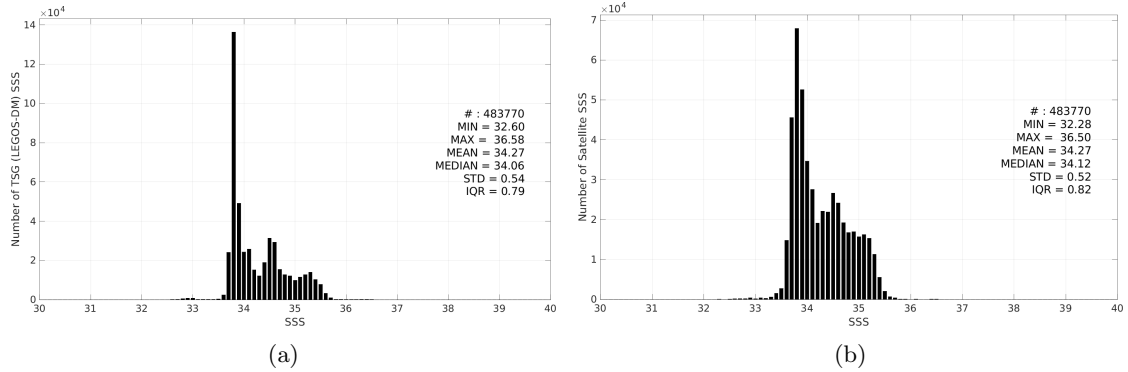
Figure 3: Histograms of SSS from TSG (LEGOS-DM) (a) and CCI SSS L4 Merged-OI v4.41 - 7-day running (ESA) (b) considering all match-up pairs per bins of 0.1 over the Roaring Forties and Furious Fifties Pi-MEP region and for the full satellite product period.
